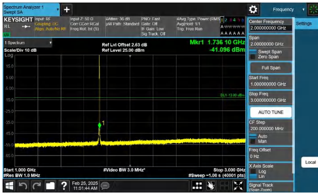
Band4-1.4MHz-QPSK-20175-1RB#5-1000~3000-PASS
