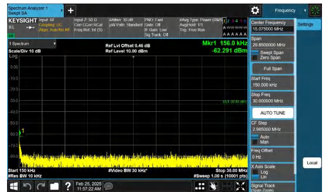
Band4-3MHz-QPSK-20385-1RB#0-0.15~30-PASS
