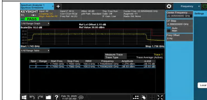
Band4-10MHz-QPSK-20350-50RB#0-PASS
