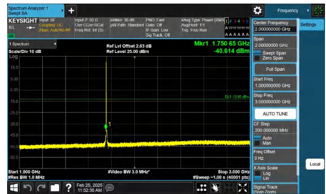
Band4-1.4MHz-QPSK-20393-1RB#0-1000~3000-PASS
