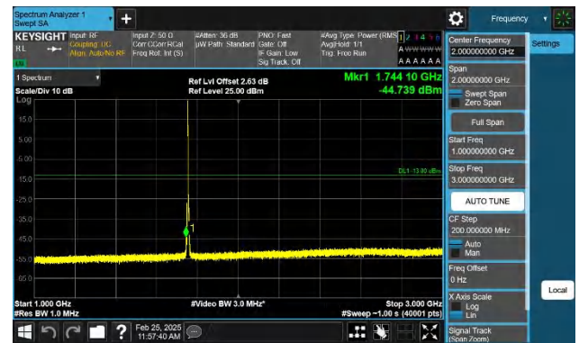
Band4-3MHz-QPSK-20385-1RB#0-1000~3000-PASS
