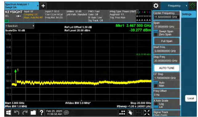
Band4-3MHz-QPSK-20175-1RB#14-3000~20000-PASS
