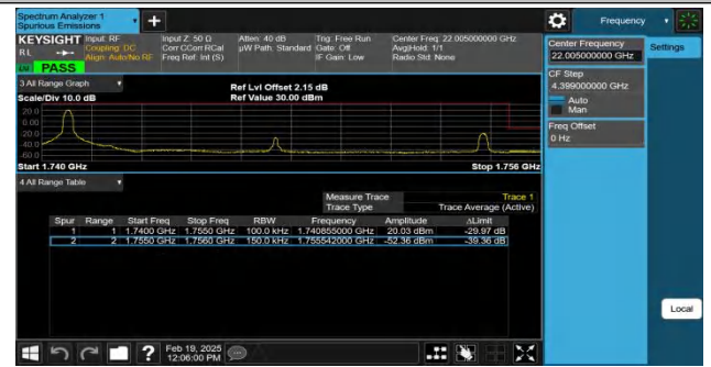
Band4-15MHz-QPSK-20325-1RB#0-PASS
