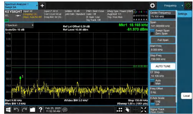
Band4-1.4MHz-QPSK-20393-1RB#5-0.009~0.15-PASS
