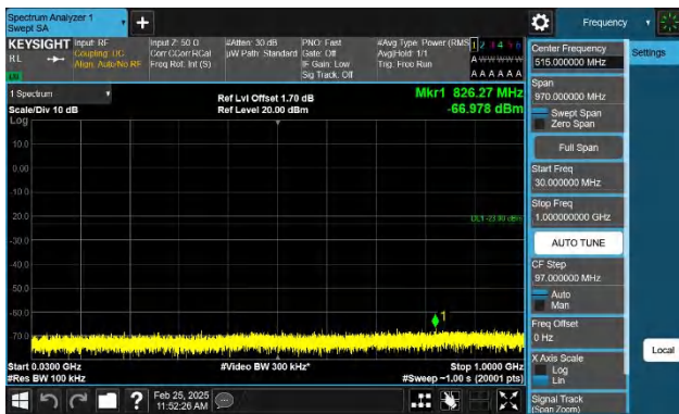
Band4-1.4MHz-QPSK-20393-1RB#0-30~1000-PASS
