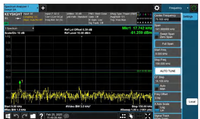
Band4-1.4MHz-QPSK-19957-1RB#5-0.009~0.15-PASS
