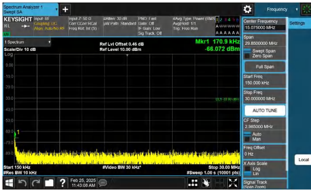
Band2-20MHz-QPSK-18700-1RB#99-0.15~30-PASS
