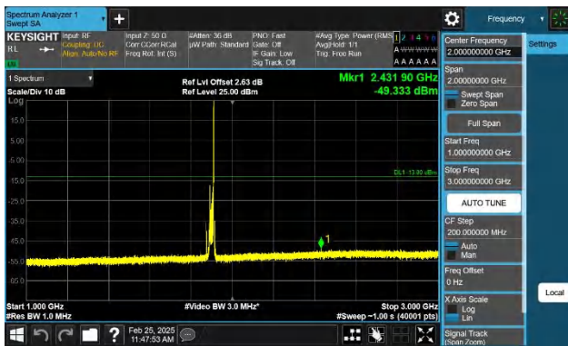
Band2-20MHz-QPSK-19100-1RB#99-1000~3000-PASS
