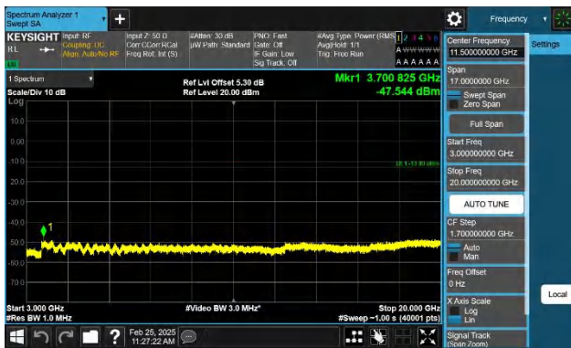
Band2-5MHz-QPSK-18625-1RB#0-3000~20000-PASS
