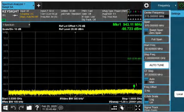
Band2-10MHz-QPSK-18900-1RB#0-30~1000-PASS
