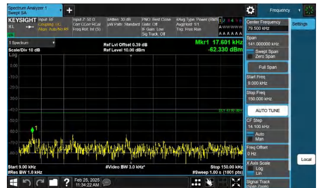
Band2-10MHz-QPSK-18900-1RB#49-0.009~0.15-PASS
