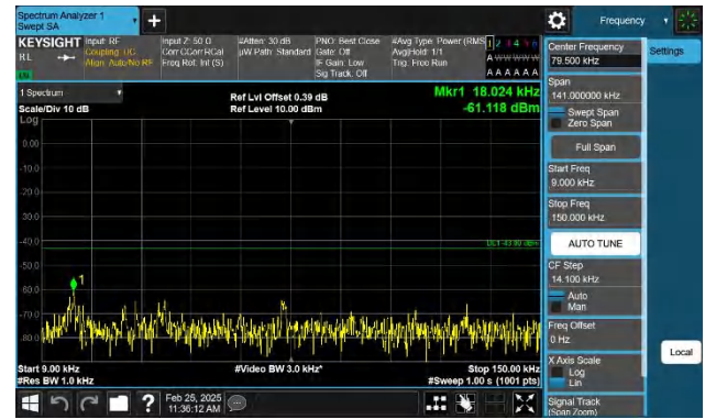
Band2-10MHz-QPSK-19150-1RB#49-0.009~0.15-PASS
