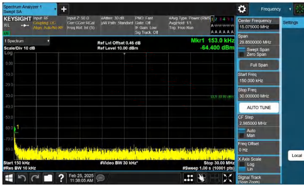
Band2-15MHz-QPSK-18675-1RB#74-0.15~30-PASS
