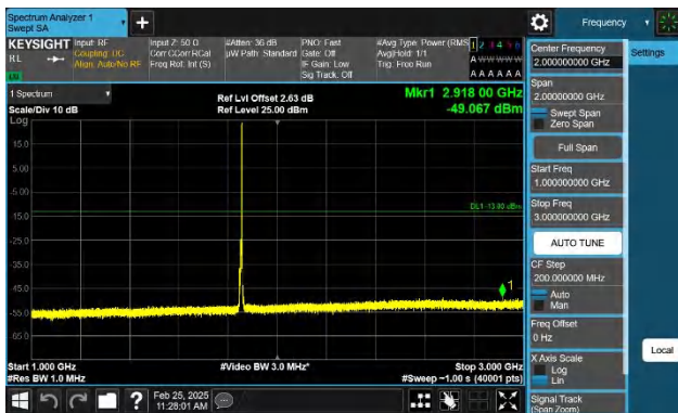
Band2-5MHz-QPSK-18625-1RB#24-1000~3000-PASS
