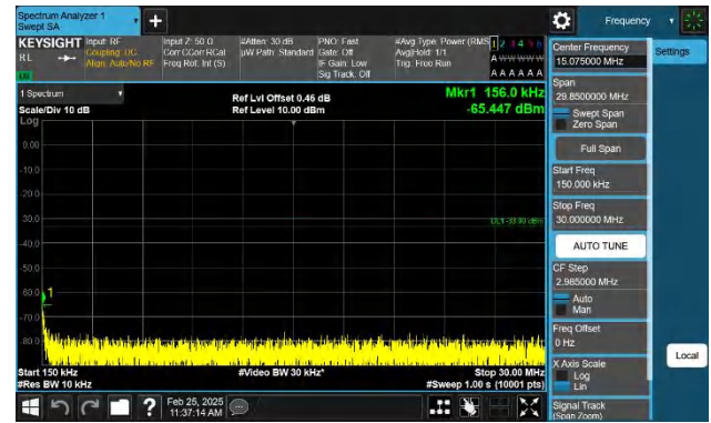
Band2-15MHz-QPSK-18675-1RB#0-0.15~30-PASS
