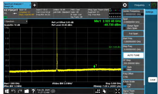
Band2-5MHz-QPSK-18625-1RB#0-1000~3000-PASS
