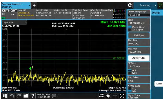
Band2-10MHz-QPSK-18900-1RB#0-0.009~0.15-PASS
