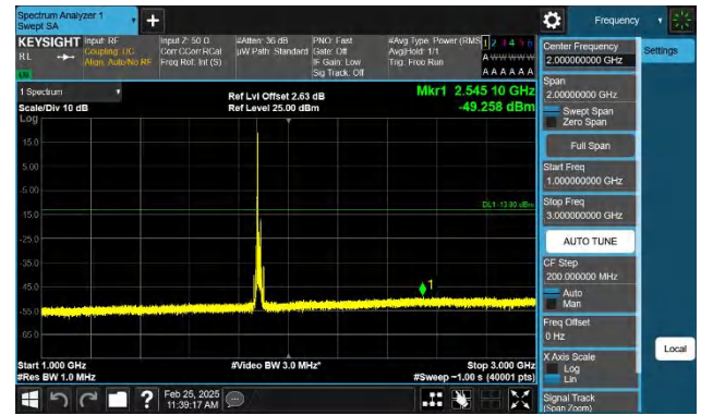
Band2-15MHz-QPSK-18900-1RB#0-1000~3000-PASS
