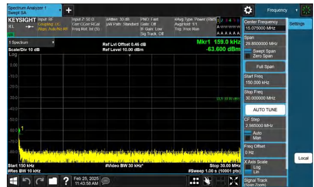
Band2-20MHz-QPSK-18900-1RB#0-0.15~30-PASS
