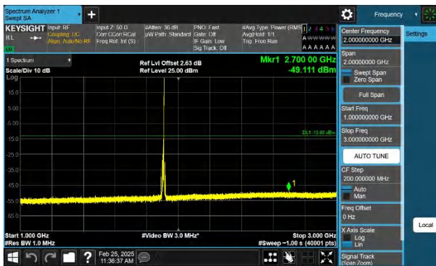
Band2-10MHz-QPSK-19150-1RB#49-1000~3000-PASS
