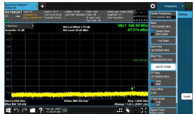
Band2-15MHz-QPSK-18900-1RB#74-30~1000-PASS
