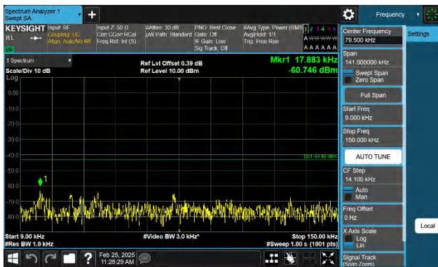
Band2-5MHz-QPSK-18900-1RB#0-0.009~0.15-PASS
