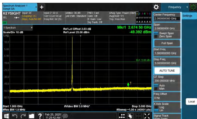
Band2-5MHz-QPSK-18900-1RB#24-1000~3000-PASS
