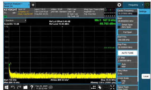
Band2-10MHz-QPSK-19150-1RB#0-0.15~30-PASS
