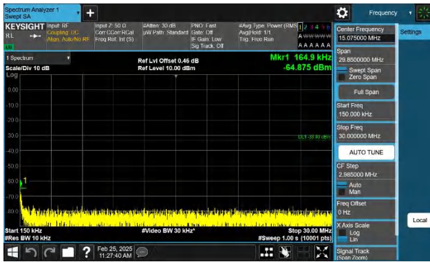
Band2-5MHz-QPSK-18625-1RB#24-0.15~30-PASS
