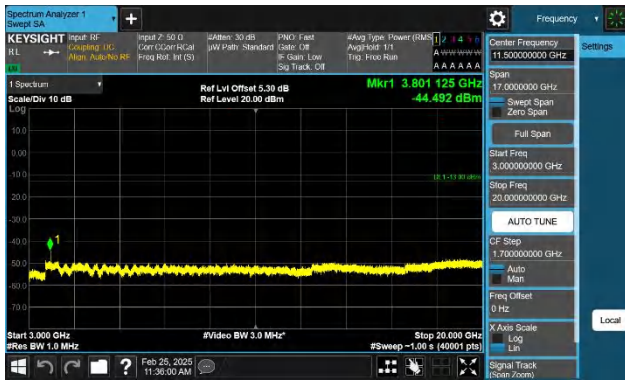
Band2-10MHz-QPSK-19150-1RB#0-3000~20000-PASS
