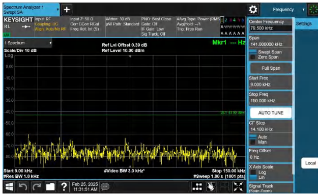
Band2-10MHz-QPSK-18650-1RB#0-0.009~0.15-PASS
