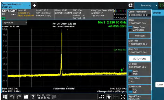
Band2-15MHz-QPSK-19125-1RB#74-1000~3000-PASS
