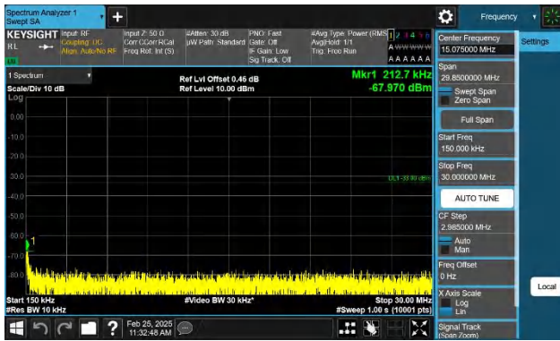
Band2-10MHz-QPSK-18650-1RB#49-0.15~30-PASS
