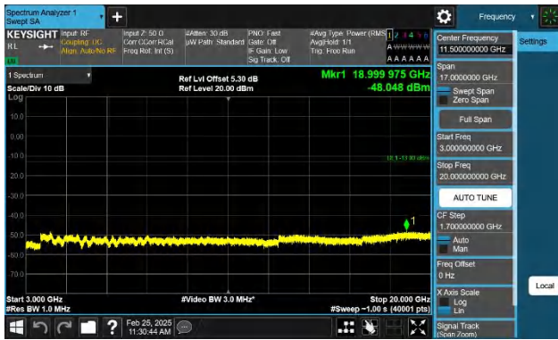
Band2-5MHz-QPSK-19175-1RB#0-3000~20000-PASS
