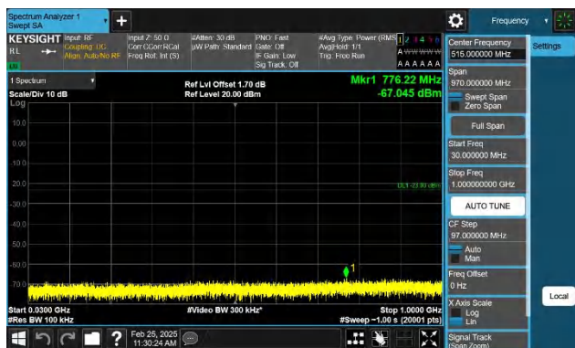
Band2-5MHz-QPSK-19175-1RB#0-30~1000-PASS
