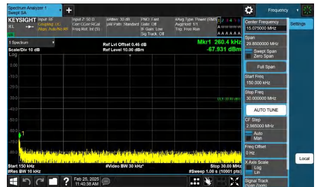
Band2-15MHz-QPSK-19125-1RB#0-0.15~30-PASS
