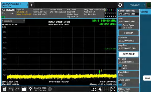
Band2-5MHz-QPSK-18625-1RB#0-30~1000-PASS
