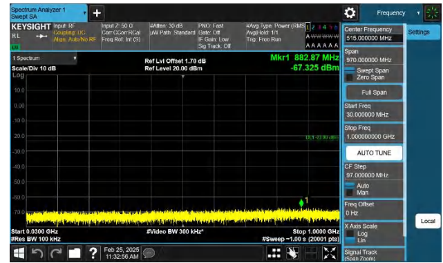
Band2-10MHz-QPSK-18650-1RB#49-30~1000-PASS
