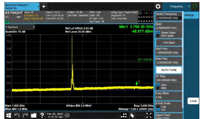
Band2-15MHz-QPSK-18675-1RB#0-1000~3000-PASS
