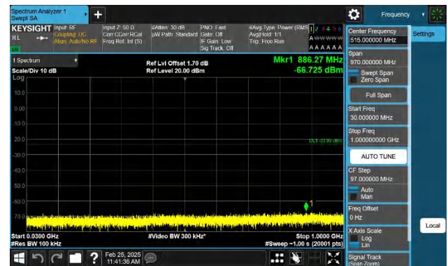
Band2-15MHz-QPSK-19125-1RB#74-30~1000-PASS
