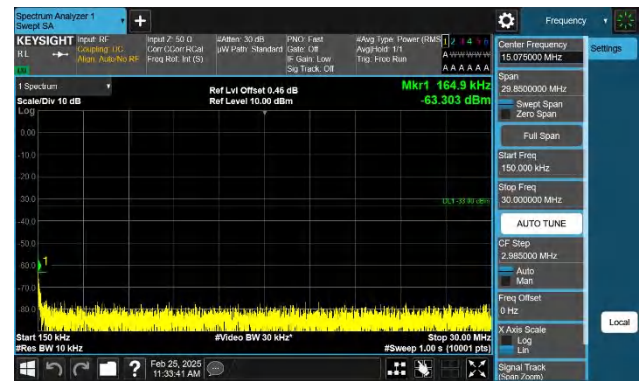
Band2-10MHz-QPSK-18900-1RB#0-0.15~30-PASS
