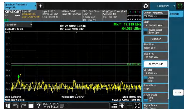
Band2-5MHz-QPSK-18900-1RB#24-0.009~0.15-PASS
