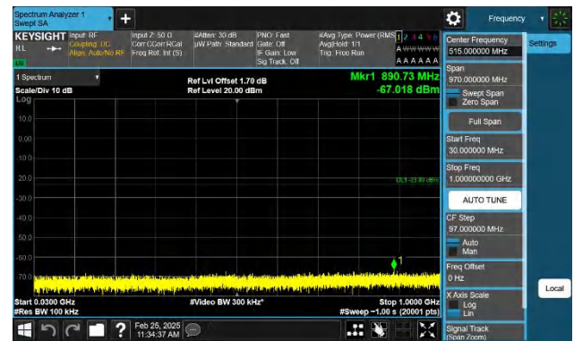
Band2-10MHz-QPSK-18900-1RB#49-30~1000-PASS
