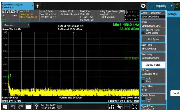
Band2-15MHz-QPSK-19125-1RB#74-0.15~30-PASS
