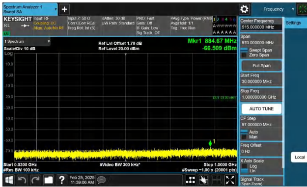
Band2-15MHz-QPSK-18900-1RB#0-30~1000-PASS
