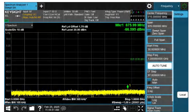
Band2-20MHz-QPSK-18900-1RB#99-30~1000-PASS
