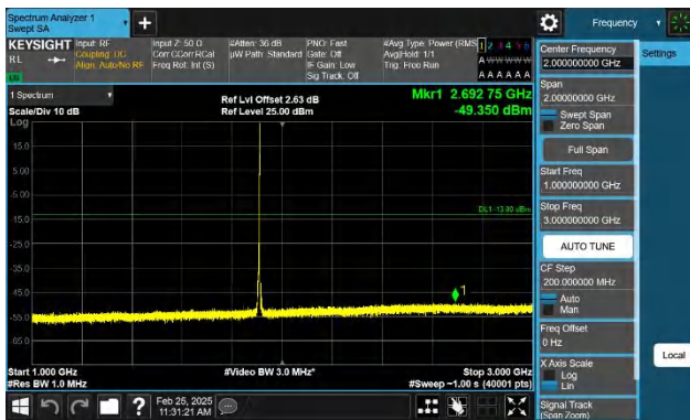
Band2-5MHz-QPSK-19175-1RB#24-1000~3000-PASS
