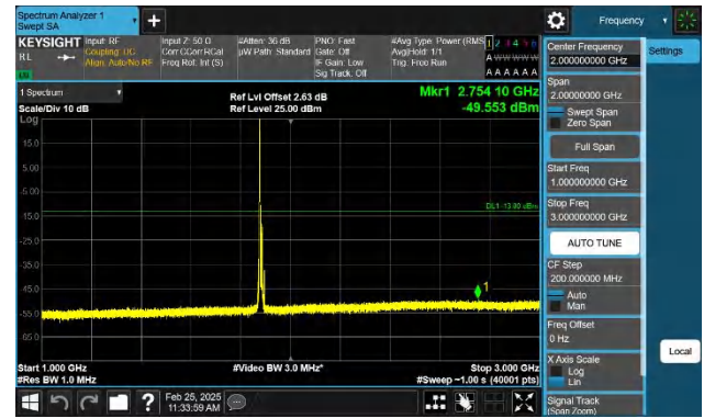
Band2-10MHz-QPSK-18900-1RB#0-1000~3000-PASS
