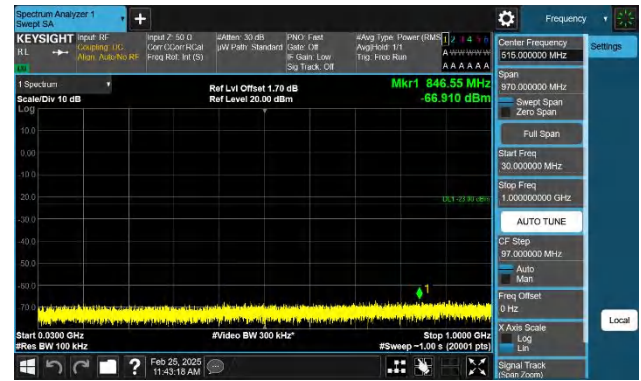
Band2-20MHz-QPSK-18700-1RB#99-30~1000-PASS
