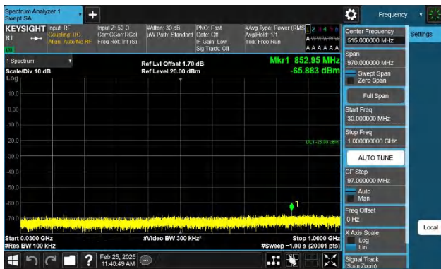
Band2-15MHz-QPSK-19125-1RB#0-30~1000-PASS
