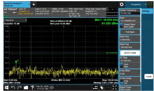
Band2-15MHz-QPSK-19125-1RB#74-0.009~0.15-PASS
