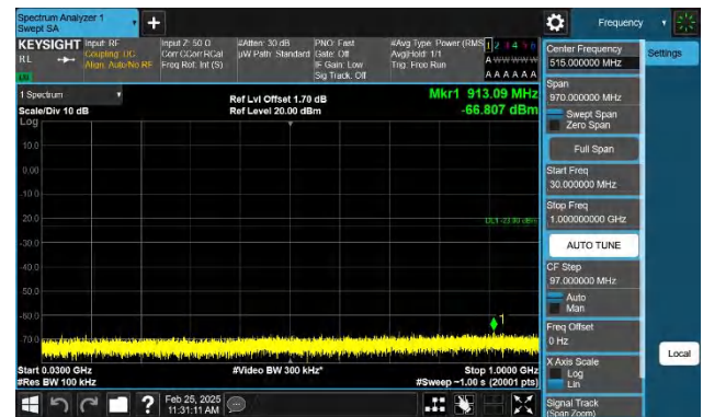
Band2-5MHz-QPSK-19175-1RB#24-30~1000-PASS
