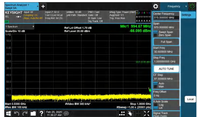
Band2-10MHz-QPSK-19150-1RB#49-30~1000-PASS
