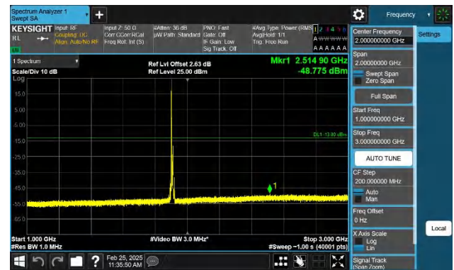
Band2-10MHz-QPSK-19150-1RB#0-1000~3000-PASS
