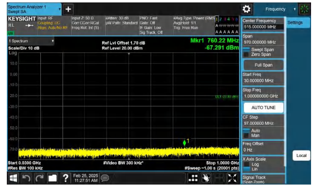
Band2-5MHz-QPSK-18625-1RB#24-30~1000-PASS
