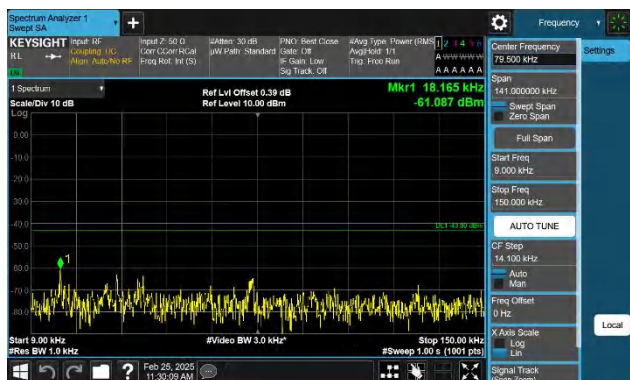
Band2-5MHz-QPSK-19175-1RB#0-0.009~0.15-PASS
