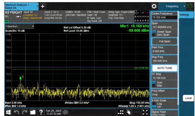
Band2-5MHz-QPSK-18625-1RB#24-0.009~0.15-PASS
