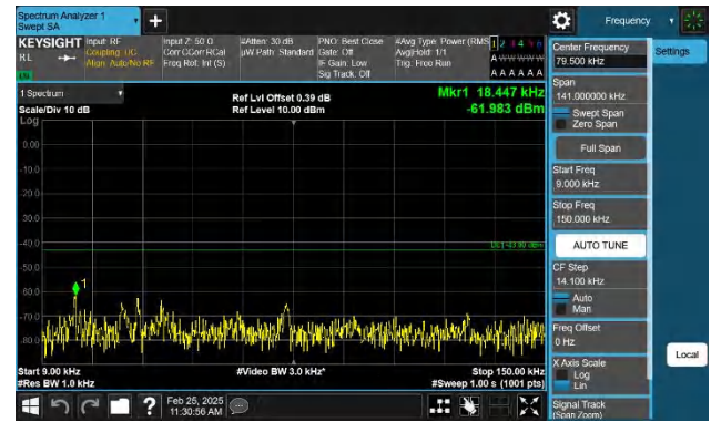
Band2-5MHz-QPSK-19175-1RB#24-0.009~0.15-PASS
