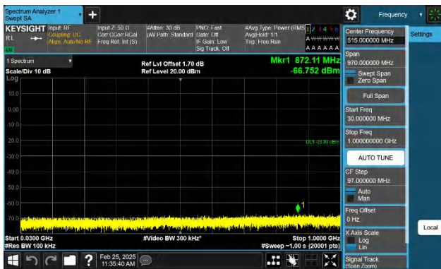
Band2-10MHz-QPSK-19150-1RB#0-30~1000-PASS
