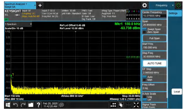
Band2-20MHz-QPSK-18700-1RB#0-0.15~30-PASS
