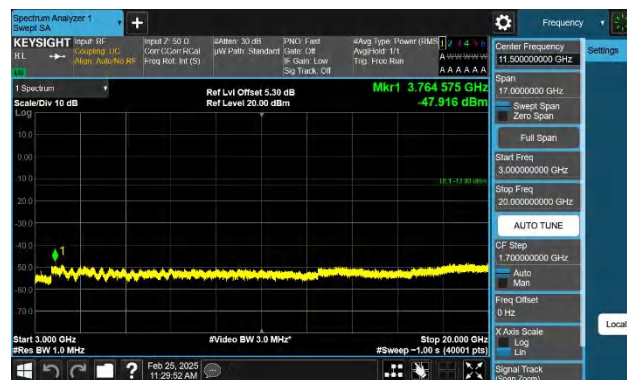
Band2-5MHz-QPSK-18900-1RB#24-3000~20000-PASS
