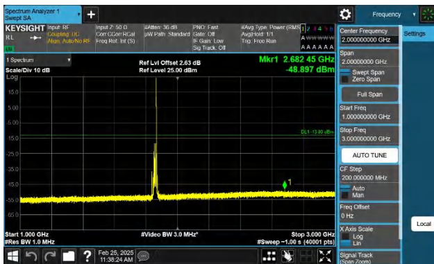
Band2-15MHz-QPSK-18675-1RB#74-1000~3000-PASS
