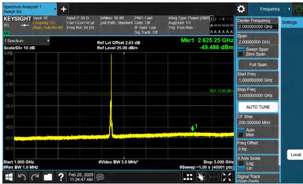
Band2-10MHz-QPSK-18900-1RB#49-1000~3000-PASS
