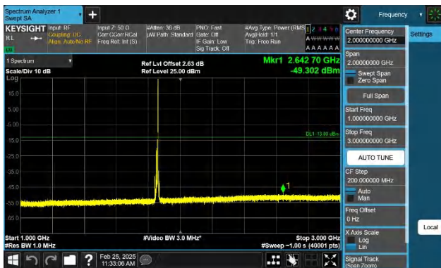
Band2-10MHz-QPSK-18650-1RB#49-1000~3000-PASS
