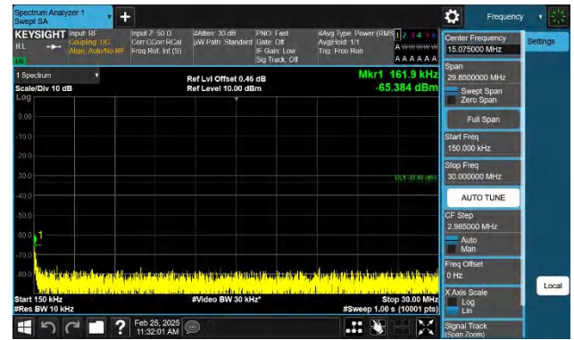
Band2-10MHz-QPSK-18650-1RB#0-0.15~30-PASS
