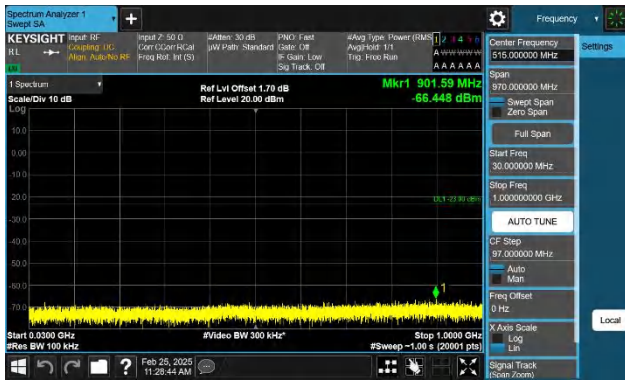
Band2-5MHz-QPSK-18900-1RB#0-30~1000-PASS
