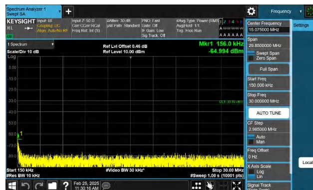
Band2-5MHz-QPSK-19175-1RB#0-0.15~30-PASS
