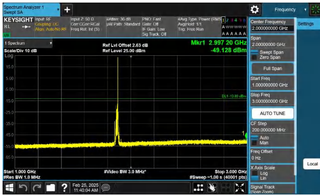
Band2-15MHz-QPSK-18900-1RB#74-1000~3000-PASS
