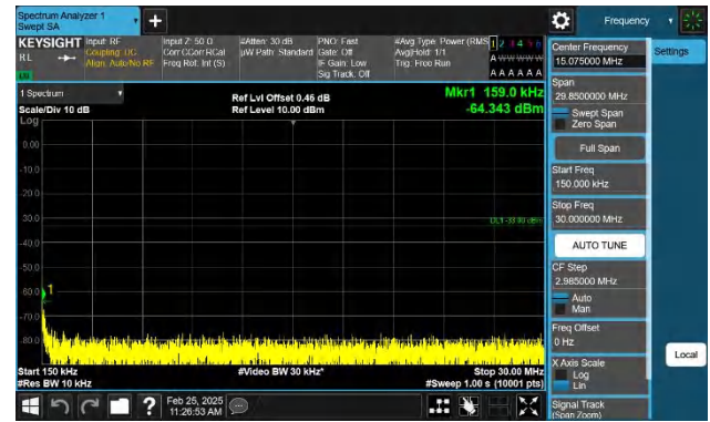
Band2-5MHz-QPSK-18625-1RB#0-0.15~30-PASS
