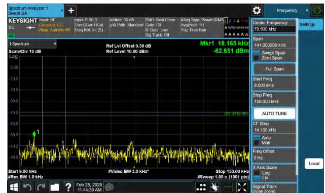
Band2-20MHz-QPSK-18900-1RB#99-0.009~0.15-PASS
