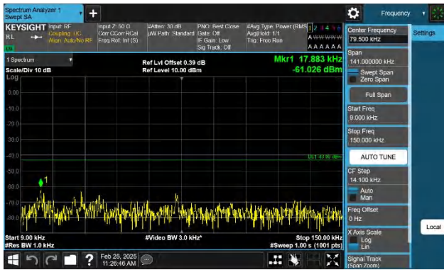
Band2-5MHz-QPSK-18625-1RB#0-0.009~0.15-PASS
