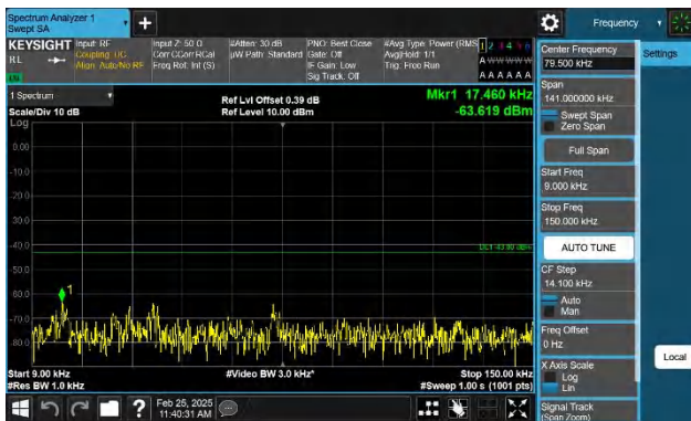
Band2-15MHz-QPSK-19125-1RB#0-0.009~0.15-PASS
