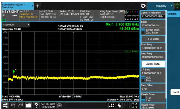
Band2-10MHz-QPSK-18650-1RB#0-3000~20000-PASS
