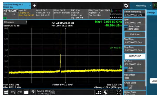
Band2-5MHz-QPSK-19175-1RB#0-1000~3000-PASS
