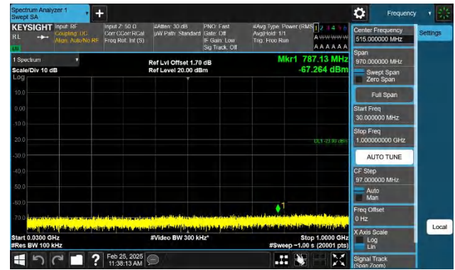
Band2-15MHz-QPSK-18675-1RB#74-30~1000-PASS
