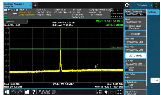
Band2-15MHz-QPSK-19125-1RB#0-1000~3000-PASS
