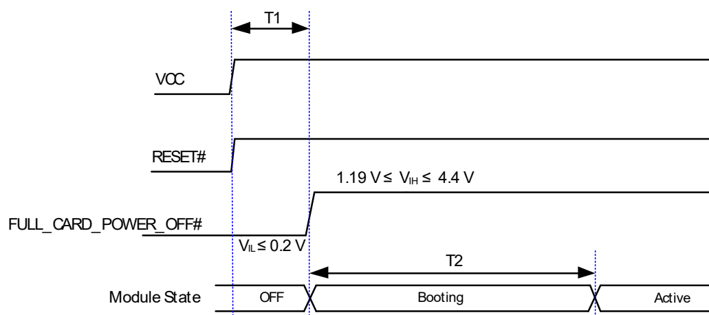
Figure 9: Turn-On Timing
