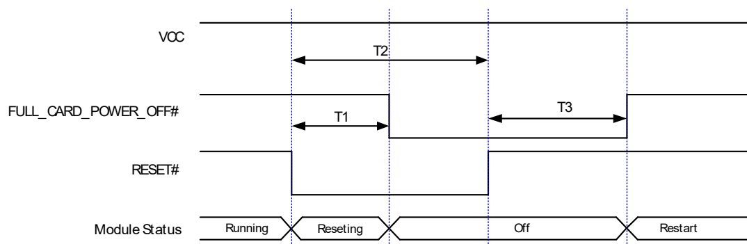
Figure 12: Reset Timing
