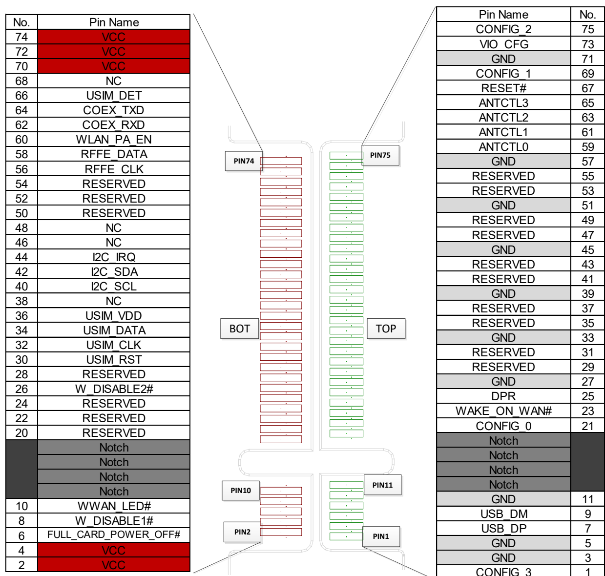
Figure 2: Pin Assignment
