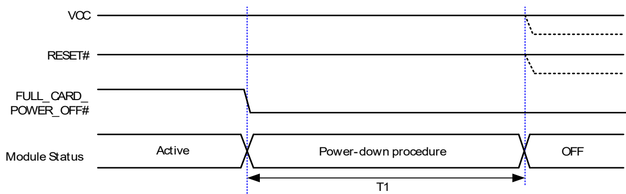
Figure 10: Turn-Off Timing
