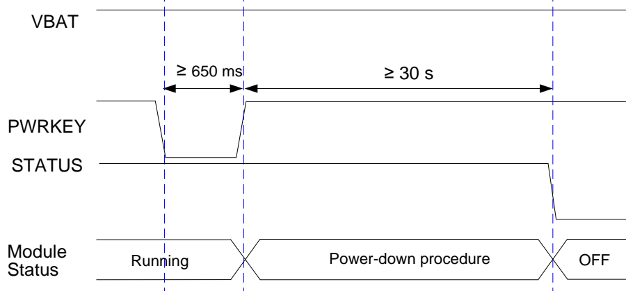
Figure 13: Turn-off Timing
