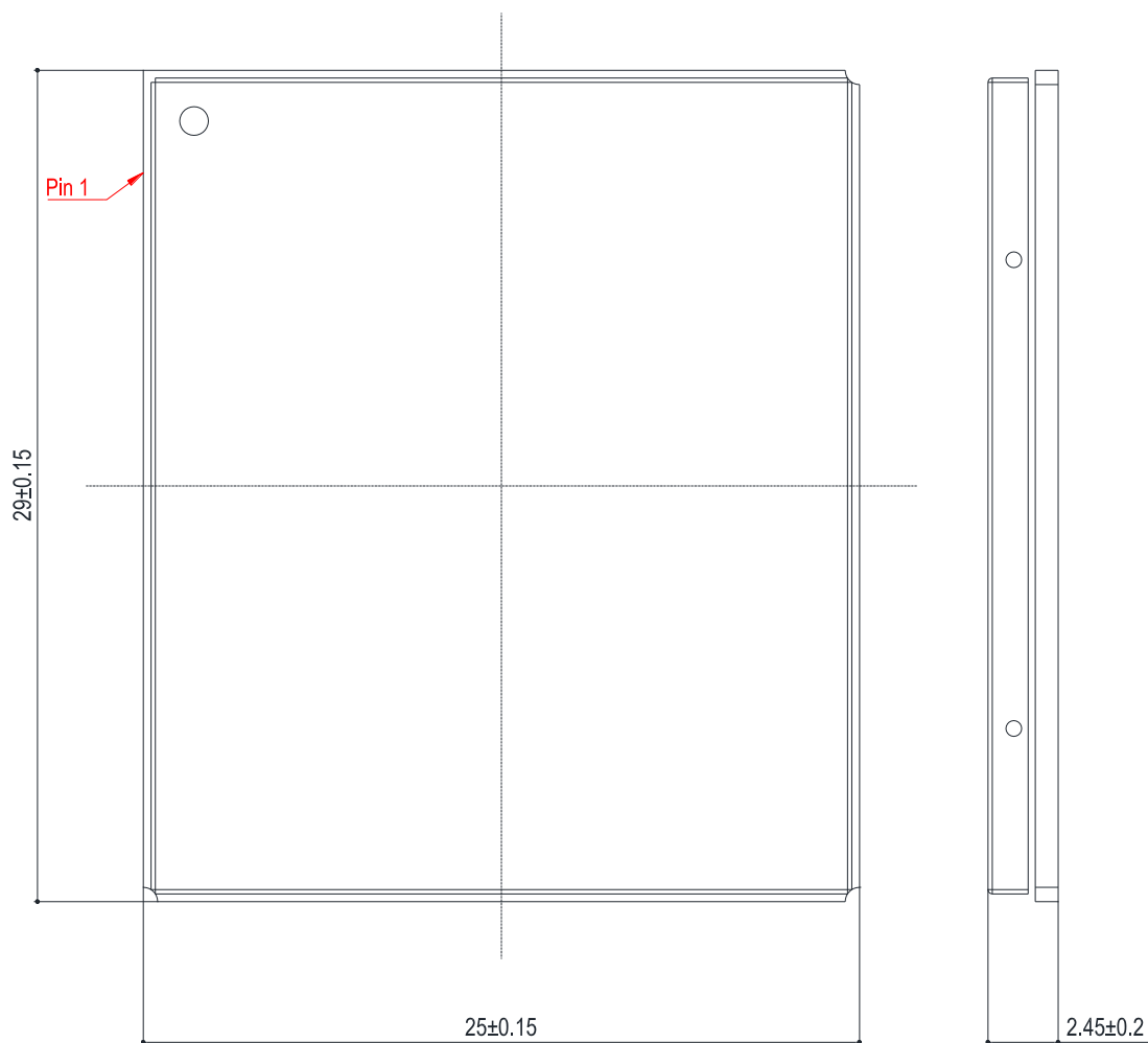
Figure 41: Top and Side Dimensions
