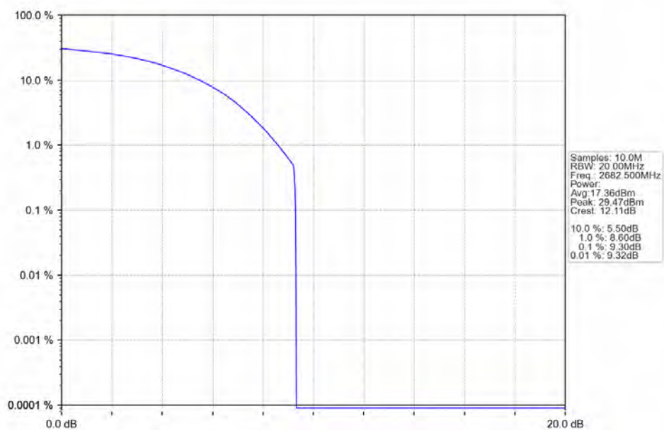
Band41_15MHz_256QAM_HCH_2682.5MHz_RB_75_0_NTNV
