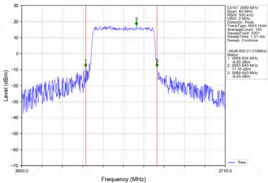
Band41_20MHz_256QAM_HCH_2680MHz_RB_100_0_NTNV
