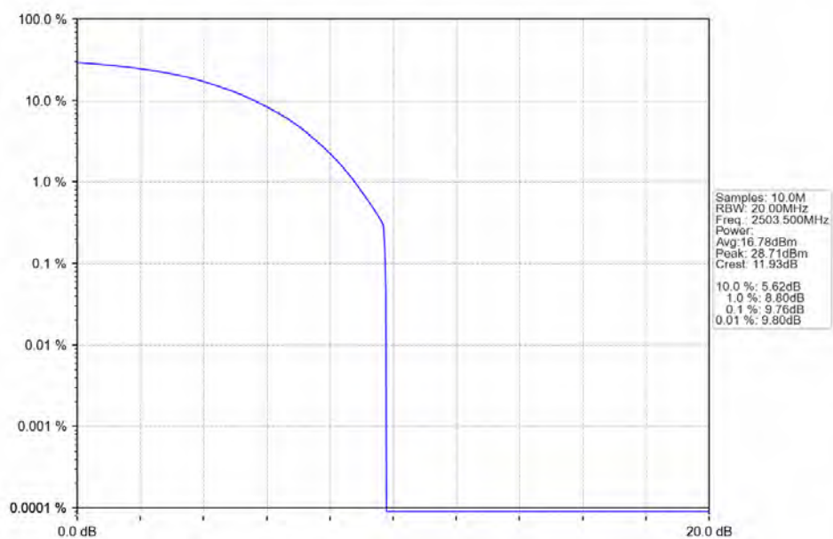
Band41_15MHz_256QAM_LCH_2503.5MHz_RB_75_0_NTNV
