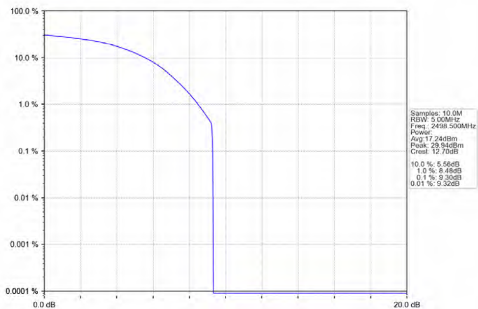
Band41_5MHz_256QAM_LCH_2498.5MHz_RB_25_0_NTNV
