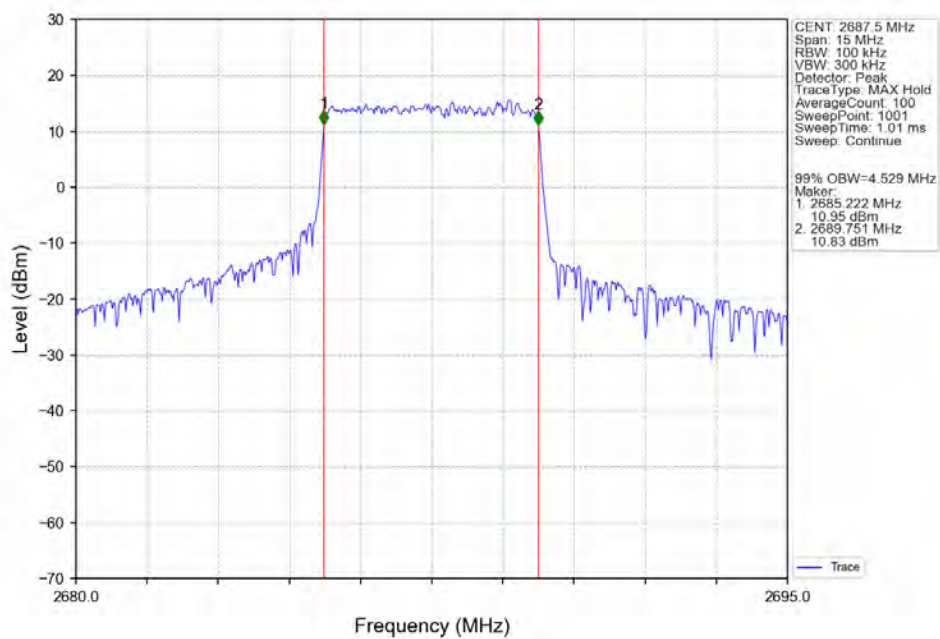
Band41_5MHz_256QAM_HCH_2687.5MHz_RB_25_0_NTNV
