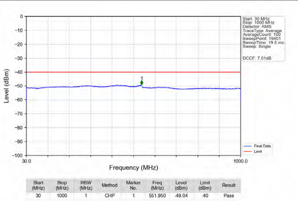
n48_30kHz_MIMO_NTNV_20MHz_CP-OFDM_QPSK_3690MHz_Edge_1RB_Right_Ant1
