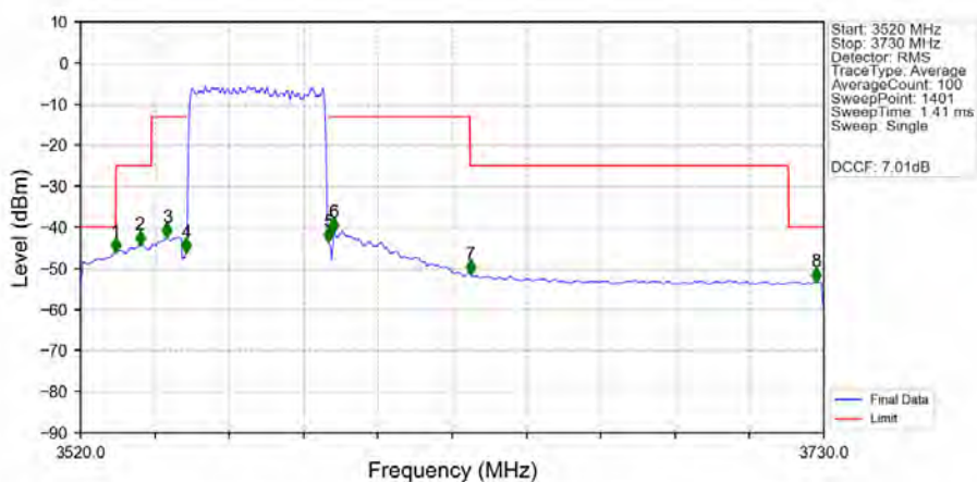
n48_30kHz_MIMO_NTNV_40MHz_CP-OFDM_QPSK_3570MHz_Outer_Full_Ant2
