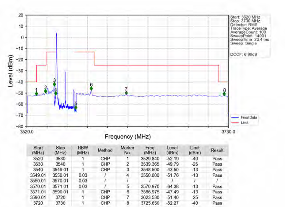
n48_30kHz_MIMO_NTNV_20MHz_CP-OFDM_QPSK_3560.01MHz_Edge_1RB_Left_Ant1
