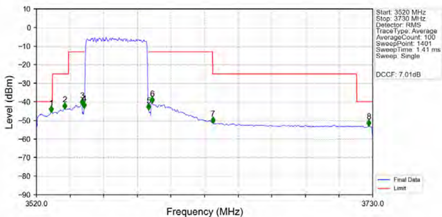
n48_30kHz_MIMO_NTNV_40MHz_CP-OFDM_QPSK_3570MHz_Outer_Full_Ant1
