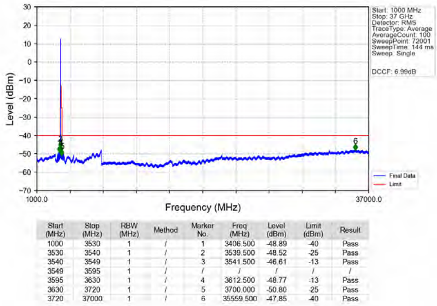
n48_30kHz_MIMO_NTNV_40MHz_CP-OFDM_QPSK_3570MHz_Edge_1RB_Left_Ant2
