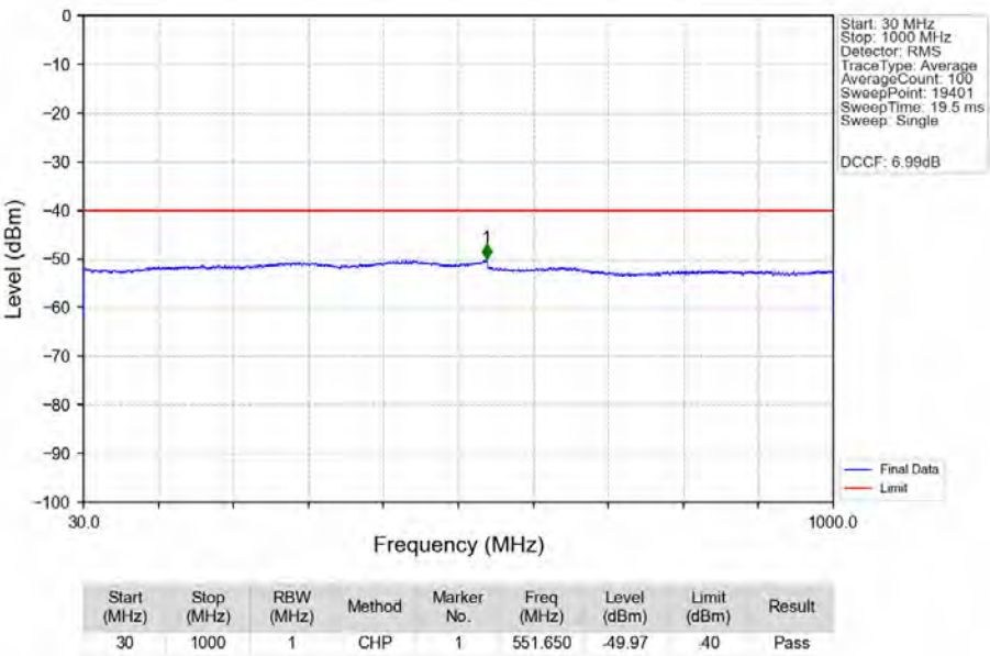
n48_30kHz_MIMO_NTNV_40MHz_CP-OFDM_QPSK_3570MHz_Edge_1RB_Left_Ant1
