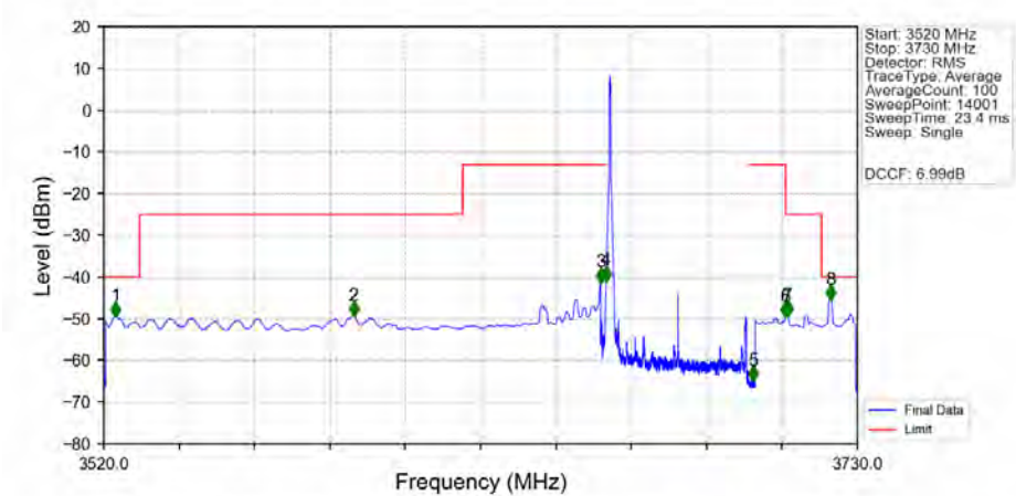
n48_30kHz_MIMO_NTNV_40MHz_DFT-s-OFDM_PI/2_BPSK_3679.98MHz_Edge_1RB_Left_Ant2
