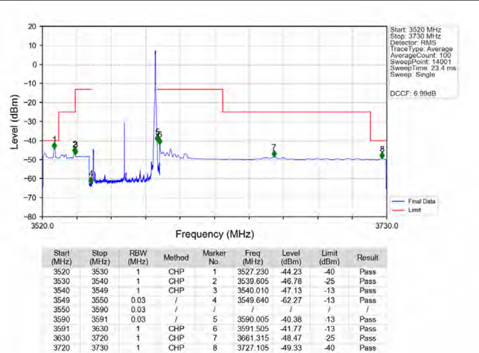
n48_30kHz_MIMO_NTNV_40MHz_CP-OFDM_QPSK_3570MHz_Edge_1RB_Right_MIMO
