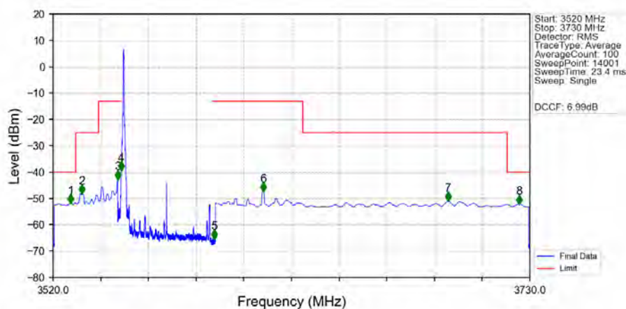
n48_30kHz_MIMO_NTNV_40MHz_DFT-s-OFDM_QPSK_3570MHz_Edge_1RB_Left_Ant2
