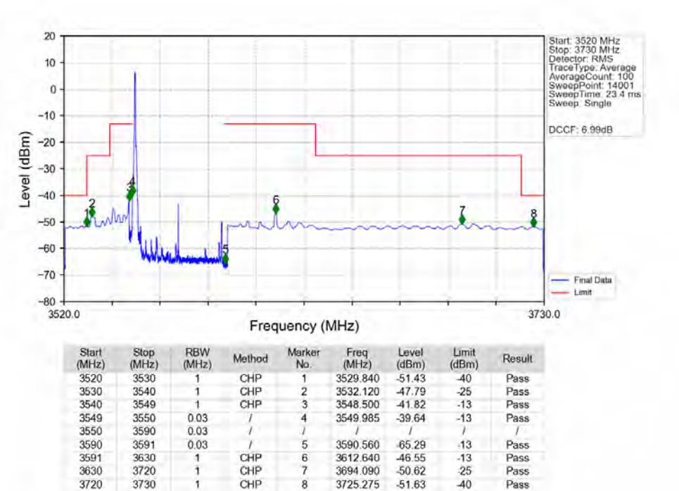
n48_30kHz_MIMO_NTNV_40MHz_DFT-s-OFDM_QPSK_3570MHz_Edge_1RB_Left_Ant1
