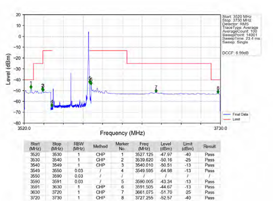
n48_30kHz_MIMO_NTNV_40MHz_CP-OFDM_QPSK_3570MHz_Edge_1RB_Right_Ant2
