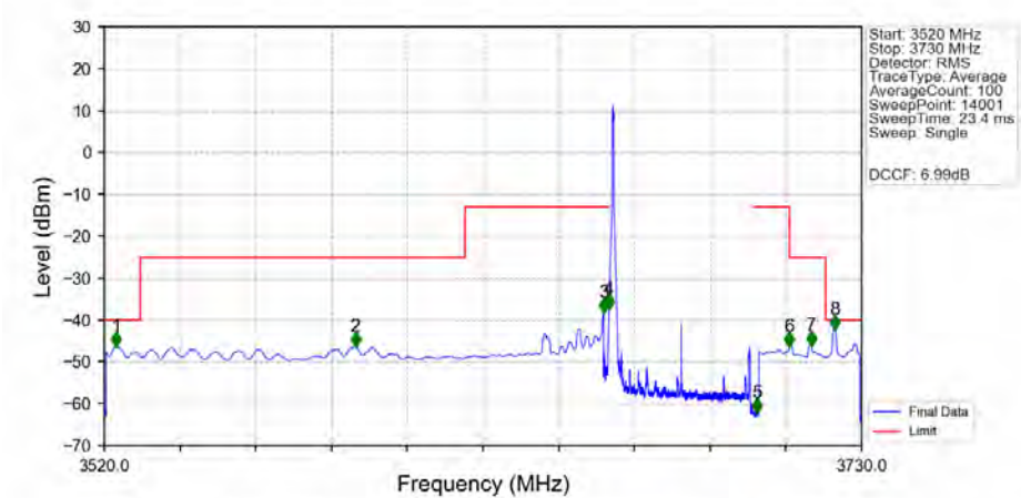
n48_30kHz_MIMO_NTNV_40MHz_DFT-s-OFDM_PI/2_BPSK_3679.98MHz_Edge_1RB_Left_MIMO
