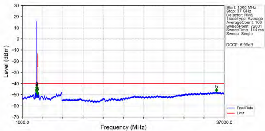
n48_30kHz_MIMO_NTNV_40MHz_DFT-s-OFDM_QPSK_3570MHz_Edge_1RB_Left_Ant1
