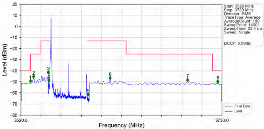
n48_30kHz_MIMO_NTNV_40MHz_DFT-s-OFDM_QPSK_3570MHz_Inner_1RB_Left_Ant1
