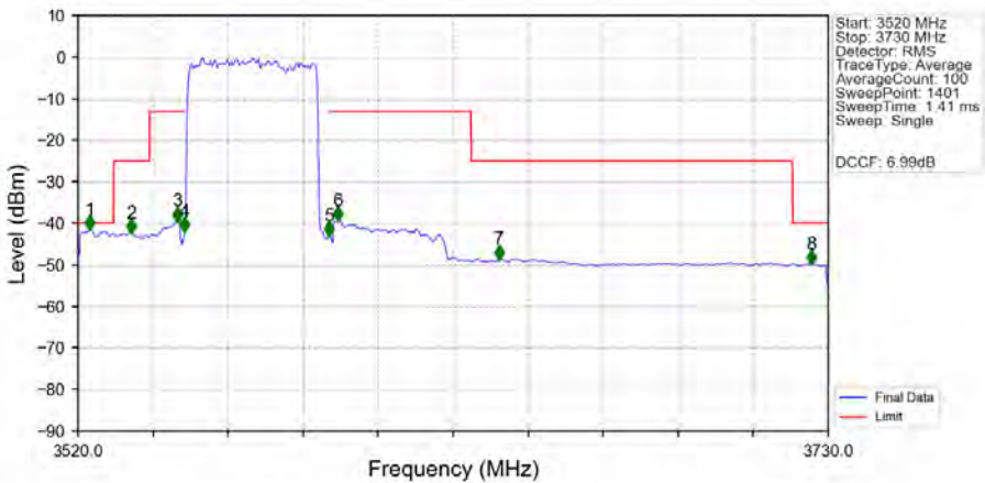
n48_30kHz_MIMO_NTNV_40MHz_DFT-s-OFDM_QPSK_3570MHz_Outer_Full_MIMO
