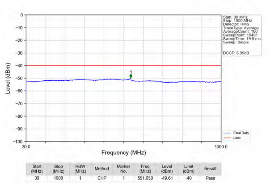
n48_30kHz_MIMO_NTNV_40MHz_DFT-s-OFDM_QPSK_3570MHz_Edge_1RB_Left_Ant1
