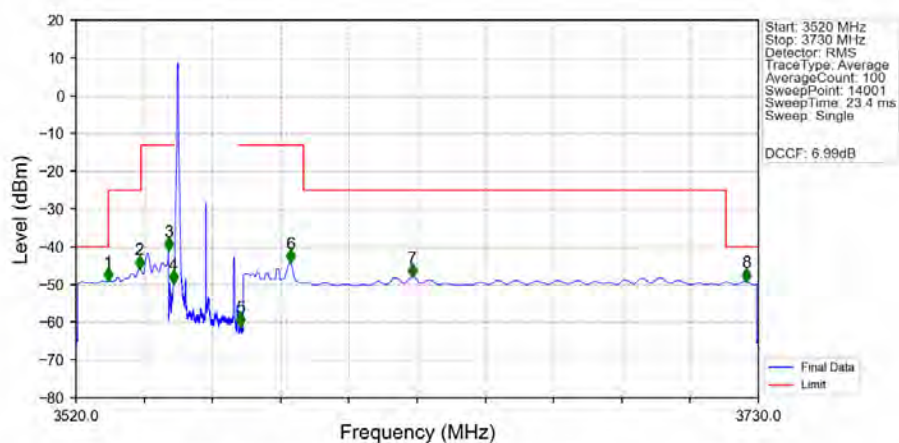
n48_30kHz_MIMO_NTNV_20MHz_CP-OFDM_QPSK_3560.01MHz_Inner_1RB_Left_MIMO
