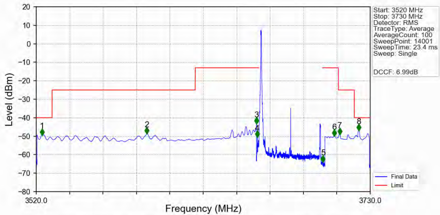
n48_30kHz_MIMO_NTNV_40MHz_DFT-s-OFDM_QPSK_3679.98MHz_Inner_1RB_Left_Ant2
