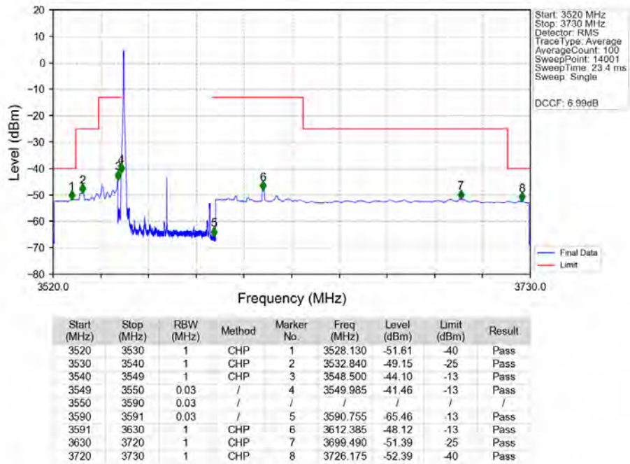
n48_30kHz_MIMO_NTNV_40MHz_CP-OFDM_QPSK_3570MHz_Edge_1RB_Left_Ant1
