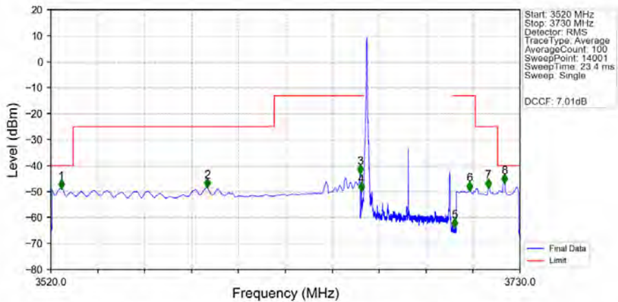
n48_30kHz_MIMO_NTNV_40MHz_DFT-s-OFDM_QPSK_3679.98MHz_Inner_1RB_Left_Ant1
