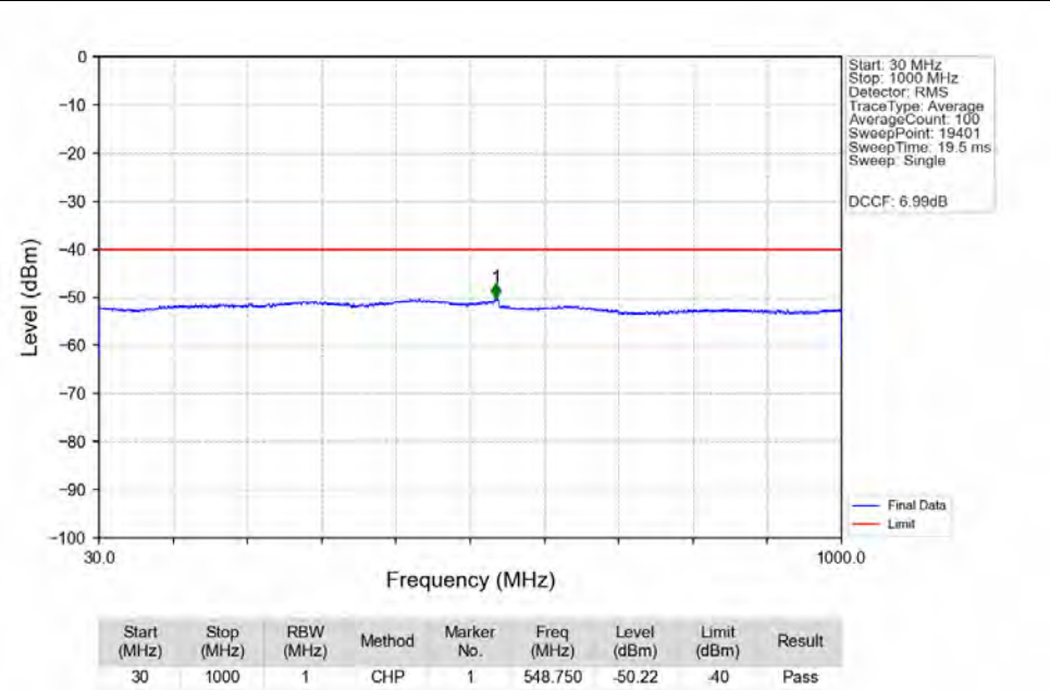
n48_30kHz_MIMO_NTNV_20MHz_CP-OFDM_QPSK_3560.01MHz_Edge_1RB_Left_Ant1
