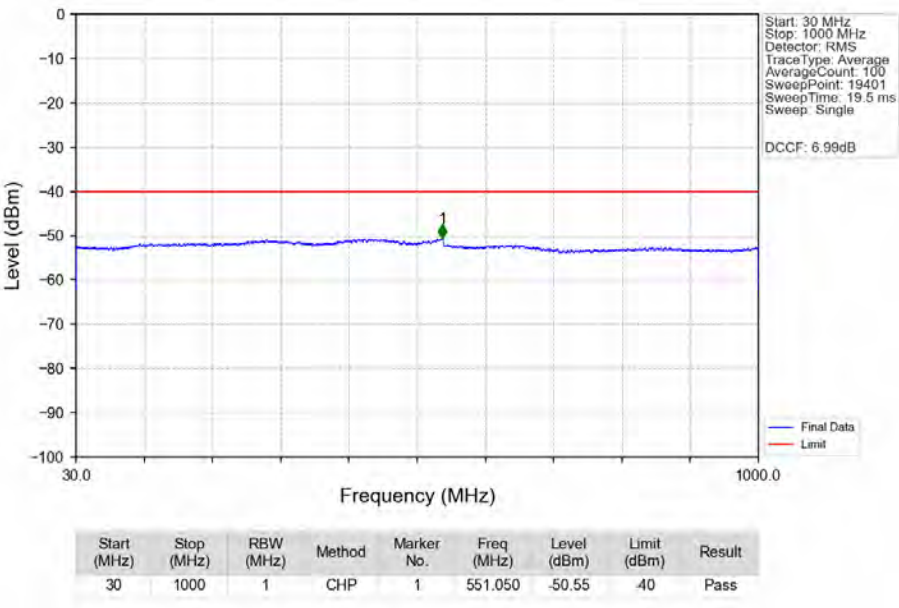
n48_30kHz_MIMO_NTNV_40MHz_CP-OFDM_QPSK_3570MHz_Edge_1RB_Left_Ant2
