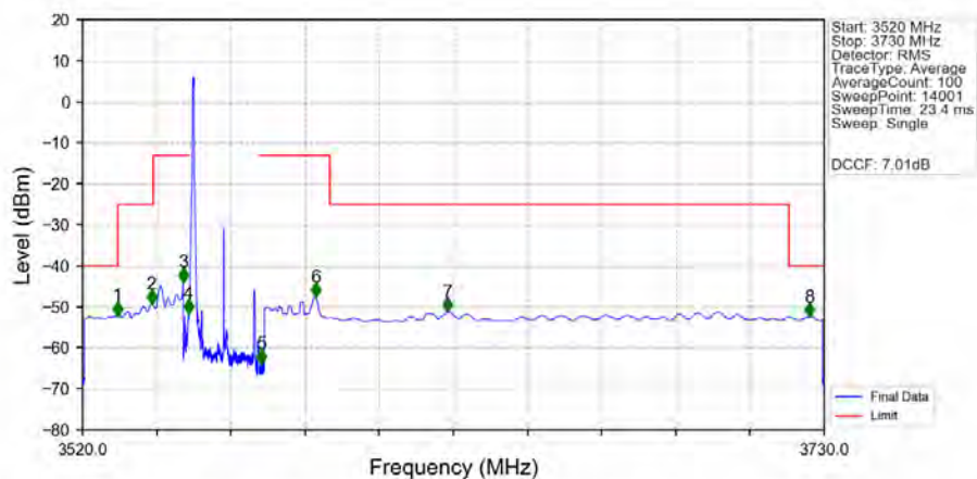
n48_30kHz_MIMO_NTNV_20MHz_CP-OFDM_QPSK_3560.01MHz_Inner_1RB_Left_Ant2
