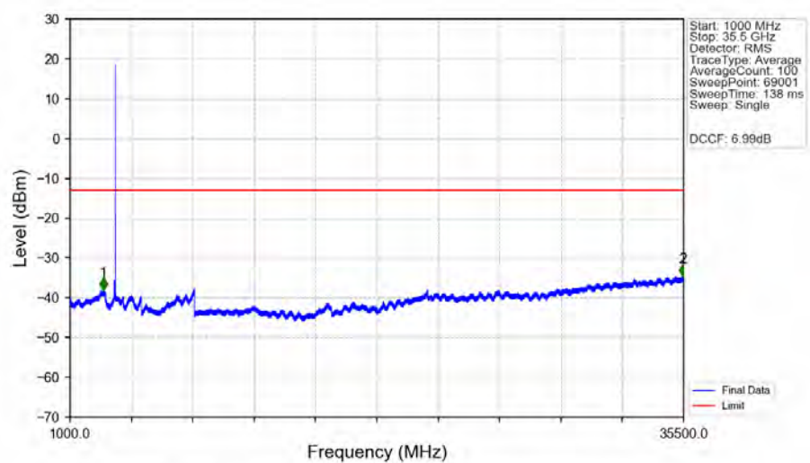
n78e_30kHz_SISO_NTNV_60MHz_CP-OFDM_QPSK_3519.99MHz_Edge_1RB_Right_Ant1
