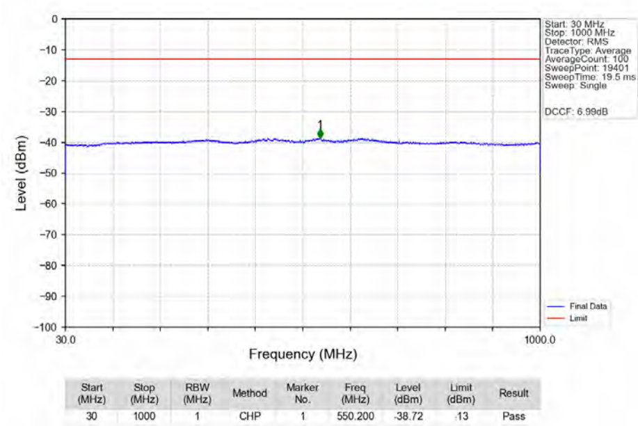
n78e_30kHz_SISO_NTNV_90MHz_DFT-s-OFDM_PI/2_BPSK_3500.01MHz_Edge_1RB_Left_Ant1
