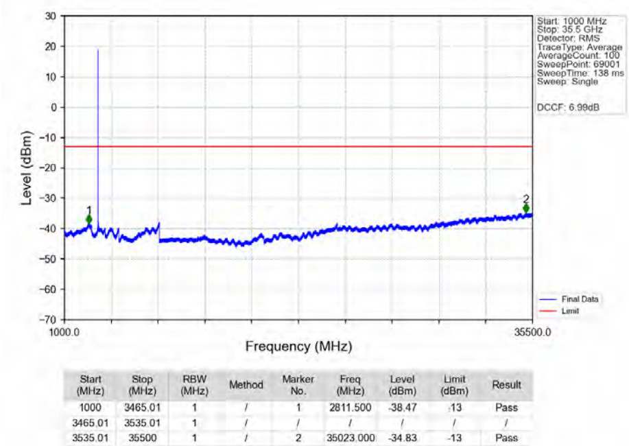
n78e_30kHz_SISO_NTNV_60MHz_DFT-s-OFDM_PI/2_BPSK_3519.99MHz_Edge_1RB_Right_Ant1
