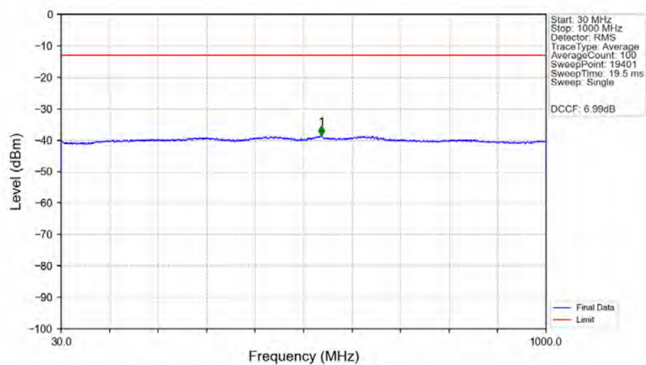
n78e_30kHz_SISO_NTNV_90MHz_CP-OFDM_QPSK_3504.99MHz_Edge_1RB_Right_Ant1
