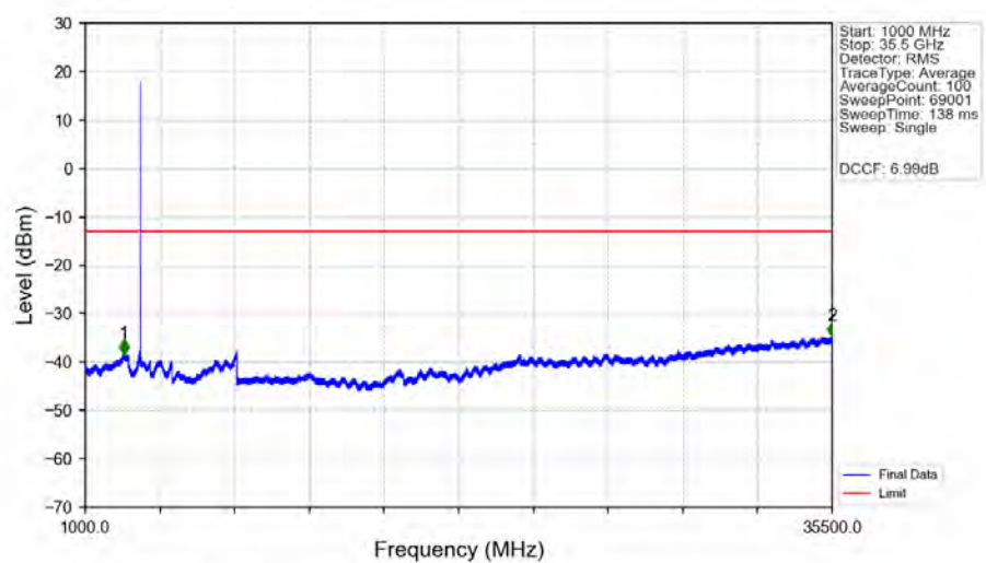
n78e_30kHz_SISO_NTNV_90MHz_CP-OFDM_QPSK_3504.99MHz_Edge_1RB_Right_Ant1
