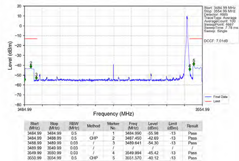
n78e_30kHz_SISO_NTNV_60MHz_DFT-s-OFDM_PI/2_BPSK_3519.99MHz_Edge_1RB_Right_Ant1
