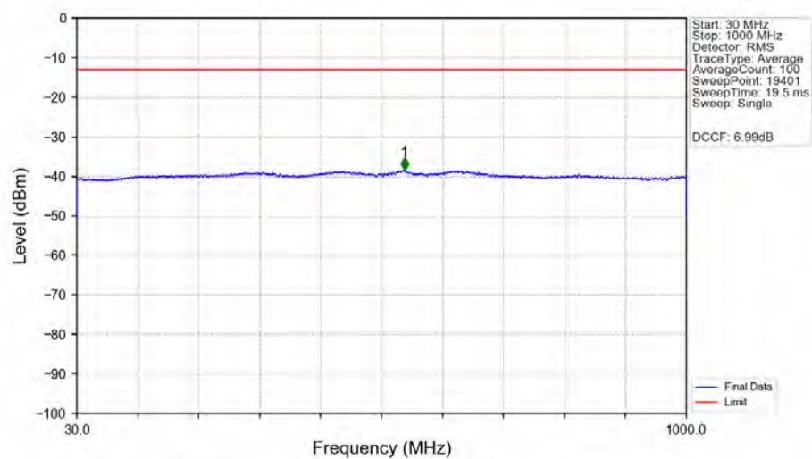
n78e_30kHz_SISO_NTNV_60MHz_CP-OFDM_QPSK_3519.99MHz_Edge_1RB_Right_Ant1
