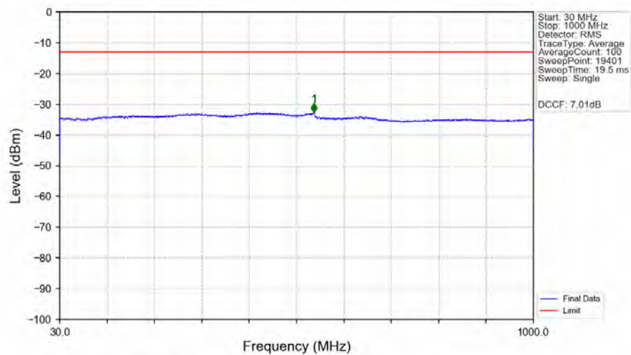
n77a_30kHz_MIMO_NTNV_100MHz_DFT-s-OFDM PI/2 BPSK_3750MHz_Edge_1RB_Left_Ant1
