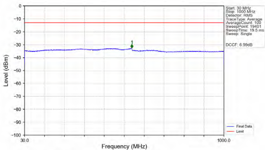
n77a_30kHz_MIMO_NTNV_90MHz_CP-OFDM_QPSK_3745.02MHz_Edge_1RB_Left_Ant2
