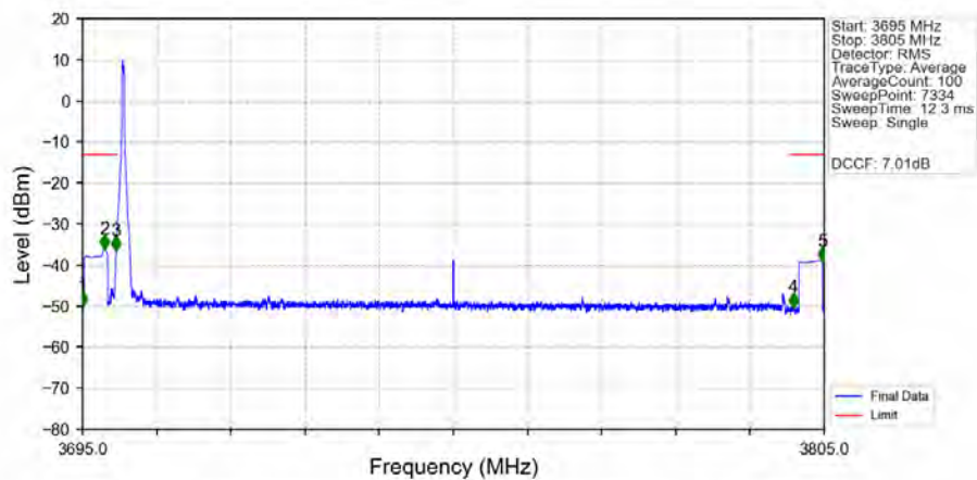
n77a_30kHz_MIMO_NTNV_100MHz_DFT-s-OFDM PI/2 BPSK_3750MHz_Edge_1RB_Left_Ant1
