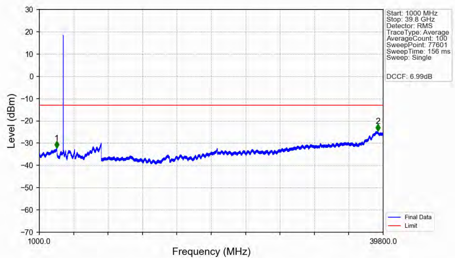
n77a_30kHz_MIMO_NTNV_100MHz_DFT-s-OFDM_PI/2_BPSK_3750MHz_Edge_1RB_Left_Ant2
