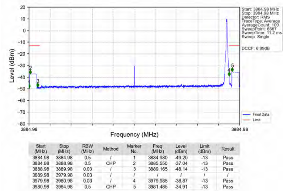
n77a_30kHz_MIMO_NTNV_90MHz_CP-OFDM_QPSK_3934.98MHz_Edge_1RB_Right_Ant2
