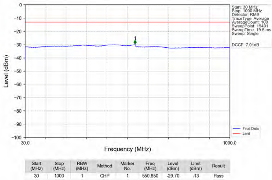
n77a_30kHz_MIMO_NTNV_90MHz_CP-OFDM_QPSK_3745.02MHz_Edge_1RB_Left_MIMO
