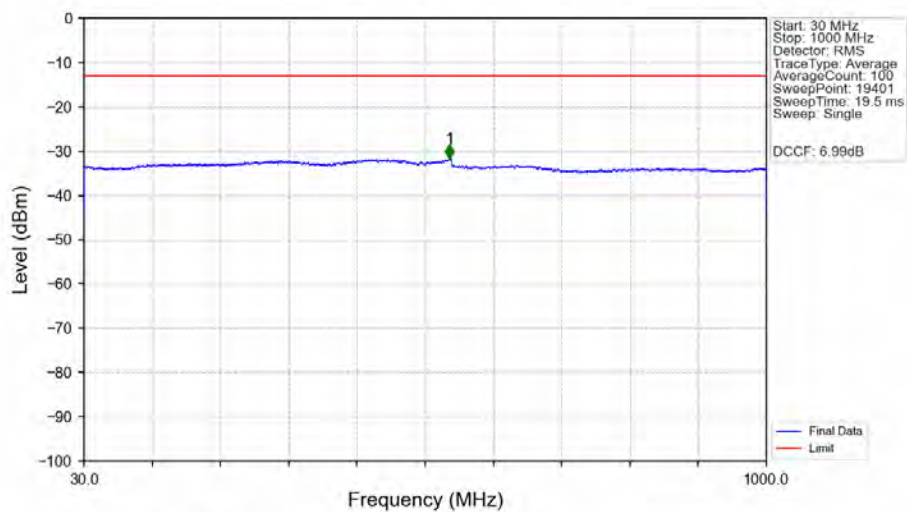
n77a_30kHz_MIMO_NTNV_60MHz_CP-OFDM_QPSK_3949.98MHz_Edge_1RB_Right_Ant1
