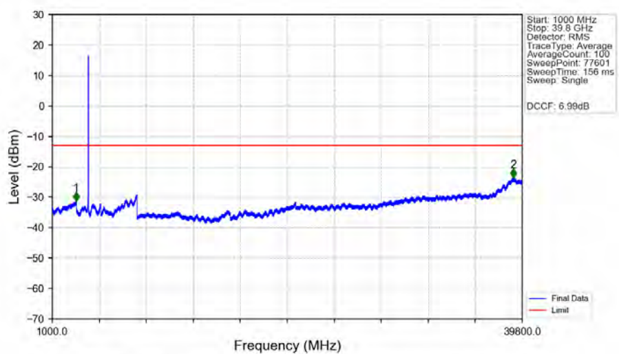
n77a_30kHz_MIMO_NTNV_60MHz_CP-OFDM_QPSK_3949.98MHz_Edge_1RB_Right_Ant1
