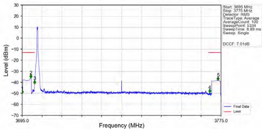
n77a_30kHz_MIMO_NTNV_70MHz_DFT-s-OFDM PI/2 BPSK_3735MHz_Edge_1RB_Left_Ant1
