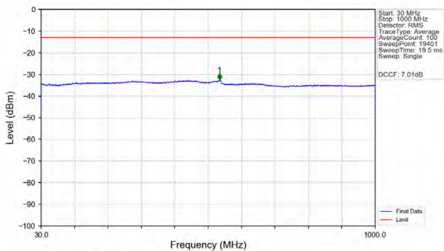
n77a_30kHz_MIMO_NTNV_70MHz_DFT-s-OFDM PI/2 BPSK_3735MHz_Edge_1RB_Left_Ant1
