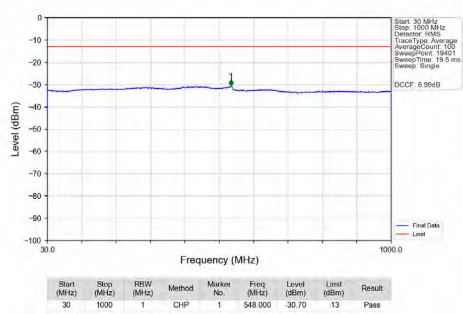
n77a_30kHz_MIMO_NTNV_50MHz_CP-OFDM_QPSK_3954.99MHz_Edge_1RB_Right_Ant2
