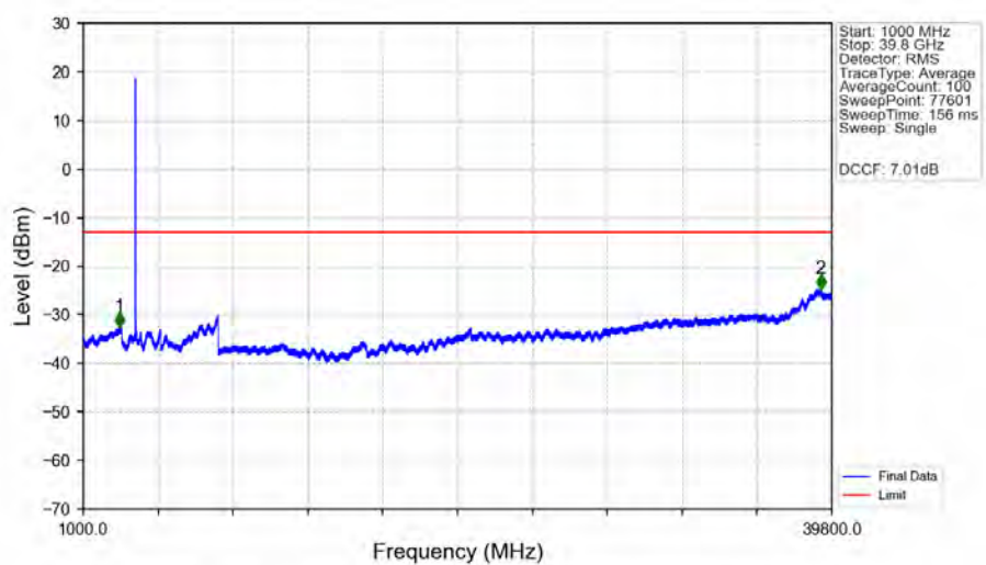
n77a_30kHz_MIMO_NTNV_60MHz_DFT-s-OFDM_QPSK_3730.02MHz_Edge_1RB_Left_Ant2
