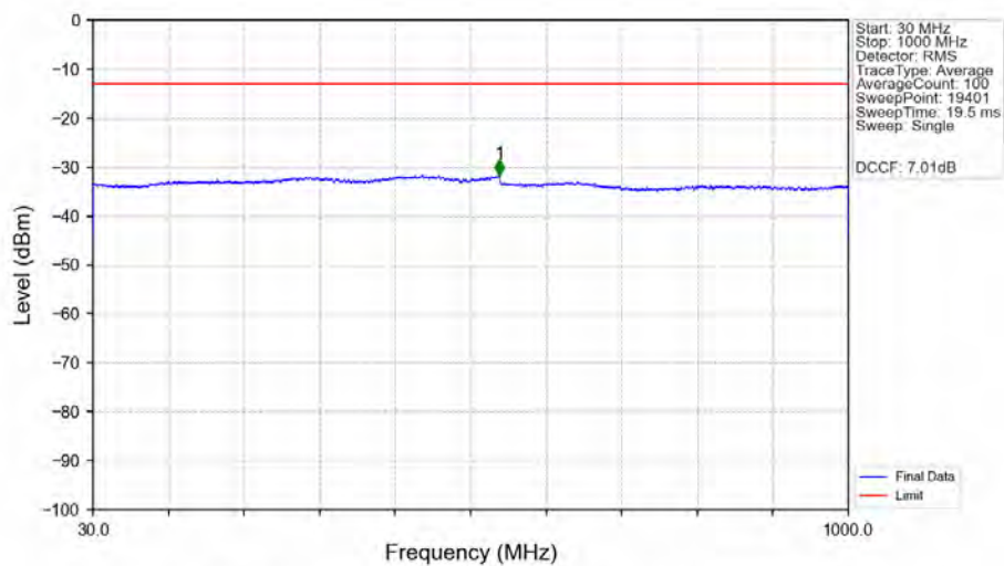
n77a_30kHz_MIMO_NTNV_50MHz_CP-OFDM_QPSK_3954.99MHz_Edge_1RB_Right_Ant1
