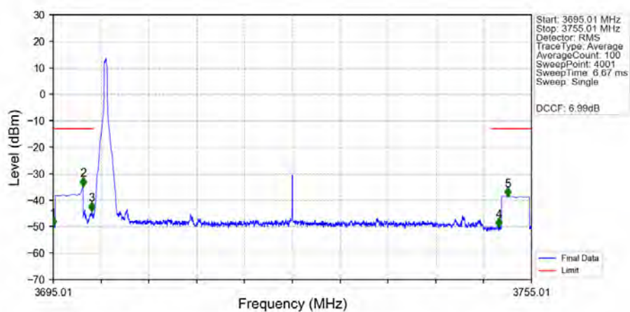
n77a_30kHz_MIMO_NTNV_50MHz_CP-OFDM_QPSK_3725.01MHz_Inner_1RB_Left_Ant2
