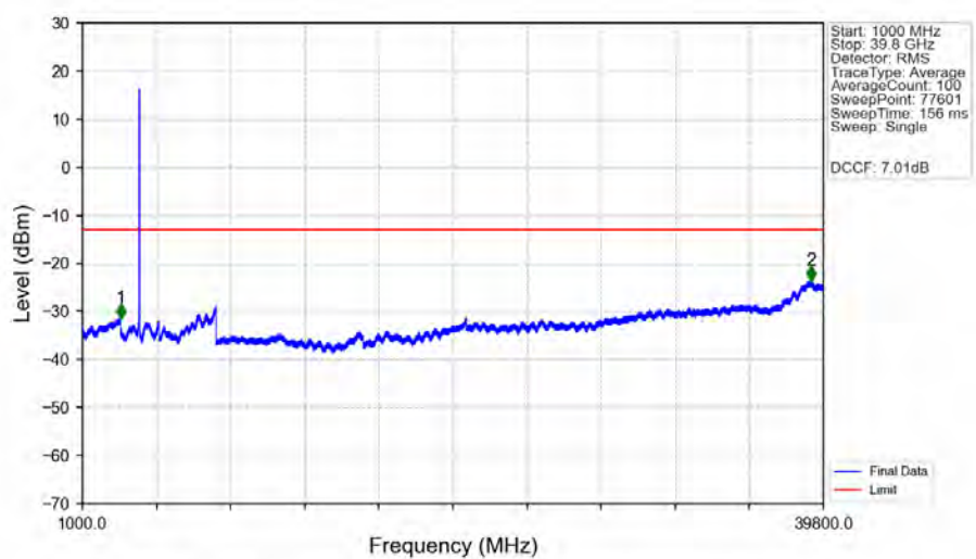
n77a_30kHz_MIMO_NTNV_50MHz_CP-OFDM_QPSK_3954.99MHz_Edge_1RB_Right_Ant1
