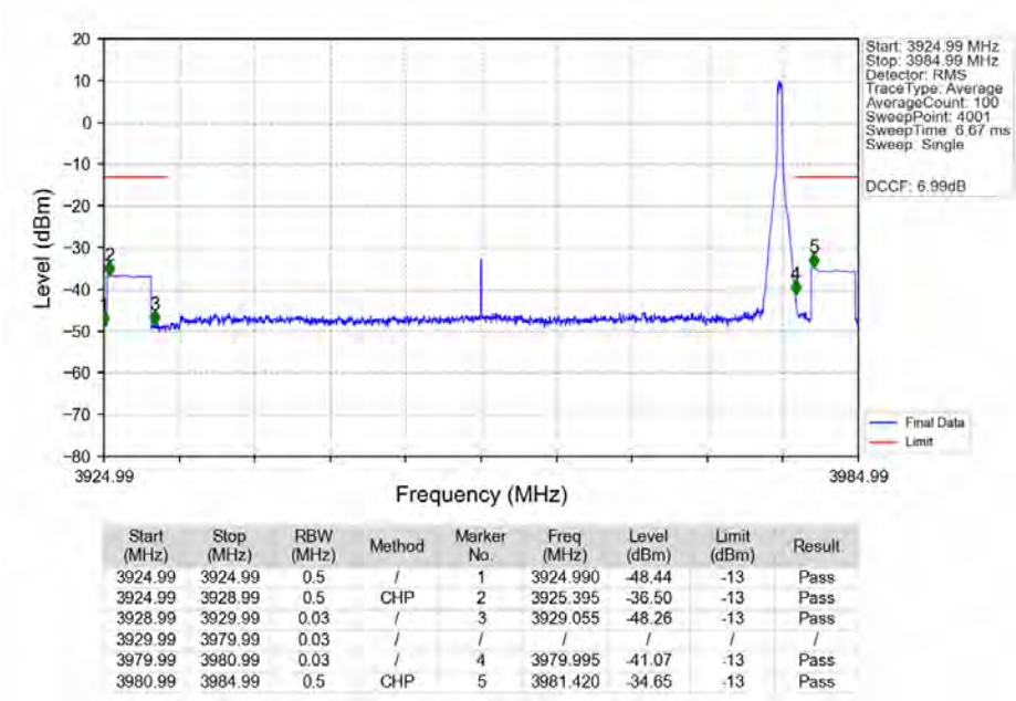
n77a_30kHz_MIMO_NTNV_50MHz_CP-OFDM_QPSK_3954.99MHz_Edge_1RB_Right_Ant2
