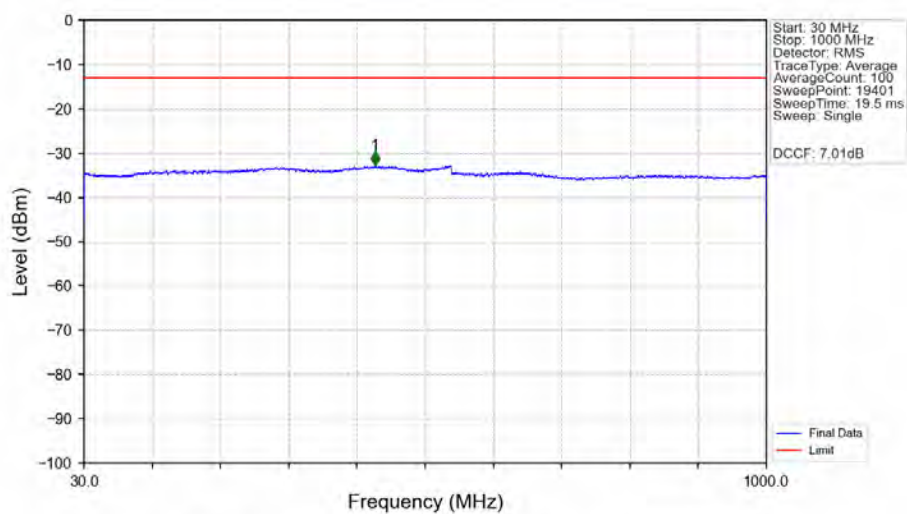
n77a_30kHz_MIMO_NTNV_60MHz_DFT-s-OFDM_QPSK_3730.02MHz_Edge_1RB_Left_Ant2
