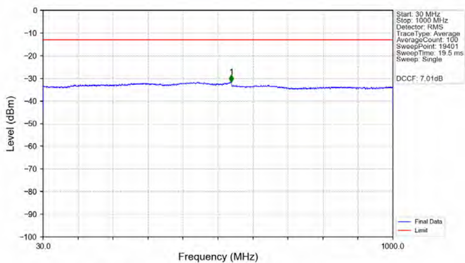
n77a_30kHz_MIMO_NTNV_30MHz_CP-OFDM_QPSK_3964.98MHz_Edge_1RB_Right_Ant1
