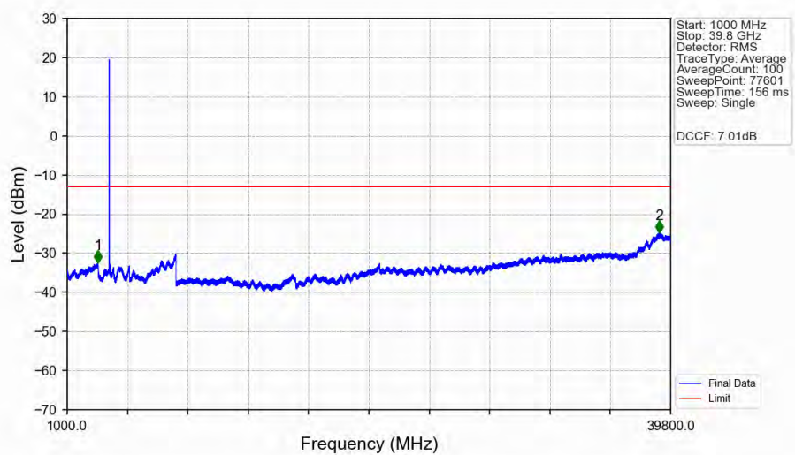
n77a_30kHz_MIMO_NTNV_50MHz_CP-OFDM_QPSK_3725.01MHz_Edge_1RB_Left_Ant2
