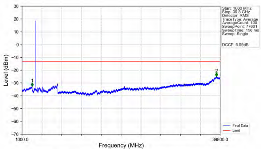
n77a_30kHz_MIMO_NTNV_30MHz_CP-OFDM_QPSK_3715.02MHz_Edge_1RB_Left_Ant2
