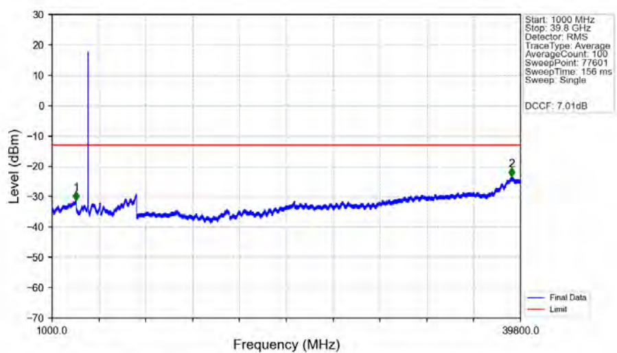
n77a_30kHz_MIMO_NTNV_30MHz_CP-OFDM_QPSK_3964.98MHz_Edge_1RB_Right_Ant1
