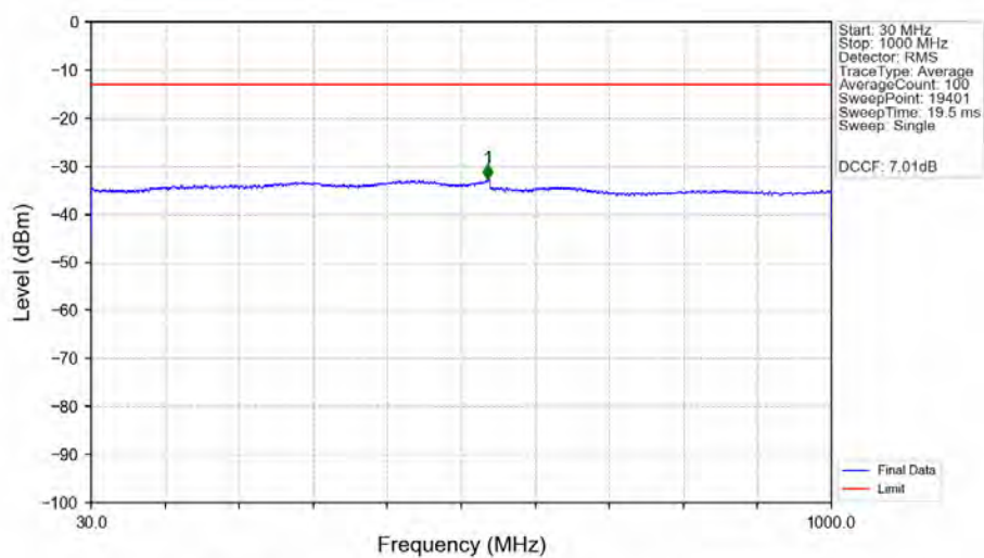
n77a_30kHz_MIMO_NTNV_50MHz_CP-OFDM_QPSK_3725.01MHz_Edge_1RB_Left_Ant2
