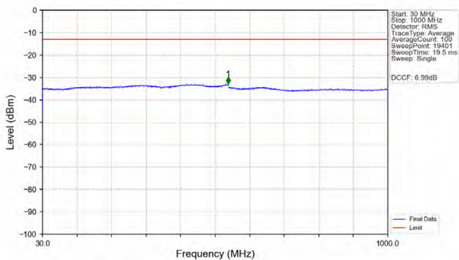
n77a_30kHz_MIMO_NTNV_30MHz_CP-OFDM_QPSK_3715.02MHz_Edge_1RB_Left_Ant2
