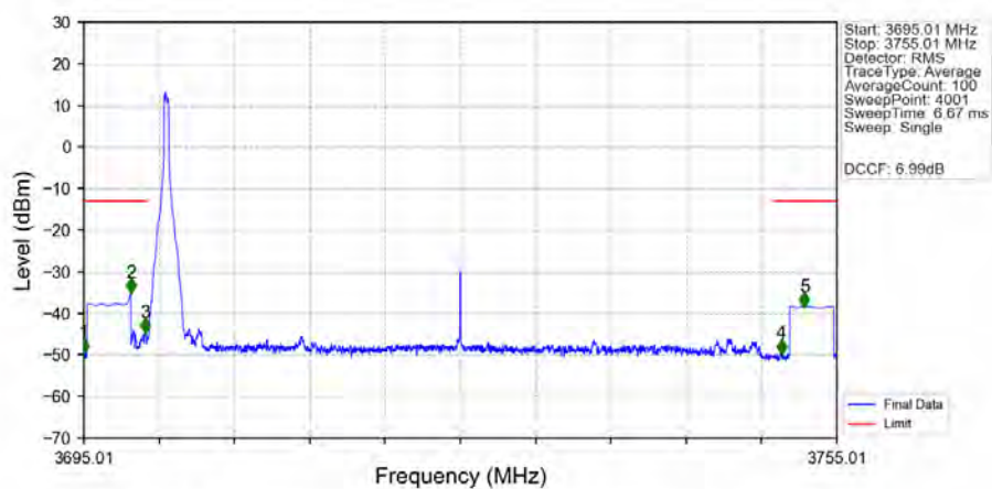
n77a_30kHz_MIMO_NTNV_50MHz_CP-OFDM_QPSK_3725.01MHz_Inner_1RB_Left_Ant1
