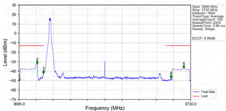
n77a_30kHz_MIMO_NTNV_25MHz_DFT-s-OFDM_PI/2_BPSK_3712.5MHz_Inner_1RB_Left_Ant1
