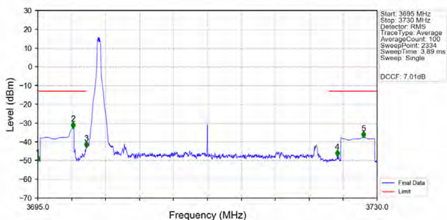
n77a_30kHz_MIMO_NTNV_25MHz_DFT-s-OFDM_PI/2_BPSK_3712.5MHz_Inner_1RB_Left_Ant2
