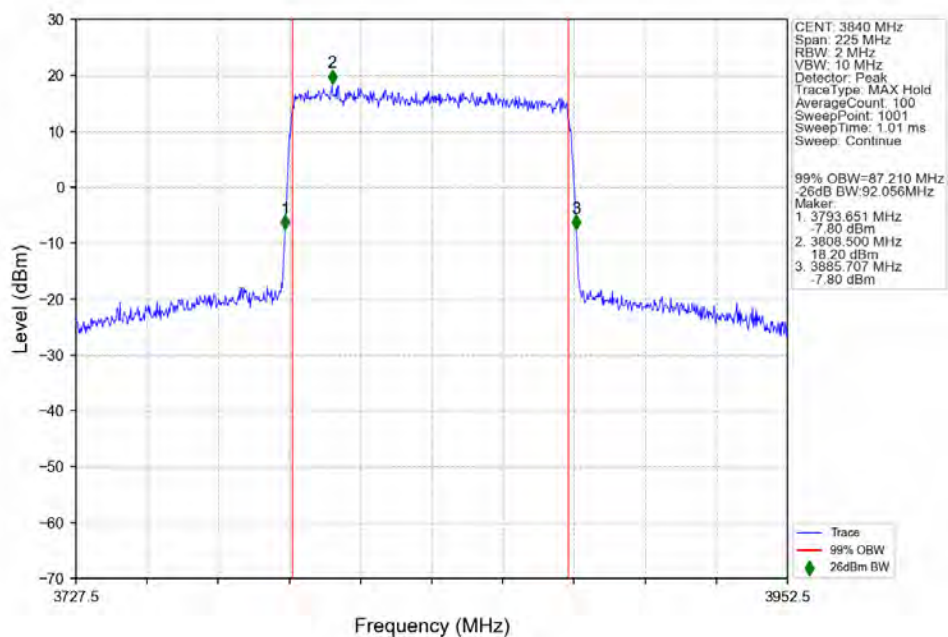
n77a_30kHz_SISO_NTNV_90MHz_DFT-s-OFDM_16_QAM_3840MHz_Outer_Full_Ant1
