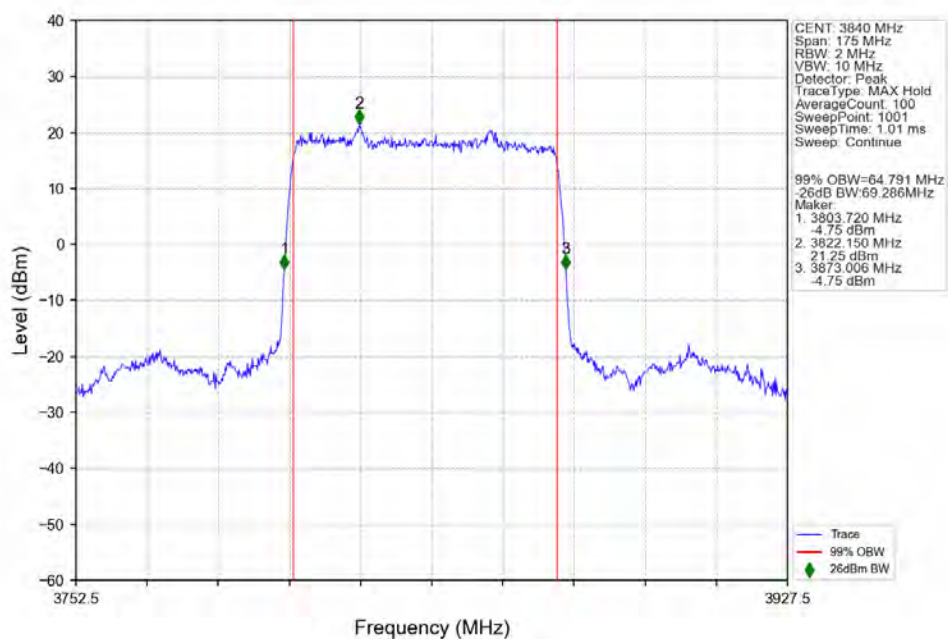
n77a_30kHz_SISO_NTNV_70MHz_DFT-s-OFDM PI/2 BPSK_3840MHz_Outer_Full_Ant1
