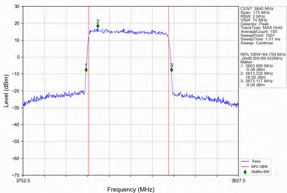
n77a_30kHz_SISO_NTNV_70MHz_DFT-s-OFDM_256_QAM_3840MHz_Outer_Full_Ant1
