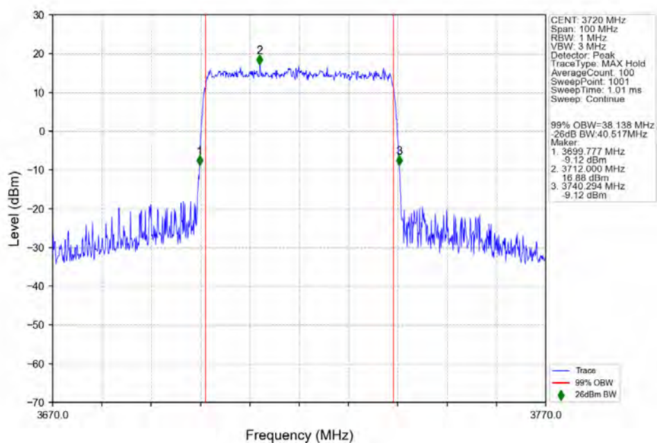
n77a_30kHz_SISO_NTNV_40MHz_CP-OFDM_QPSK_3720MHz_Outer_Full_Ant1
