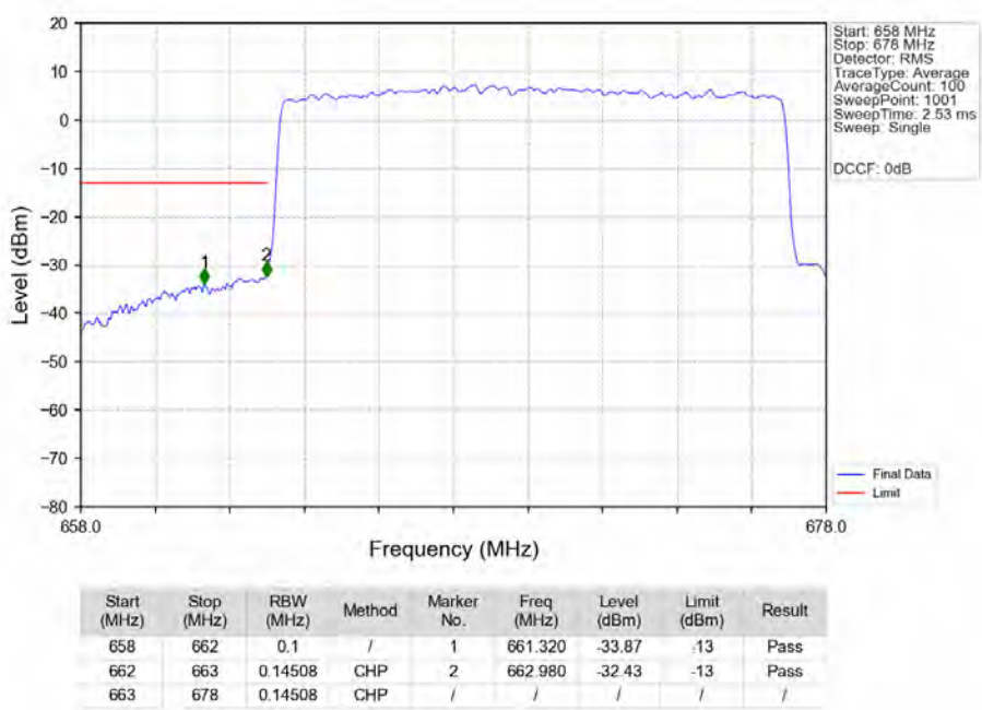
n71 15kHz SISO NTN 15MHz DFT-s-OFDM QPSK 670.5MHz Outer Full Ant1
