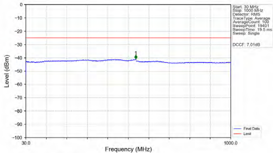
n41_30kHz_MIMO_NTNV_90MHz_DFT-s-OFDM PI/2 BPSK_2541MHz_Edge_1RB_Left_Ant1
