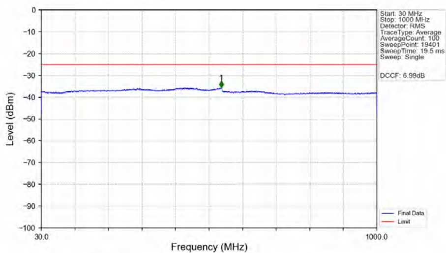
n41_30kHz_MIMO_NTNV_80MHz_DFT-s-OFDM_PI/2_BPSK_2536.02MHz_Edge_1RB_Left_Ant2
