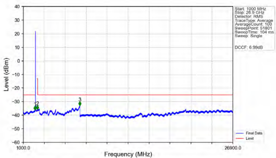
n41_30kHz_MIMO_NTNV_80MHz_DFT-s-OFDM_PI/2_BPSK_2536.02MHz_Edge_1RB_Left_Ant2
