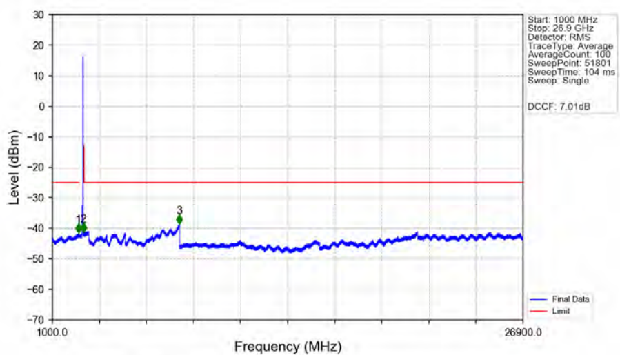
n41_30kHz_MIMO_NTNV_50MHz_CP-OFDM_QPSK_2664.99MHz_Edge_1RB_Right_Ant1
