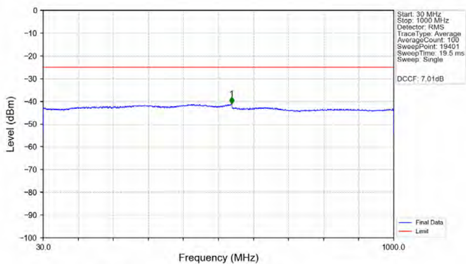
n41_30kHz_MIMO_NTNV_50MHz_CP-OFDM_QPSK_2664.99MHz_Edge_1RB_Right_Ant1
