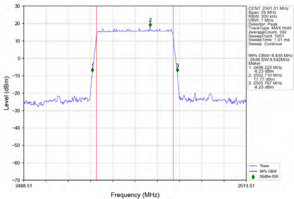
n41_30kHz_SISO_NTNV_10MHz_DFT-s-OFDM_QPSK_2501.01MHz_Outer_Full_Ant1
