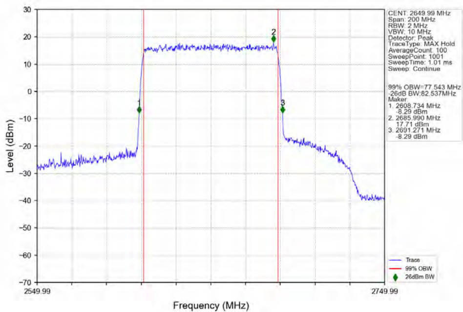
n41_30kHz_SISO_NTNV_80MHz_DFT-s-OFDM_QPSK_2649.99MHz_Outer_Full_Ant1
