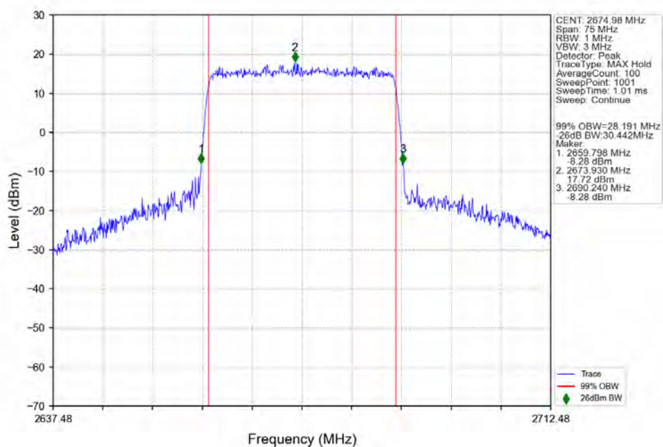
n41_30kHz_SISO_NTNV_30MHz_CP-OFDM_QPSK_2674.98MHz_Outer_Full_Ant1
