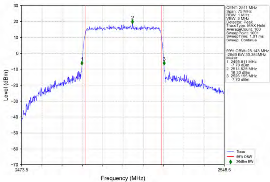
n41_30kHz_SISO_NTNV_30MHz_CP-OFDM_QPSK_2511MHz_Outer_Full_Ant1
