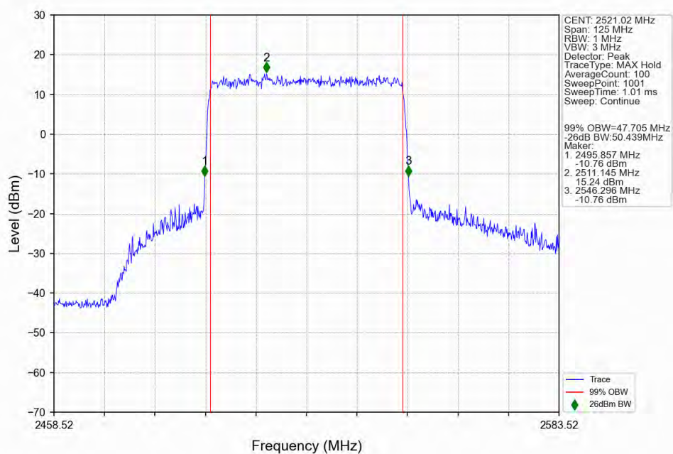
n41_30kHz_SISO_NTNV_50MHz_CP-OFDM_QPSK_2521.02MHz_Outer_Full_Ant1
