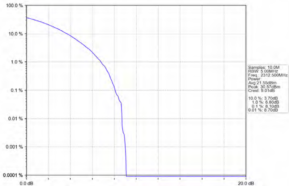
n30 15kHz SISO NTN 5MHz CP-OFDM 16 QAM 2312.5MHz Outer Full Ant1
