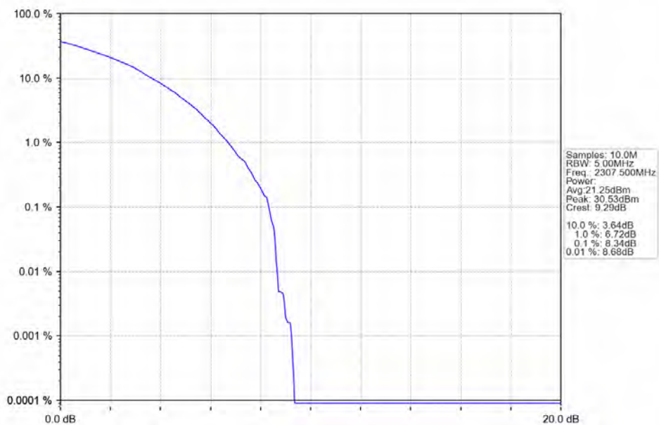
n30 15kHz SISO NTN 5MHz CP-OFDM 64 QAM 2307.5MHz Outer Full Ant1
