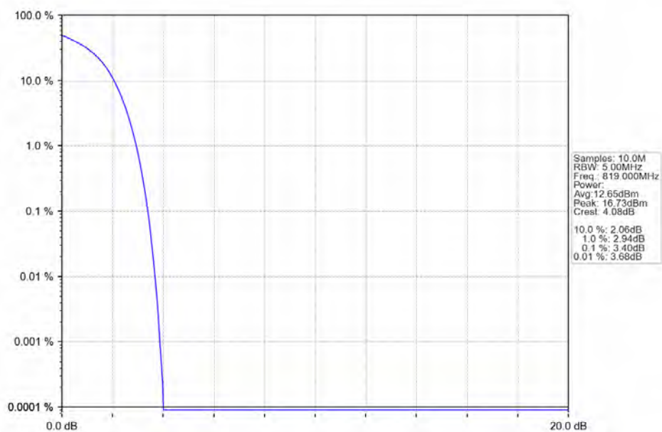
n26a 15kHz SISO NTN 5MHz CP-OFDM 16 QAM 819MHz Outer Full Ant1
