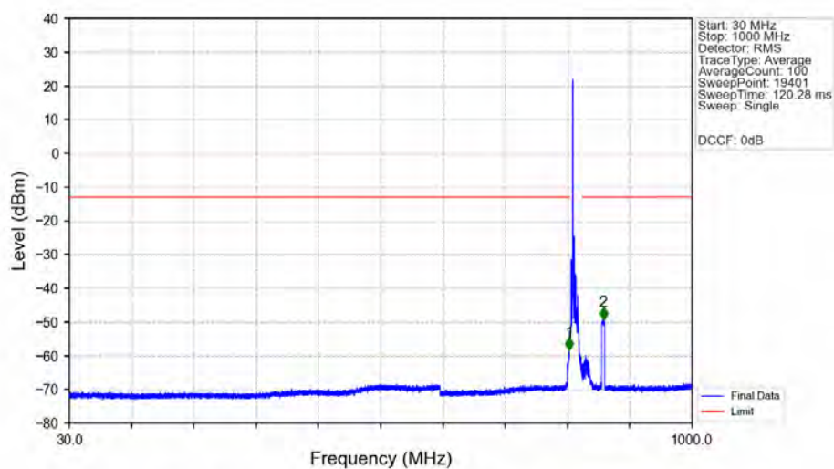
n26a_15kHz_SISO_NTNV_5MHz_DFT-s-OFDM_PI/2_BPSK_816.5MHz_Edge_1RB_Left_Ant1
