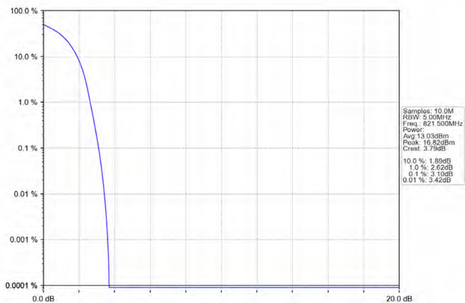
n26a 15kHz SISO NTN 5MHz DFT-s-OFDM 64 QAM 821.5MHz Outer Full Ant1
