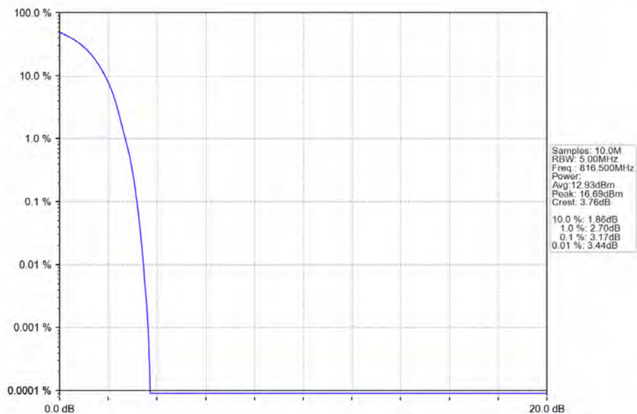
n26a_15kHz_SISO_NTNV_5MHz_DFT-s-OFDM_QPSK_816.5MHz_Outer_Full_Ant1
