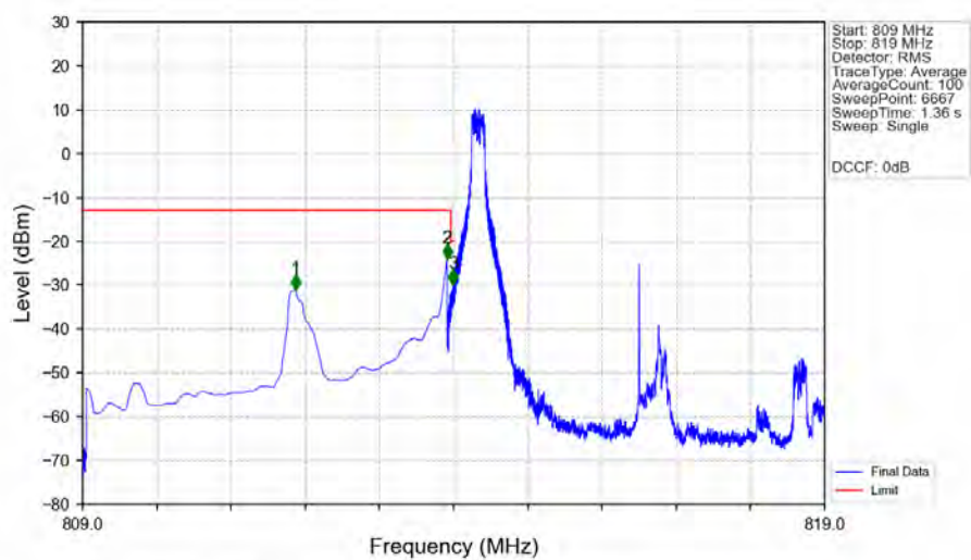
n26a_15kHz_SISO_NTNV_5MHz_DFT-s-OFDM_PI/2_BPSK_816.5MHz_Edge_1RB_Left_Ant1
