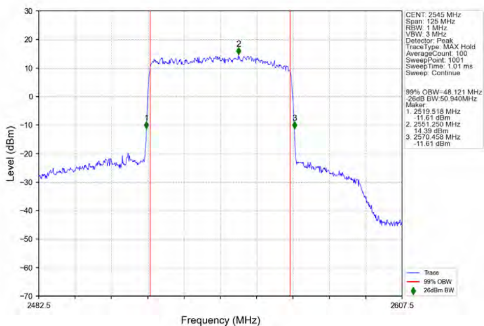
n7_15kHz_SISO_NTNV_50MHz_DFT-s-OFDM_QPSK_2545MHz_Outer_Full_Ant1
