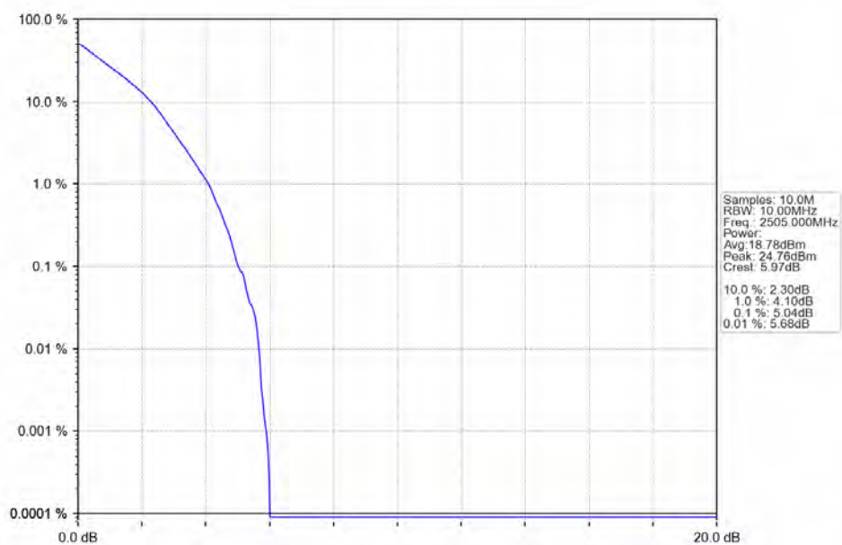
n7_15kHz_SISO_NTNV_10MHz_DFT-s-OFDM QPSK_2505MHz_Outer_Full_Ant1
