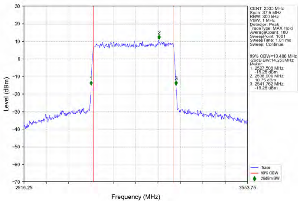
n7_15kHz_SISO_NTNV_15MHz_DFT-s-OFDM_256_QAM_2535MHz_Outer_Full_Ant1
