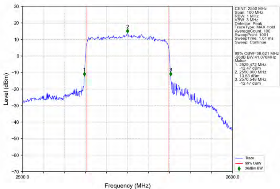
n7_15kHz_SISO_NTNV_40MHz_CP-OFDM_64_QAM_2550MHz_Outer_Full_Ant1
