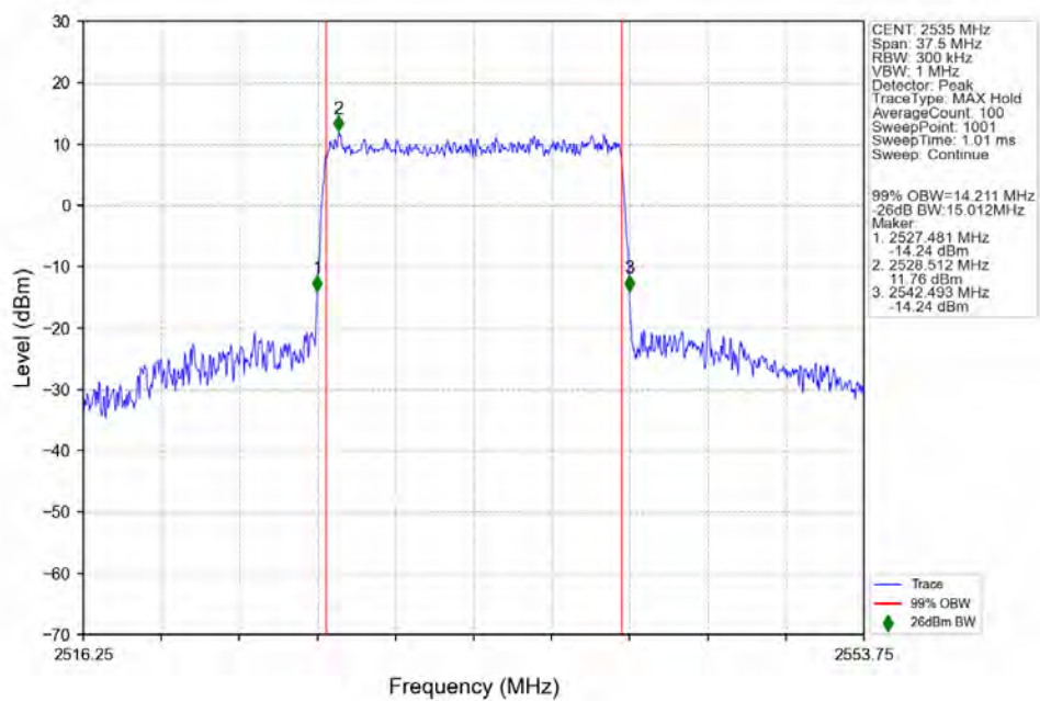
n7_15kHz_SISO_NTNV_15MHz_CP-OFDM_16_QAM_2535MHz_Outer_Full_Ant1
