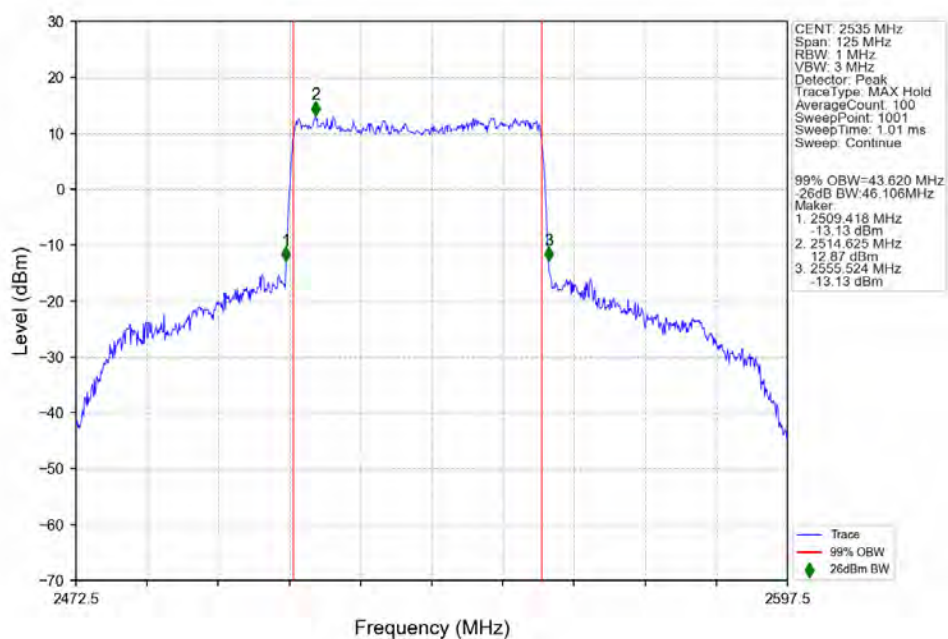
n7_15kHz_SISO_NTNV_50MHz_CP-OFDM_16_QAM_2535MHz_Outer_Full_Ant1
