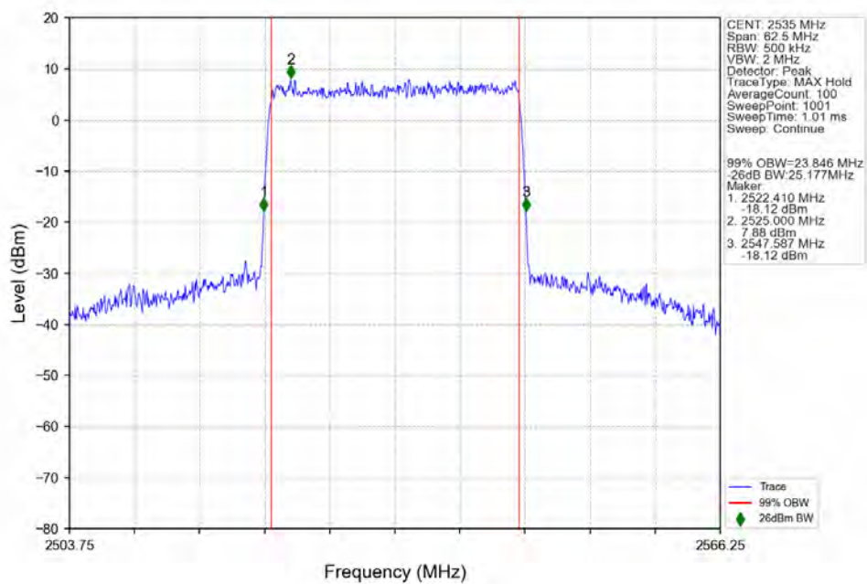
n7_15kHz_SISO_NTNV_25MHz_CP-OFDM_256_QAM_2535MHz_Outer_Full_Ant1
