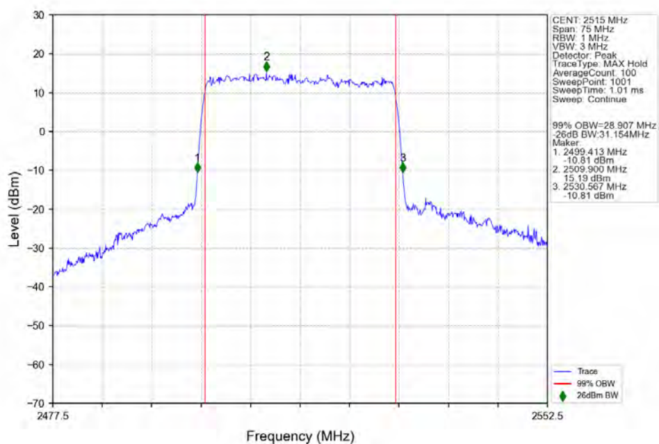
n7_15kHz_SISO_NTNV_30MHz_DFT-s-OFDM_64_QAM_2515MHz_Outer_Full_Ant1
