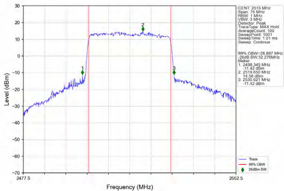
n7_15kHz_SISO_NTNV_30MHz_CP-OFDM_QPSK_2515MHz_Outer_Full_Ant1
