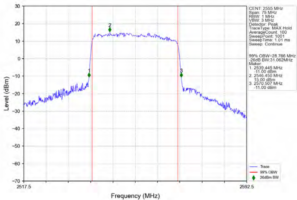
n7_15kHz_SISO_NTNV_30MHz_CP-OFDM_QPSK_2555MHz_Outer_Full_Ant1
