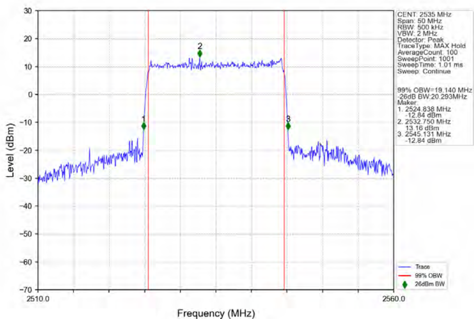
n7_15kHz_SISO_NTNV_20MHz_CP-OFDM_16_QAM_2535MHz_Outer_Full_Ant1
