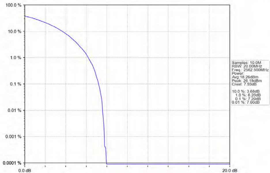
n7_15kHz_SISO_NTNV_15MHz_CP-OFDM_16_QAM_2562.5MHz_Outer_Full_Ant1
