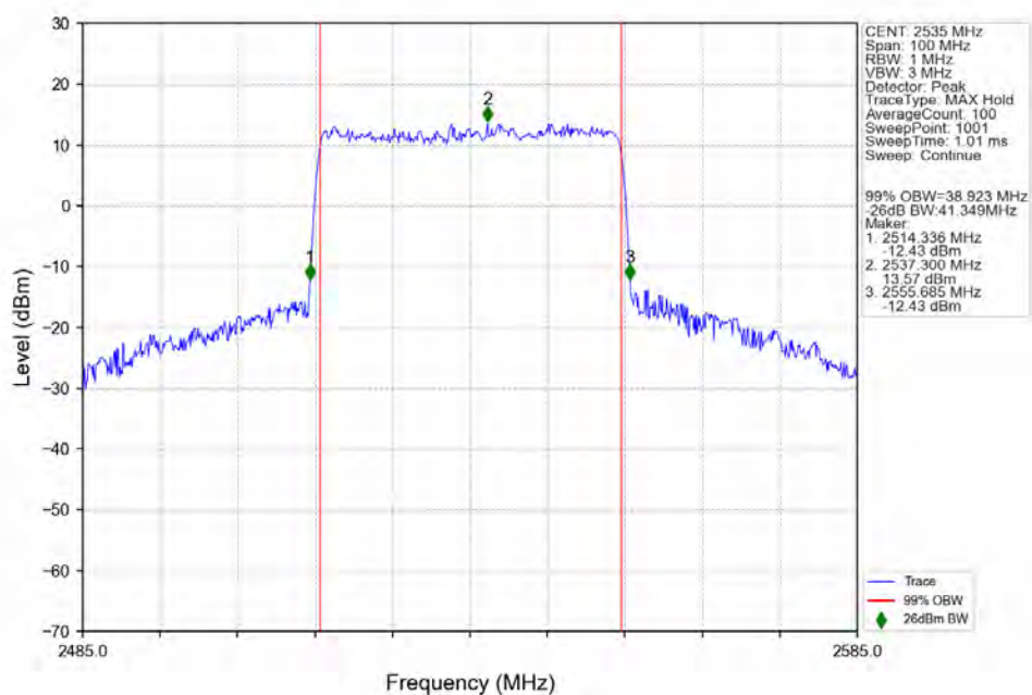
n7_15kHz_SISO_NTNV_40MHz_CP-OFDM_16_QAM_2535MHz_Outer_Full_Ant1
