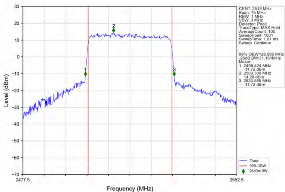
n7_15kHz_SISO_NTNV_30MHz_CP-OFDM_64_QAM_2515MHz_Outer_Full_Ant1
