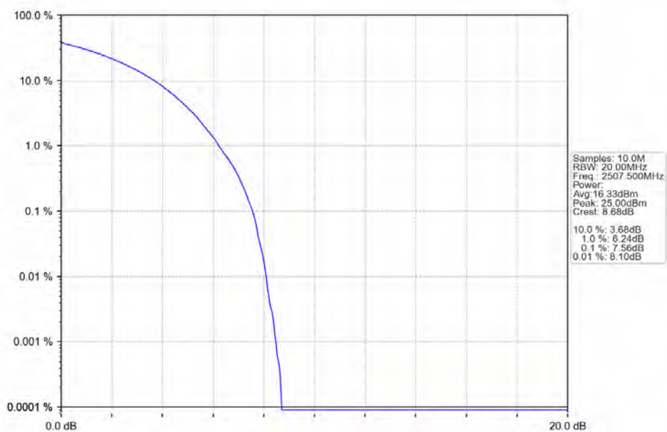
n7_15kHz_SISO_NTNV_15MHz_CP-OFDM_64_QAM_2507.5MHz_Outer_Full_Ant1
