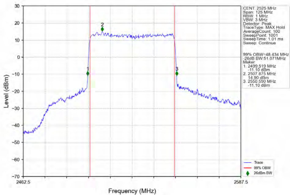
n7_15kHz_SISO_NTNV_50MHz_DFT-s-OFDM_QPSK_2525MHz_Outer_Full_Ant1
