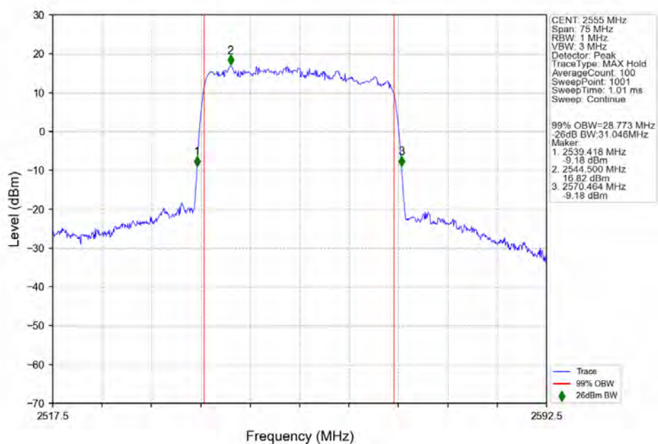
n7_15kHz_SISO_NTNV_30MHz_DFT-s-OFDM_QPSK_2555MHz_Outer_Full_Ant1
