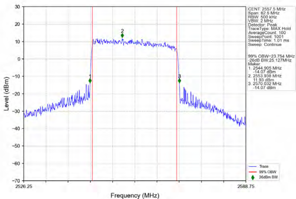
n7_15kHz_SISO_NTNV_25MHz_CP-OFDM_64_QAM_2557.5MHz_Outer_Full_Ant1
