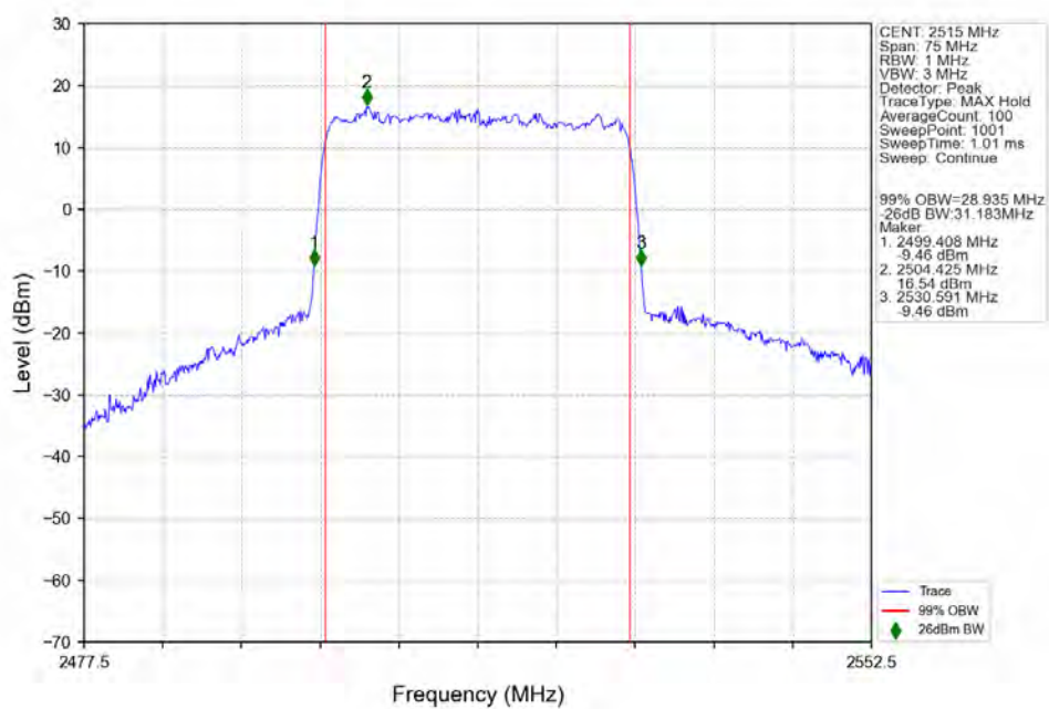
n7_15kHz_SISO_NTNV_30MHz_DFT-s-OFDM_QPSK_2515MHz_Outer_Full_Ant1
