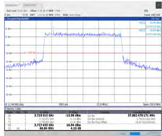
1-N78-3700-3800-PC2-30-60-M-8-CP-64QAM-Outer_Full-162@0-Ant0-57.882-60.840-≤60-PASS
