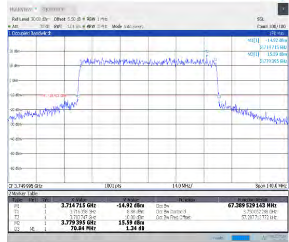
1-N78-3700-3800-PC2-30-70-M-7-CP-16QAM-Outer_Full-189@0-Ant0-67.39-70.840-≤70-PASS
