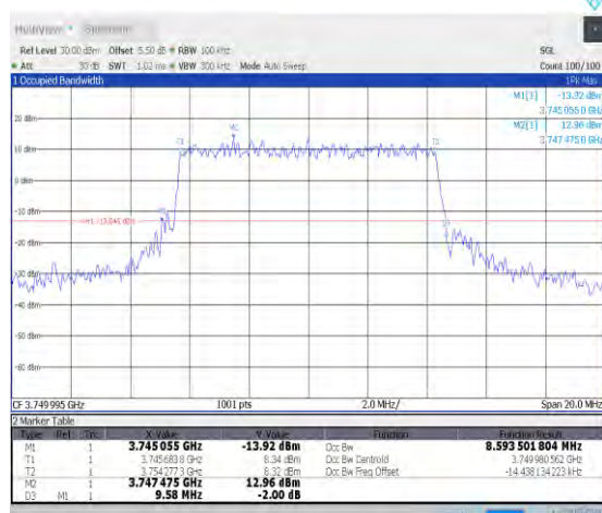
1-N78-3700-3800-PC2-30-10-M-8-CP-64QAM-Outer_Full-24@0-Ant0-8.594-9.580-≤10-PASS
