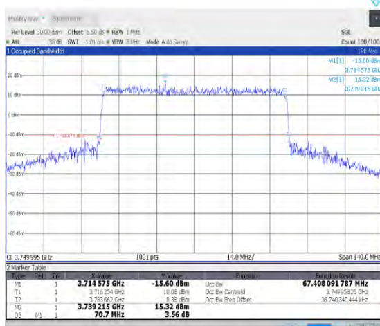
1-N78-3700-3800-PC2-30-70-M-8-CP-64QAM-Outer_Full-189@0-Ant0-67.408-70.700-≤70-PASS
