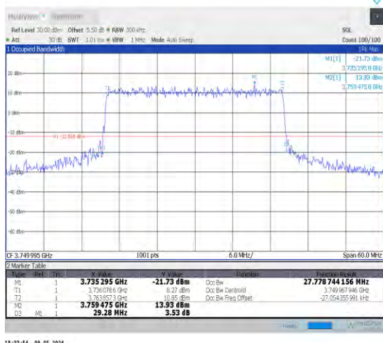
1-N78-3700-3800-PC2-30-30-M-6-CP-QPSK-Outer_Full-78@0-Ant0-27.78-29.280-≤30-PASS
