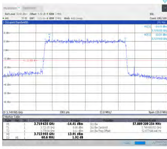
1-N78-3700-3800-PC2-30-60-M-9-CP-256QAM-Outer_Full-162@0-Ant0-57.889-60.600-≤60-PASS
