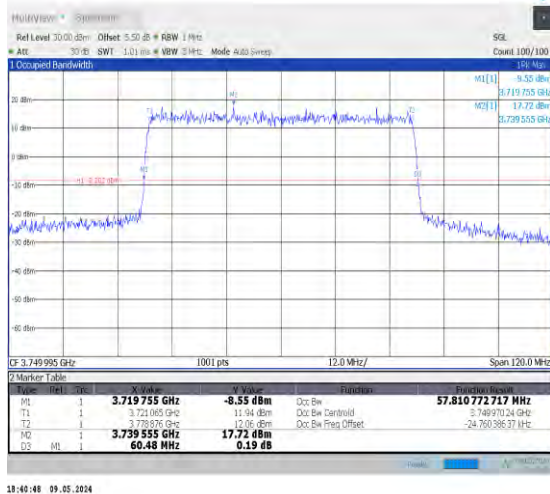
1-N78-3700-3800-PC2-30-60-M-7-CP-16QAM-Outer_Full-162@0-Ant0-57.811-60.480-≤60-PASS
