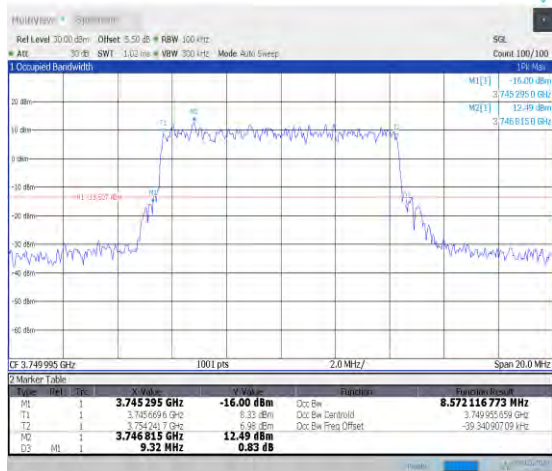
1-N78-3700-3800-PC2-30-10-M-5-DFT-256QAM-Outer_Full-24@0-Ant0-8.572-9.320-≤10-PASS
