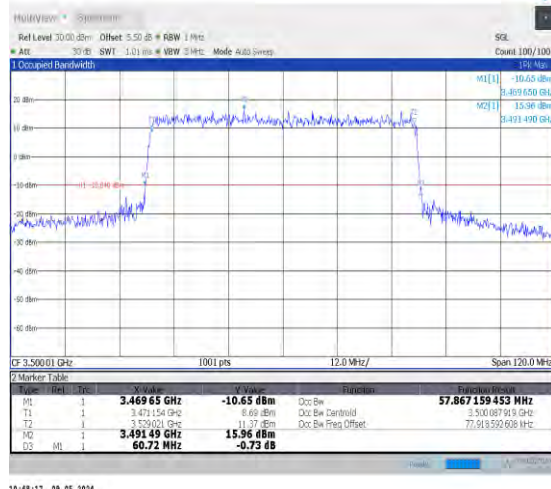
1-N78-3450-3550-PC2-30-60-M-8-CP-64QAM-Outer_Full-162@0-Ant0-57.867-60.720-≤60-PASS
