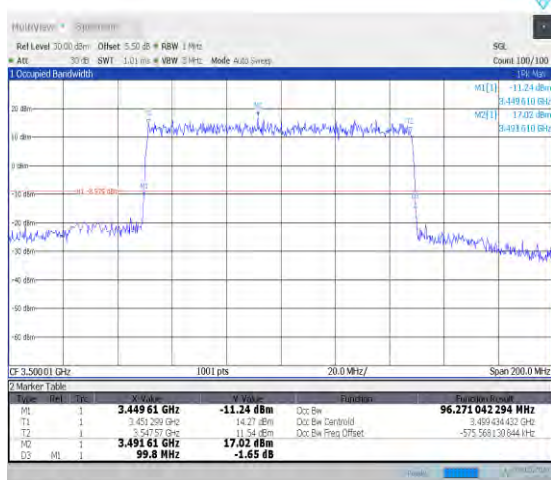
1-N78-3450-3550-PC2-30-100-M-1-DFT-QPSK-Outer_Full-270@0-Ant0-96.271-99.800-≤100-PASS
