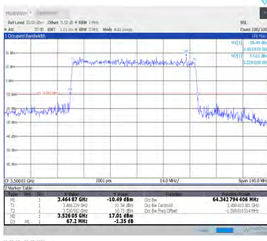
1-N78-3450-3550-PC2-30-70-M-4-DFT-64QAM-Outer_Full-180@0-Ant0-64.343-67.200-≤70-PASS
