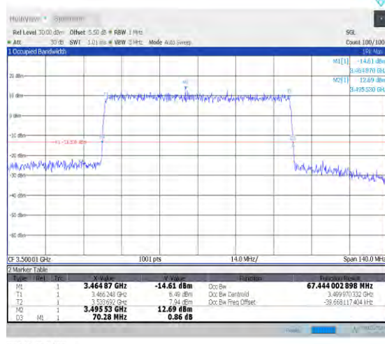
1-N78-3450-3550-PC2-30-70-M-9-CP-256QAM-Outer_Full-189@0-Ant0-67.444-70.280-≤70-PASS
