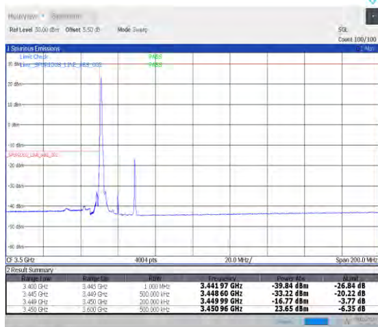
1-N78-3450-3550-PC2-30-20-L-1-DFT-PI2BPSK-Edge_1RB_Left-1@0-Ant0-1--PASS-see graph
