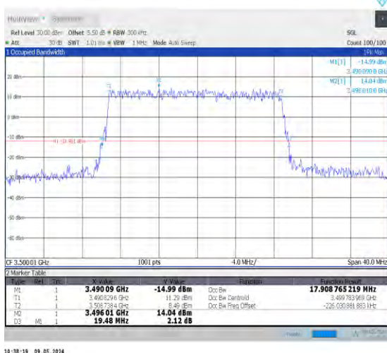
1-N78-3450-3550-PC2-30-20-M-5-DFT-256QAM-Out ter_Full-50@0-Ant0-17.909-19.480-≤20-PASS
