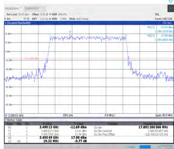
1-N78-3450-3550-PC2-30-20-M-2-DFT-PI2BPSK-Outer_Full-50@0-Ant0-17.892-19.320-≤20-PASS
