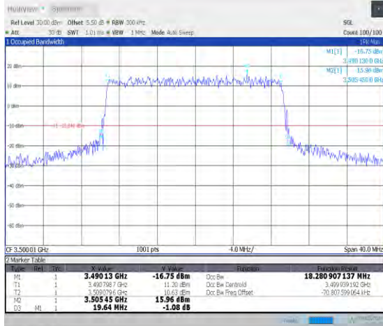
1-N78-3450-3550-PC2-30-20-M-7-CP-16QAM-Outer_Full-51@0-Ant0-18.281-19.640-≤20-PASS
