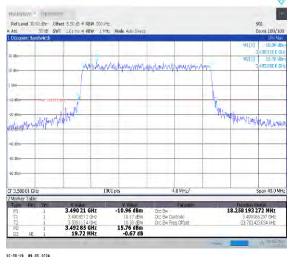
1-N78-3450-3550-PC2-30-20-M-6-CP-QPSK-Out Full-51@0-Ant0-18.258-19.720-≤20-PASS
