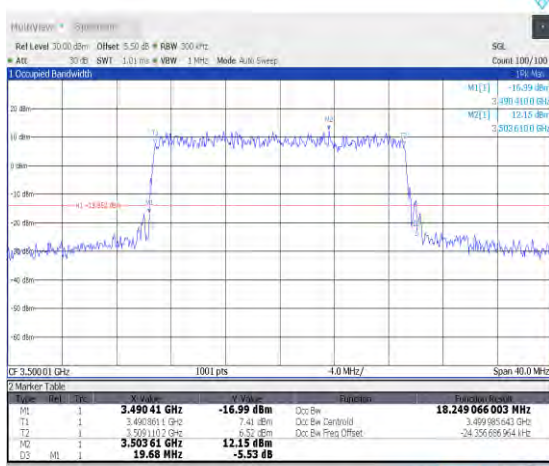
1-N78-3450-3550-PC2-30-20-M-9-CP-256QAM-Out er_Full-51@0-Ant0-18.249-19.680-≤20-PASS
