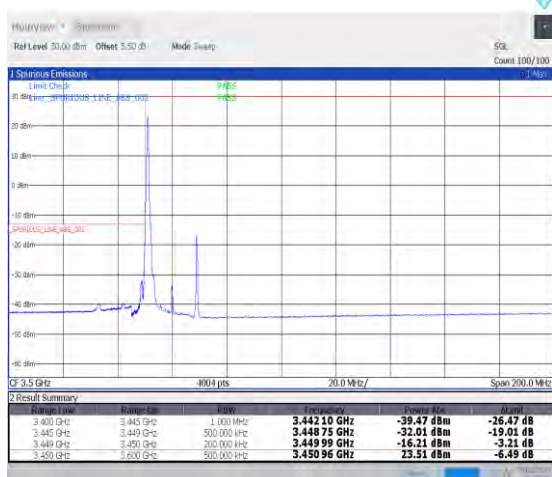
1-N78-3450-3550-PC2-30-20-L-4-CP-QPSK-Edge_1RB_Left-1@0-Ant0-1--PASS-see graph
