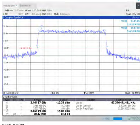
1-N78-3450-3550-PC2-30-70-M-7-CP-16QAM-Outer_Full-189@0-Ant0-67.346-70.420-≤70-PASS
