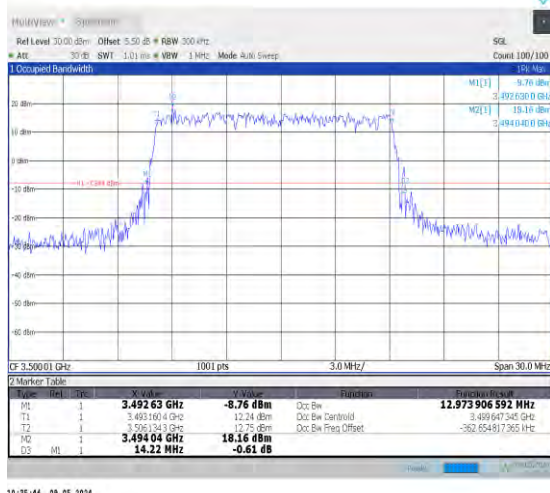
1-N78-3450-3550-PC2-30-15-M-4-DFT-64QAM-Out er_Full-36@0-Ant0-12.974-14.220-≤15-PASS
