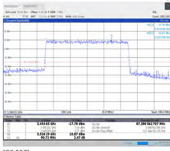
1-N78-3450-3550-PC2-30-90-M-9-CP-256QAM-Outer_Full-245@0-Ant0-87.381-90.720-≤90-PASS
