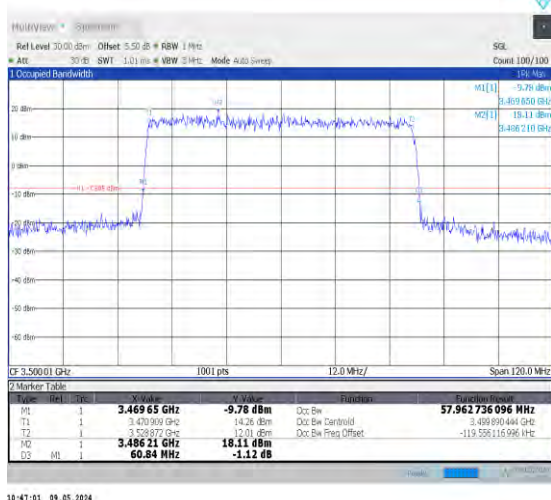
1-N78-3450-3550-PC2-30-60-M-1-DFT-QPSK-Outer_Full-162@0-Ant0-57.963-60.840-≤60-PASS
