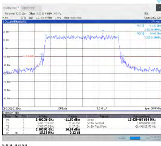
1-N78-3450-3550-PC2-30-15-M-6-CP-QPSK-Outer_Full-38@0-Ant0-13.639-15.330-≤15-PASS
