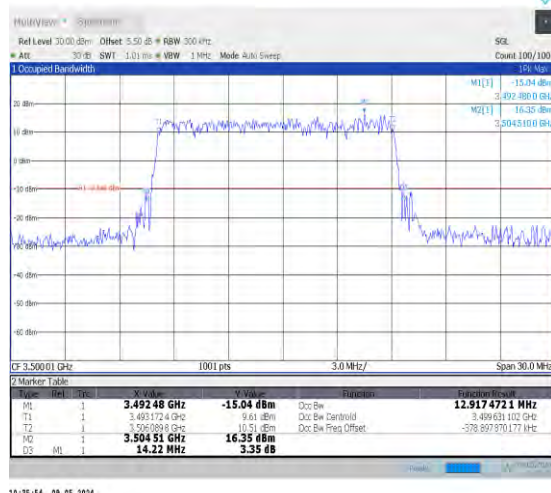
1-N78-3450-3550-PC2-30-15-M-5-DFT-256QAM-Out er_Full-36@0-Ant0-12.917-14.220-≤15-PASS
