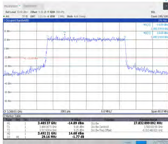
1-N78-3450-3550-PC2-30-30-M-7-CP-16QAM-Out-er_Full-78@0-Ant0-27.815-29.160-≤30-PASS
