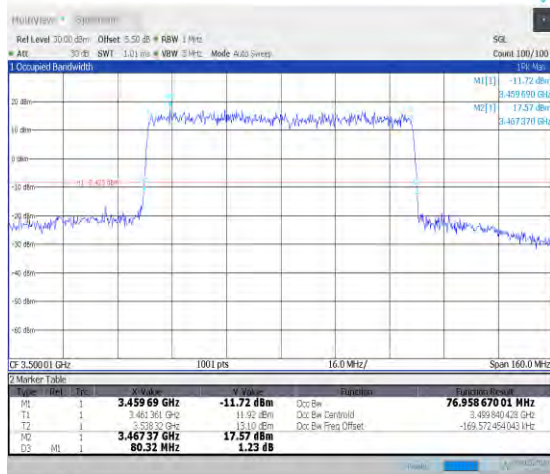
1-N78-3450-3550-PC2-30-80-M-1-DFT-QPSK-Outer_Full-216@0-Ant0-76.959-80.320-≤80-PASS
