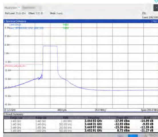
1-N78-3450-3550-PC2-30-20-L-6-CP-QPSK-Outer_Full-51@0-Ant0-1--PASS-see graph
