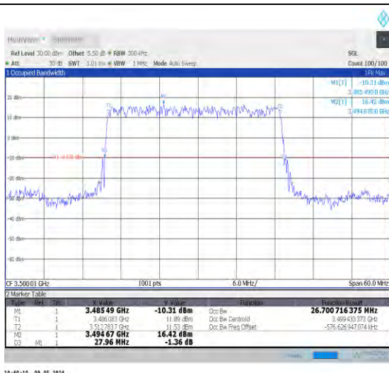
1-N78-3450-3550-PC2-30-30-M-2-DFT-PI2BPSK-Outer_Full-75@0-Ant0-26.7-27.960-≤30-PASS
