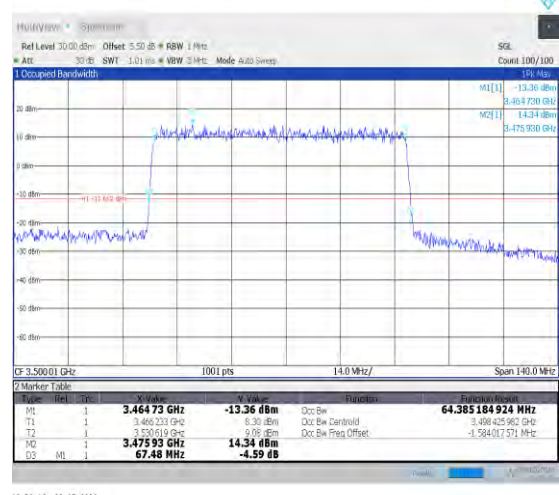
1-N78-3450-3550-PC2-30-70-M-5-DFT-256QAM-Outer_Full-180@0-Ant0-64.385-67.480-≤70-PASS
