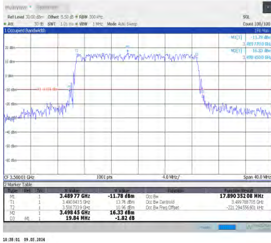
1-N78-3450-3550-PC2-30-20-M-3-DFT-16QAM-Out er_Full-50@0-Ant0-17.89-19.840-≤20-PASS
