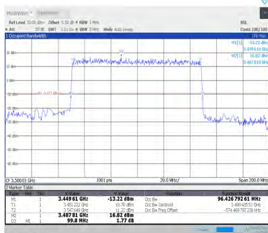
1-N78-3450-3550-PC2-30-100-M-2-DFT-PI2BPSK-Outer_Full-270@0-Ant0-96.427-99.800-≤100-PASS
