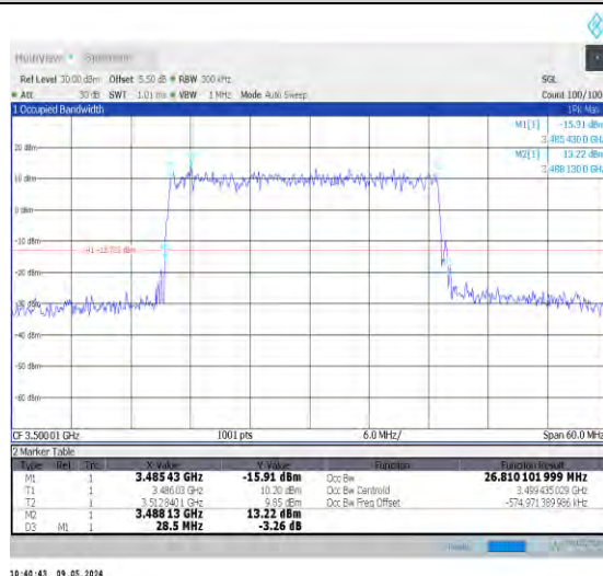
1-N78-3450-3550-PC2-30-30-M-5-DFT-256QAM-Outer_Full-75@0-Ant0-26.812-28.500-≤30-PASS
