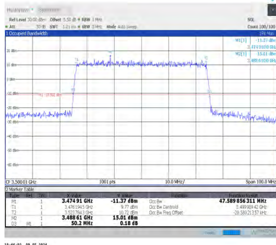
1-N78-3450-3550-PC2-30-50-M-9-CP-256QAM-Outer_Full-133@0-Ant0-47.59-50.200-≤50-PASS
