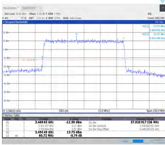
1-N78-3450-3550-PC2-30-60-M-9-CP-256QAM-Outer_Full-162@0-Ant0-57.927-60.720-≤60-PASS
