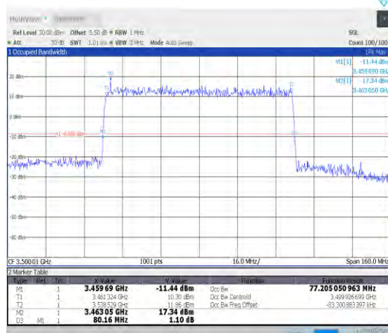
1-N78-3450-3550-PC2-30-80-M-4-DFT-64QAM-Outer_Full-216@0-Ant0-77.205-80.160-≤80-PASS
