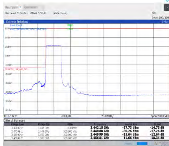
1-N78-3450-3550-PC2-30-20-L-3-DFT-PI2BPSK-Outer_Full-50@0-Ant0-1--PASS-see graph
