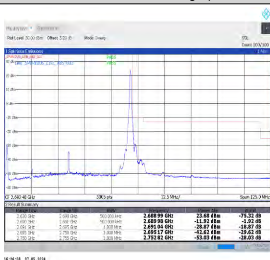
1-N41-30-60-H-5-CP-QPSK-Edge_1RB_Right-1@161-Ant0-1--PASS-see graph
