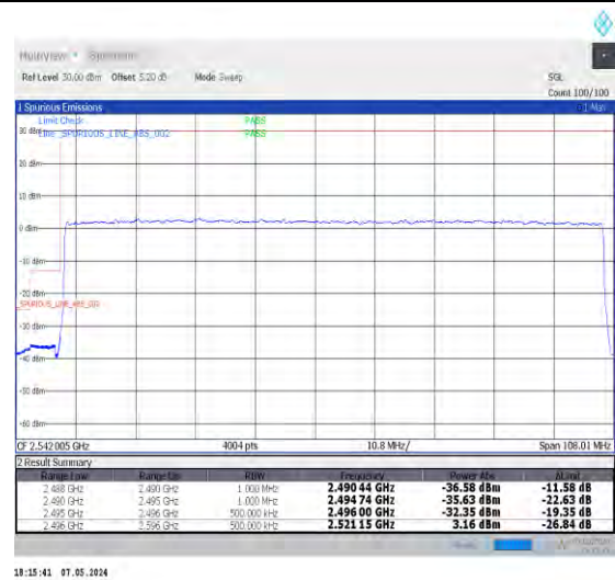
1-N41-30-100-L-3-DFT-PI2BPSK-Outer_Full-270@0-Ant0-1--PASS-see graph
