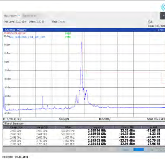
1-N41-30-90-H-2-DFT-PI2BPSK-Edge_1RB_Right-1@244-Ant0-1--PASS-see graph
