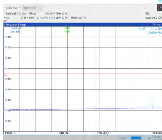
1-N41-30-100-M-1-DFT-PI2BPSK-Inner_1RB_Left-1 @1-0.15-30-Ant0-28.03--77.13--45-PASS
