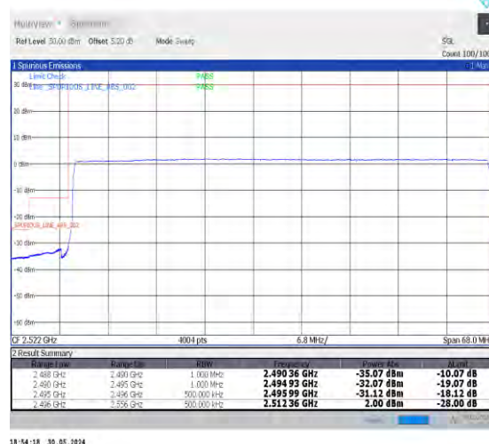
1-N41-30-60-L-6-CP-QPSK-Outer_Full-162@0-Ant0-1--PASS-see graph
