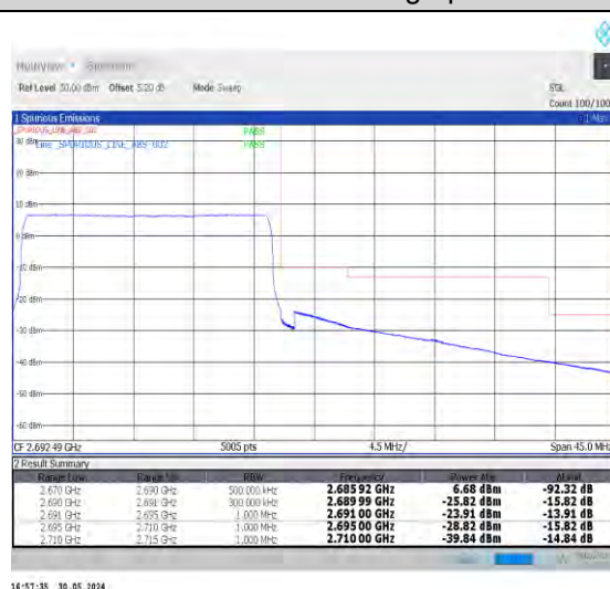
1-N41-30-20-H-6-CP-QPSK-Outer_Full-51@0-Ant0-1--PASS-see graph
