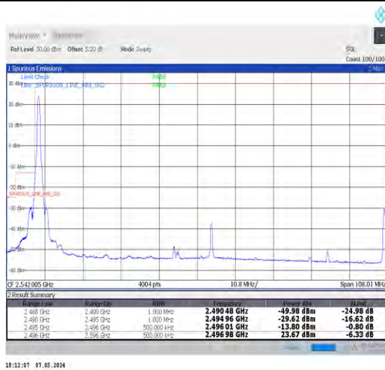
1-N41-30-100-L-1-DFT-PI2BPSK-Edge_1RB_Left-1@0-Ant0-1--PASS-see graph
