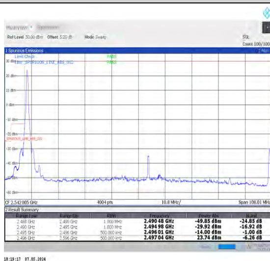
1-N41-30-100-L-4-CP-QPSK-Edge_1RB_Left-1@0-Ant0-1--PASS-see graph
