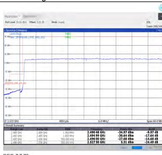
1-N41-30-60-L-3-DFT-PI2BPSK-Outer_Full-162@0-Ant0-1--PASS-see graph
