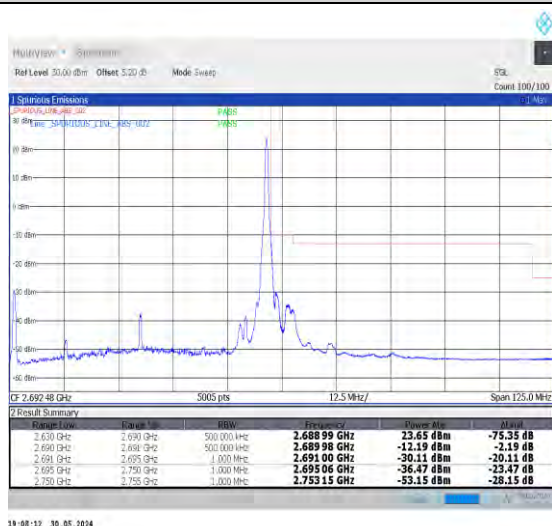
1-N41-30-60-H-5-CP-QPSK-Edge_1RB_Right-1@161-Ant0-1--PASS-see graph
