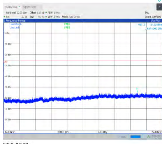
1-N41-30-100-L-1-DFT-PI2BPSK-Inner_1RB_Left-1 @1-12000-27000-Ant0-26238.50--54.85--25-PASS
