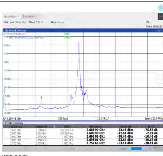
1-N41-30-60-H-2-DFT-PI2BPSK-Edge_1RB_Right-1@161-Ant0-1--PASS-see graph
