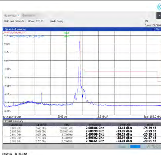
1-N41-30-90-H-5-CP-QPSK-Edge_1RB_Right-1@244-Ant0-1--PASS-see graph
