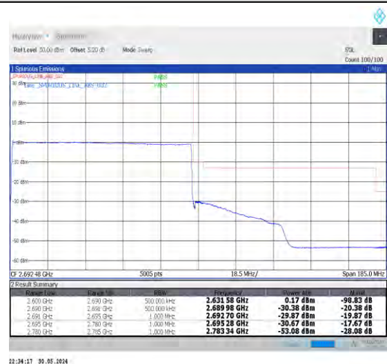
1-N41-30-90-H-6-CP-QPSK-Outer_Full-245@0-Ant0-1--PASS-see graph
