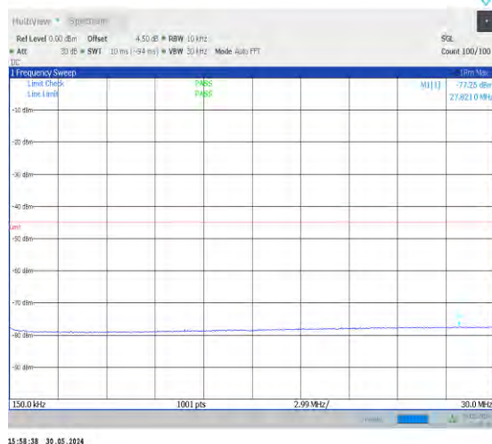
1-N41-30-100-H-1-DFT-PI2BPSK-Inner_1RB_Left-1 @1-0.15-30-Ant0-0.15--77.25--45-PASS
