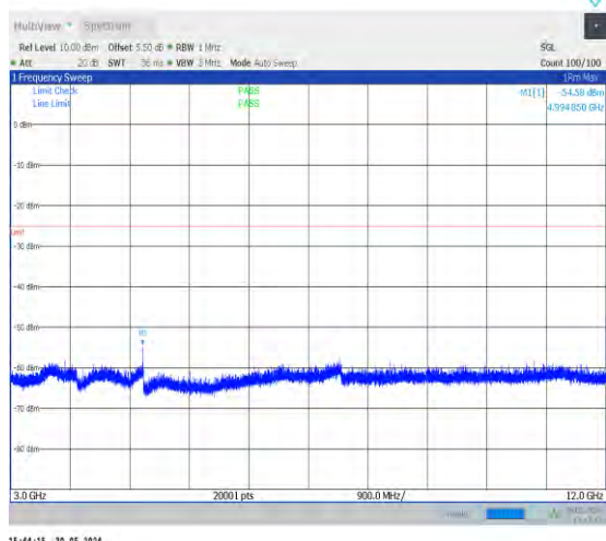
1-N41-30-100-L-1-DFT-PI2BPSK-Inner_1RB_Left-1 @1-3000-12000-Ant0-4994.85--54.58--25-PASS
