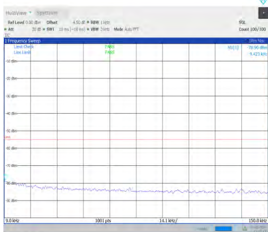
1-N41-30-100-M-1-DFT-PI2BPSK-Inner_1RB_Left-1 @1-0.009-0.15-Ant0-0.01--78.90--55-PASS
