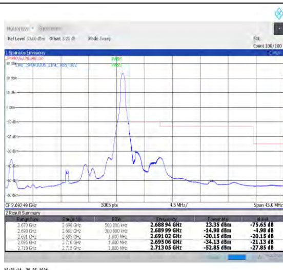
1-N41-30-20-H-2-DFT-PI2BPSK-Edge_1RB_Right-1@50-Ant0-1--PASS-see graph
