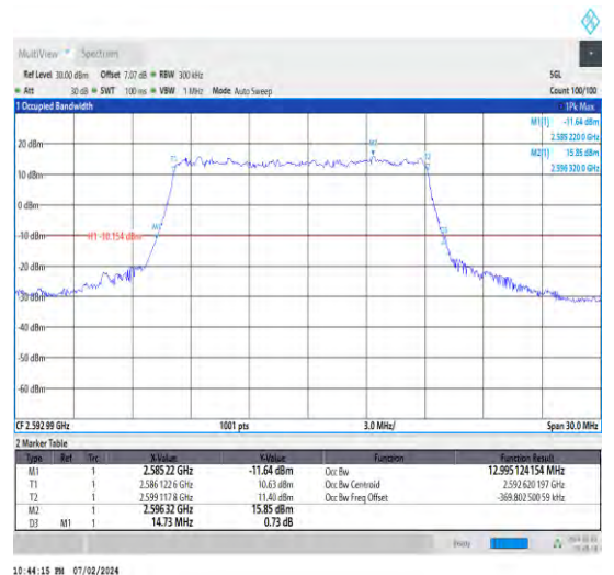
1-N41-30-15-M-3-DFT-16QAM-Outer_Full-36 @0-Ant1-12.995-14.730-≤15-PASS
