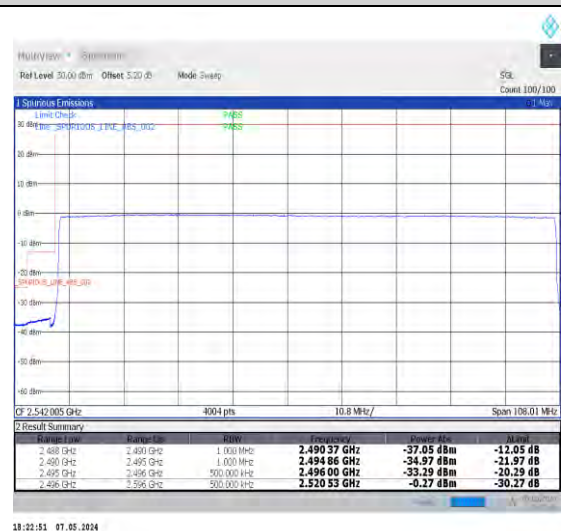
1-N41-30-100-L-6-CP-QPSK-Outer_Full-273@0-Ant0-1--PASS-see graph
