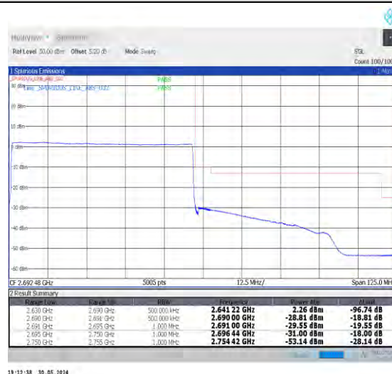
1-N41-30-60-H-6-CP-QPSK-Outer_Full-162@0-Ant0-1--PASS-see graph
