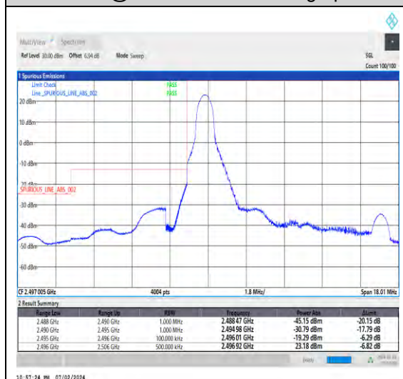
1-N41-30-10-L-4-CP-QPSK-Edge_1RB_Left-1@0-Ant1-1--PASS-see graph
