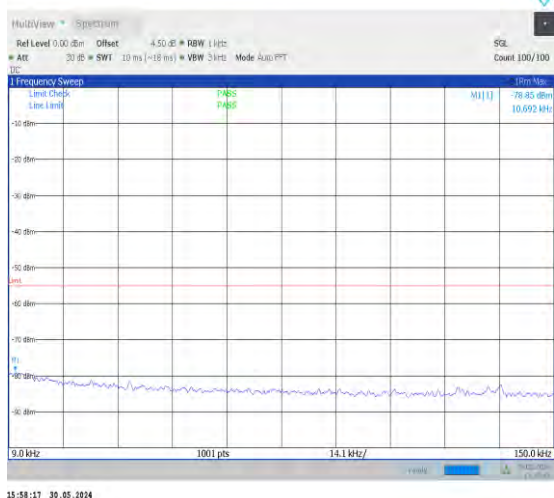
1-N41-30-100-H-1-DFT-PI2BPSK-Inner_1RB_Left-1 @1-0.009-0.15-Ant0-0.01--78.85--55-PASS
