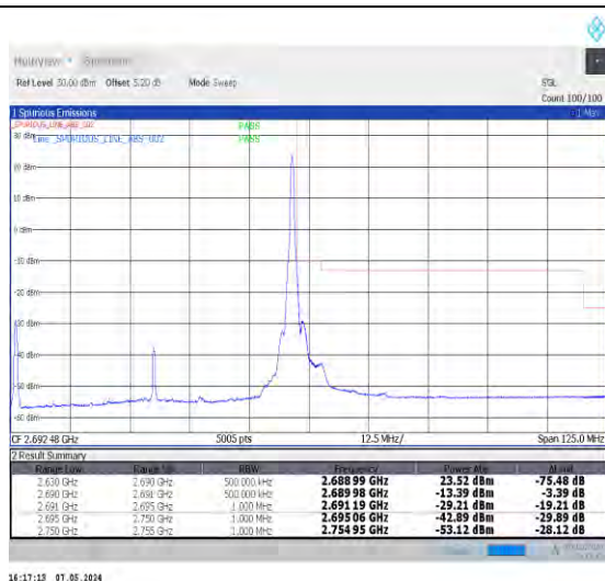
1-N41-30-60-H-2-DFT-PI2BPSK-Edge_1RB_Right-1@161-Ant0-1--PASS-see graph
