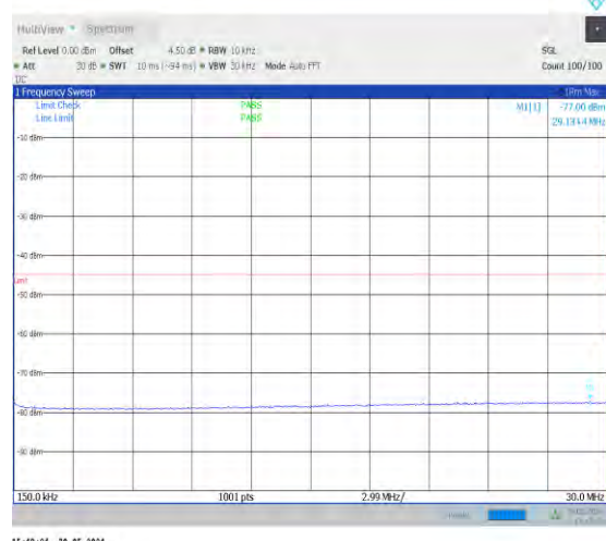
1-N41-30-100-M-1-DFT-PI2BPSK-Inner_1RB_Left-1 @1-0.15-30-Ant0-28.03--77.00--45-PASS
