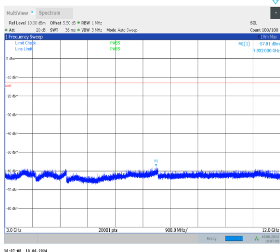
1-N26-814-824-PC3-15-10-M-1-DFT-PI2BPSK-Inner_1RB_Left-1 @ 1-3000-12000-Ant0-7932.00--57.81--13-PASS
