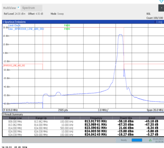
1-N26-814-824-15-10-H-5-CP-QPSK-Edge_1RB_Right-1@51-Ant0-1--PASS-see graph
