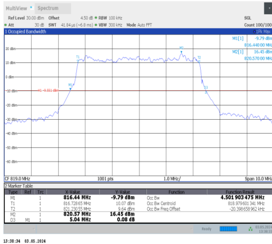
1-N26-814-824-15-5-M-3-DFT-16QAM-Outet_Full-25 @0-Ant0-4.502-5.040-≤5-PASS
