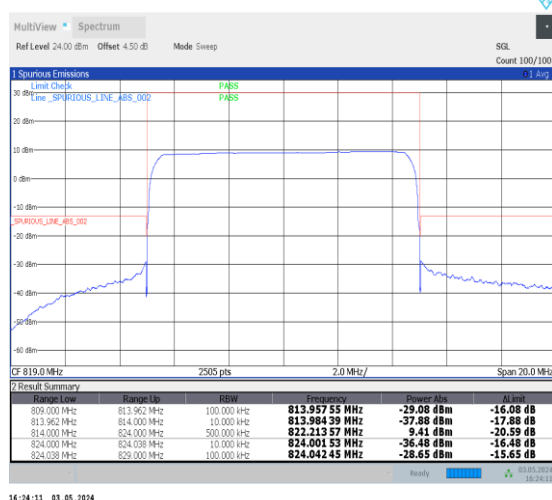
1-N26-814-824-15-10-H-6-CP-QPSK-Outer_Full-52@0-Ant0-1--PASS-see graph
