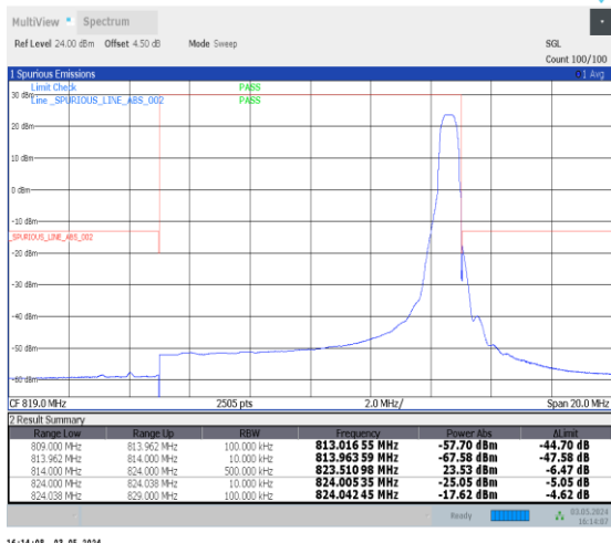
1-N26-814-824-15-10-H-2-DFT-PI2BPSK-Edge_1RB_Right-1@51-Ant0-1--PASS-see graph
