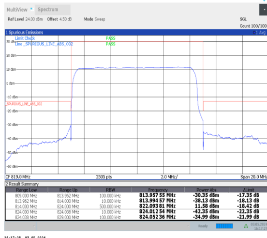
1-N26-814-824-15-10-H-3-DFT-PI2BPSK-Outer_Full-50@0-Ant0-1--PASS-see graph
