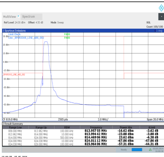
1-N26-814-824-15-10-L-1-DFT-PI2BPSK-Edge_1RB_L eft-1 @0-Ant0-1--PASS-see graph
