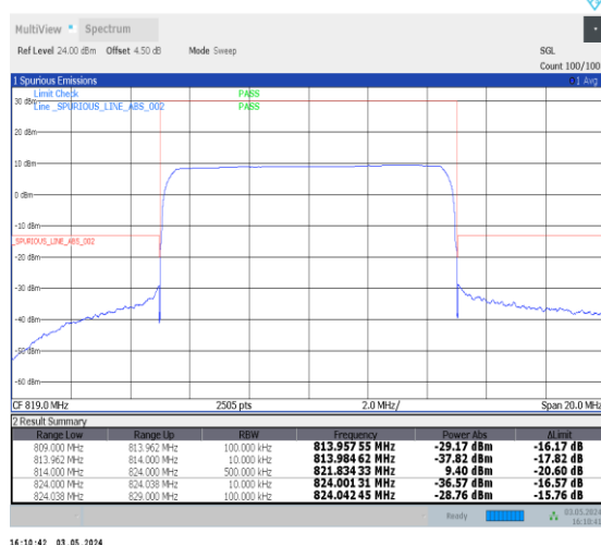
1-N26-814-824-15-10-L-6-CP-QPSK-Outer_Full-5 2 @0-Ant0-1--PASS-see graph
