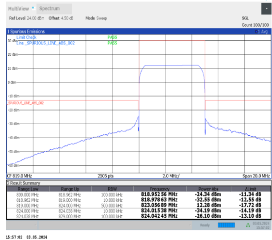
1-N26-814-824-15-5-H-6-CP-QPSK-Outer_Full-25@0-Ant0-1--PASS-see graph
