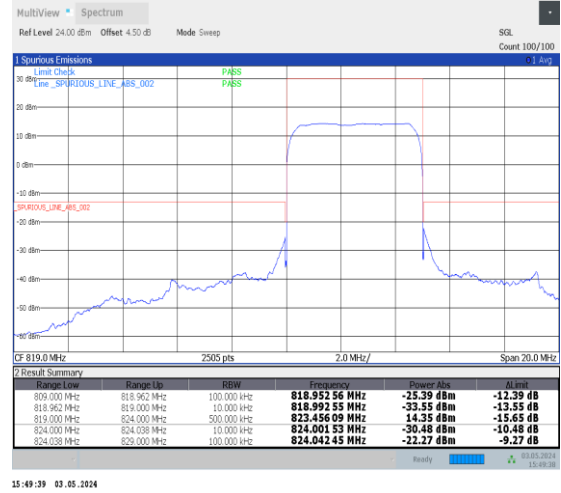
1-N26-814-824-15-5-H-3-DFT-PI2BPSK-Outer_Full-25@0-Ant0-1--PASS-see graph
