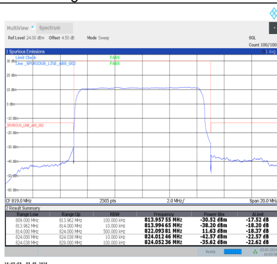
1-N26-814-824-15-10-L-3-DFT-PI2BPSK-Outer_F ull-50 @0-Ant0-1--PASS-see graph
