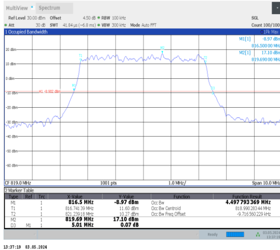
1-N26-814-824-15-5-M-1-DFT-QPSK-Outet_Full-25 @0-Ant0-4.498-5.010-≤5-PASS
