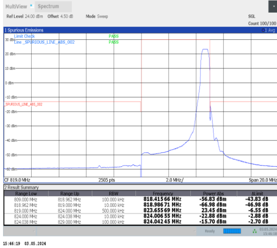
1-N26-814-824-15-5-H-2-DFT-PI2BPSK-Edge_1RB_Right-1@24-Ant0-1--PASS-see graph
