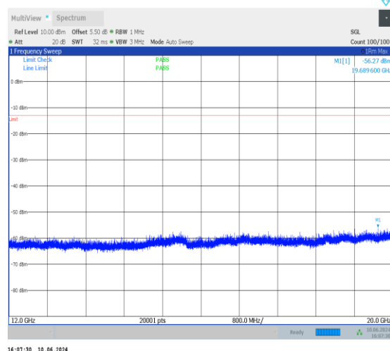
1-N26-814-824-PC3-15-10-M-1-DFT-PI2BPSK-Inner_1RB_Left-1 @ 1-12000-20000-Ant0-19689.60--56.27--13-PASS
