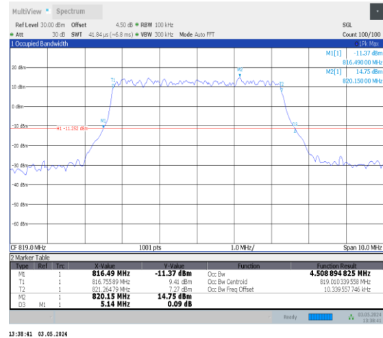
1-N26-814-824-15-5-M-4-DFT-64QAM-Outet_Full-25 @0-Ant0-4.509-5.140-≤5-PASS
