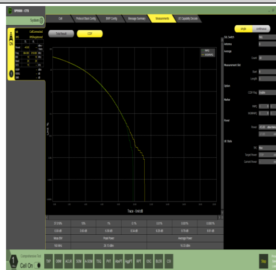
1-N26-814-824-15-10-M-2-CP-256QAM-Outer_Full- 52@0-16.40-16.40-19~27.5-PASS
