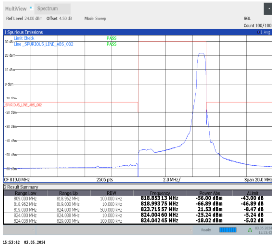
1-N26-814-824-15-5-H-5-CP-QPSK-Edge_1RB_Right-1@24-Ant0-1--PASS-see graph
