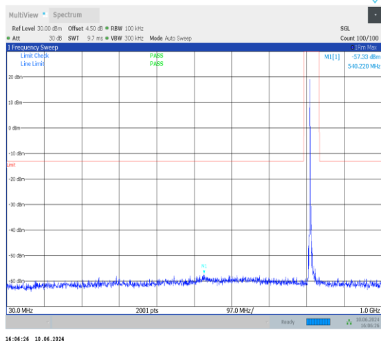
1-N26-814-824-PC3-15-10-M-1-DFT-PI2BPSK-Inner_1RB_Left-1 @ 1-30-1000-Ant0-540.22--57.33--13-P ASS
