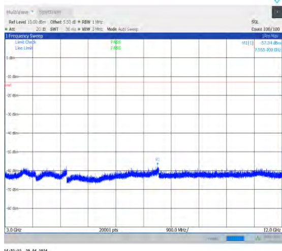
1-N2-15-20-L-1-DFT-PI2BPSK-Inner_1RB_Left-1@ 1-3000-12000-Ant0-3638.55--57.34--13-PASS
