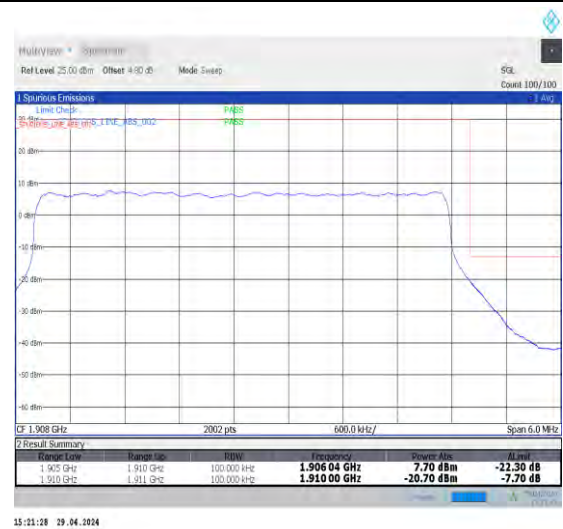
1-N2-15-5-H-3-DFT-PI2BPSK-Outer_Full-25@0-Ant0-1-seegraph-PASS-see graph
