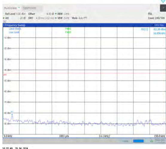
1-N2-15-20-M-1-DFT-PI2BPSK-Inner_1RB_Left-1@ 1-0.009-0.15-Ant0-0.02--82.38--43-PASS
