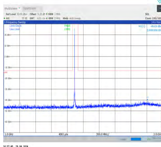
1-N2-15-20-H-1-DFT-PI2BPSK-Inner_1RB_Left-1@ -1000-3000-Ant0-2794.00--40.63--13-PASS
