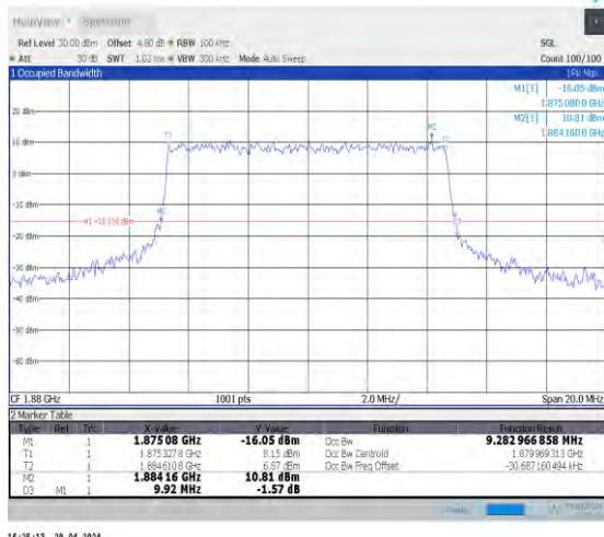
1-N2-15-10-M-8-CP-64QAM-Outer_Full-52@0-Ant0-9.283-9.920-≤10-PASS
