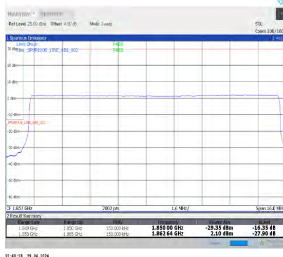
1-N2-15-15-L-6-CP-QPSK-Outer_Full-79@0-Ant0-1-seegraph-PASS-see graph
