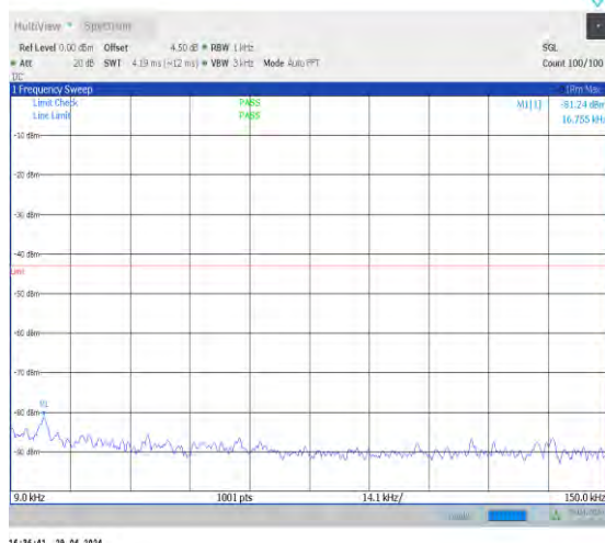
1-N2-15-20-H-1-DFT-PI2BPSK-Inner_1RB_Left-1@ 1-0.009-0.15-Ant0-0.02--81.24--43-PASS
