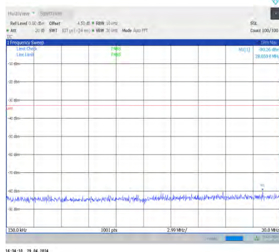
1-N2-15-20-M-1-DFT-PI2BPSK-Inner_1RB_Left-1@1 -0.15-30-Ant0-19.34--80.26--33-PASS
