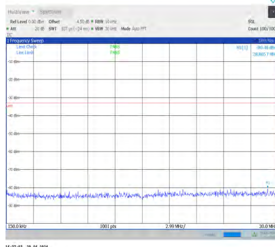
1-N2-15-20-H-1-DFT-PI2BPSK-Inner_1RB_Left-1@ -0.15-30-Ant0-16.33--80.48--33-PASS
