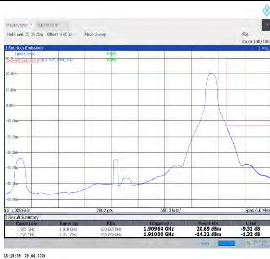
1-N2-15-5-H-2-DFT-PI2BPSK-Edge_1RB_Right-1@24-Ant0-1-seegraph-PASS-see graph
