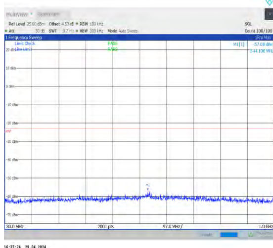
1-N2-15-20-H-1-DFT-PI2BPSK-Inner_1RB_Left-1@ 1-30-1000-Ant0-543.13--57.08--23-PASS
