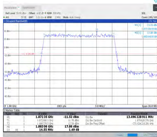
1-N2-15-15-M-2-DFT-PI2BPSK-Outer_Full-75@0-Ant0-13.496-14.550-≤15-PASS
