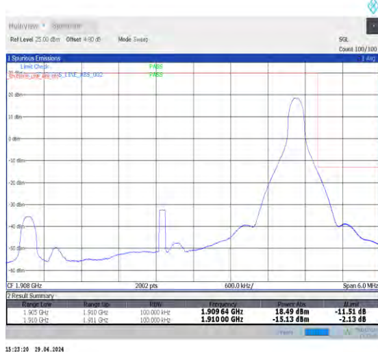
1-N2-15-5-H-5-CP-QPSK-Edge_1RB_Right-1@24-Ant0-1-seegraph-PASS-see graph
