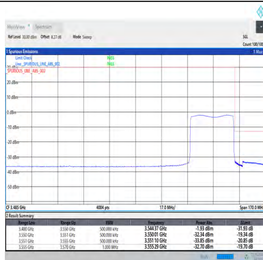
1-N78-3450-3550-30-30-H-6-CP-QPSK-Outer_Full-78@0-Ant0-1--PASS-see graph
