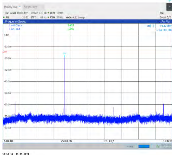
1-N78-3450-3550-PC2-30-100-L-1-DFT-PI2BPSK-In ner_1RB_Left-1@1-6000-18000-Ant0-10354.08--19. 12--13-PASS
