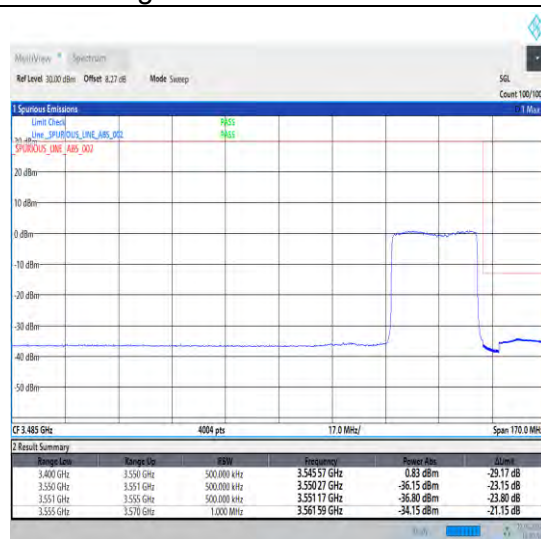
1-N78-3450-3550-30-30-H-3-DFT-PI2BPSK-Outer_Full-75@0-Ant0-1--PASS-see graph
