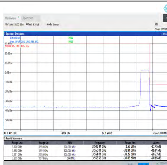
1-N78-3450-3550-30-10-H-6-CP-QPSK-Outer_Full-24@0-Ant0-1--PASS-see graph
