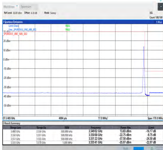
1-N78-3450-3550-30-60-H-2-DFT-PI2BPSK-Edge_1R B_Right-1@161-Ant0-1--PASS-see graph
