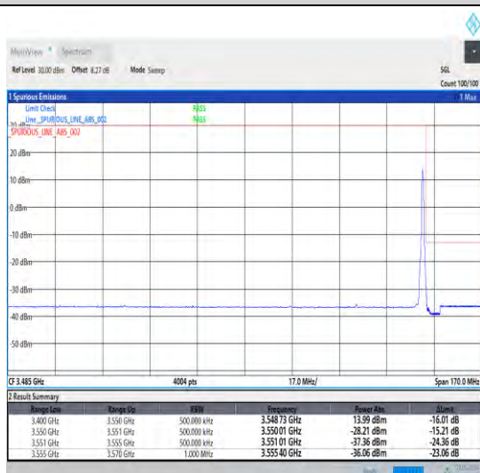
1-N78-3450-3550-30-50-H-5-CP-QPSK-Edge_1RB_Ri ght-1@132-Ant0-1--PASS-see graph
