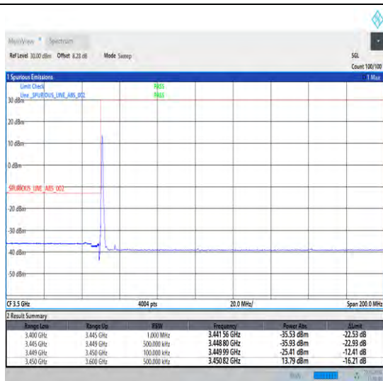
1-N78-3450-3550-30-15-L-1-DFT-PI2BPSK-Edge_1RB _Left-1@0-Ant0-1--PASS-see graph
