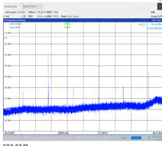
1-N78-3450-3550-PC2-30-100-L-1-DFT-PI2BPSK-In ner_1RB_Left-1@1-18000-40000-Ant0-24160.49--34. .49--13-PASS
