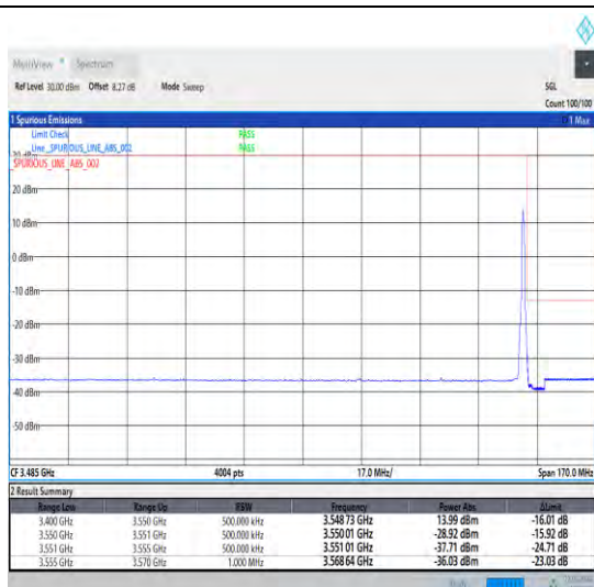
1-N78-3450-3550-30-50-H-2-DFT-PI2BPSK-Edge_1R B_Right-1@132-Ant0-1--PASS-see graph
