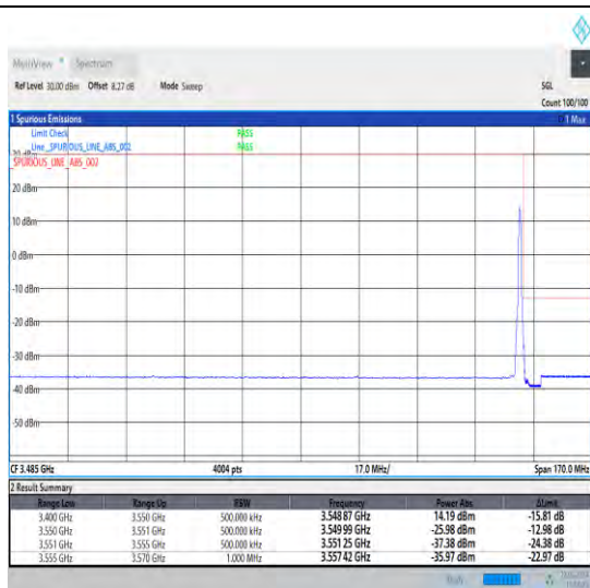
1-N78-3450-3550-30-30-H-2-DFT-PI2BPSK-Edge_1R_B_Right-1@77-Ant0-1--PASS-see graph
