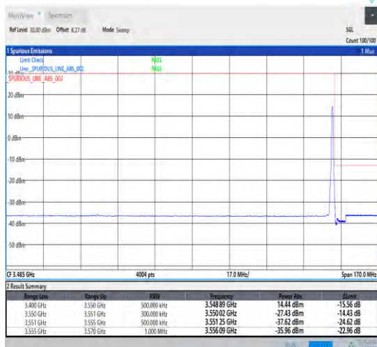
1-N78-3450-3550-30-40-H-2-DFT-PI2BPSK-Edge_1R B_Right-1@105-Ant0-1--PASS-see graph
