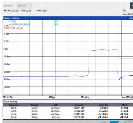
1-N78-3450-3550-30-40-H-3-DFT-PI2BPSK-Outer _Full-100@0-Ant0-1--PASS-see graph
