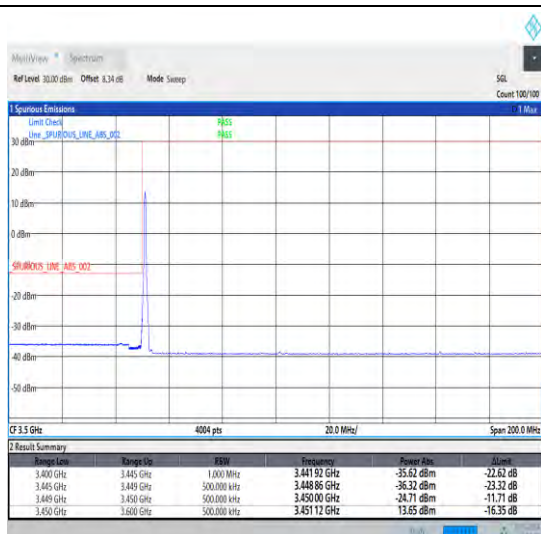
1-N78-3450-3550-30-90-L-1-DFT-PI2BPSK-Edge_1RB _Left-1@0-Ant0-1--PASS-see graph
