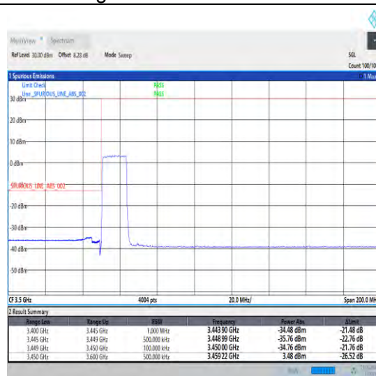
1-N78-3450-3550-30-15-L-3-DFT-PI2BPSK-Outer _Full-36@0-Ant0-1--PASS-see graph
