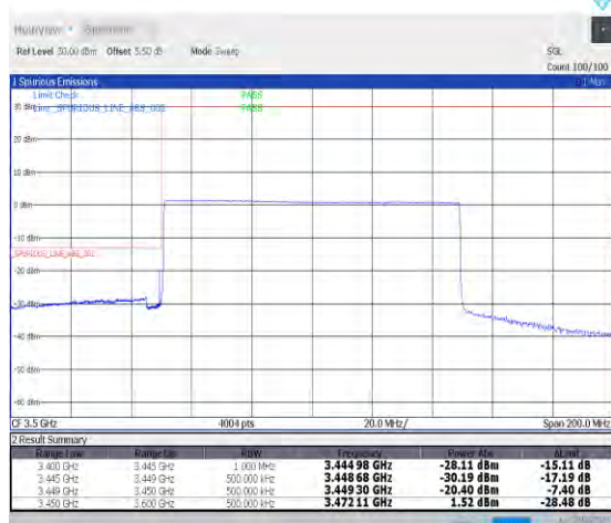
1-N78-3450-3550-PC2-30-100-L-6-CP-QPSK-Outer_Full-273@0-Ant0-1--PASS-see graph
