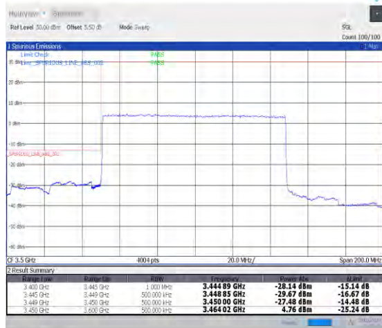
1-N78-3450-3550-PC2-30-100-L-3-DFT-PI2BPSK-Outer_Full-270@0-Ant0-1--PASS-see graph
