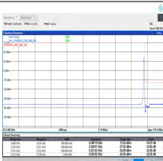
1-N78-3450-3550-30-10-H-5-CP-QPSK-Edge_1RB_Right-1@23-Ant0-1--PASS-see graph
