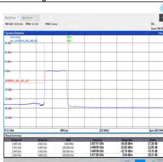
1-N78-3450-3550-30-30-L-3-DFT-PI2BPSK-Outer_Full-75@0-Ant0-1--PASS-see graph
