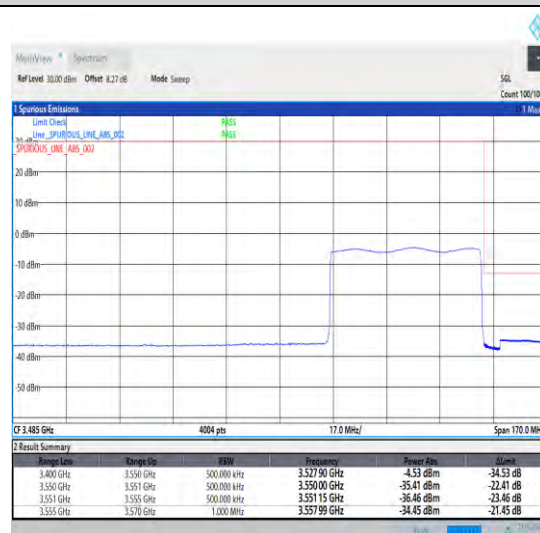
1-N78-3450-3550-30-50-H-6-CP-QPSK-Outer_Full -133@0-Ant0-1--PASS-see graph
