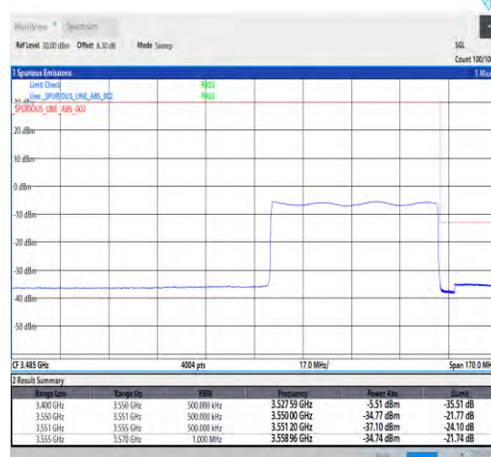
1-N78-3450-3550-30-60-H-6-CP-QPSK-Outer_Full -162@0-Ant0-1--PASS-see graph
