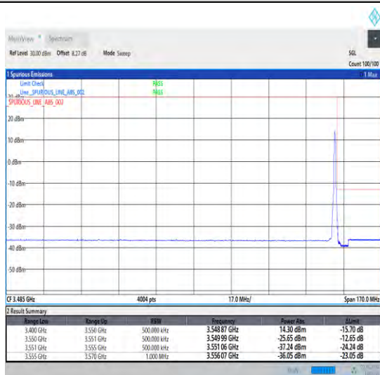
1-N78-3450-3550-30-30-H-5-CP-QPSK-Edge_1RB_Right-1@77-Ant0-1--PASS-see graph
