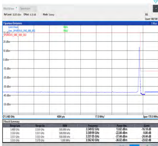
1-N78-3450-3550-30-60-H-5-CP-QPSK-Edge_1RB_Ri ght-1@161-Ant0-1--PASS-see graph
