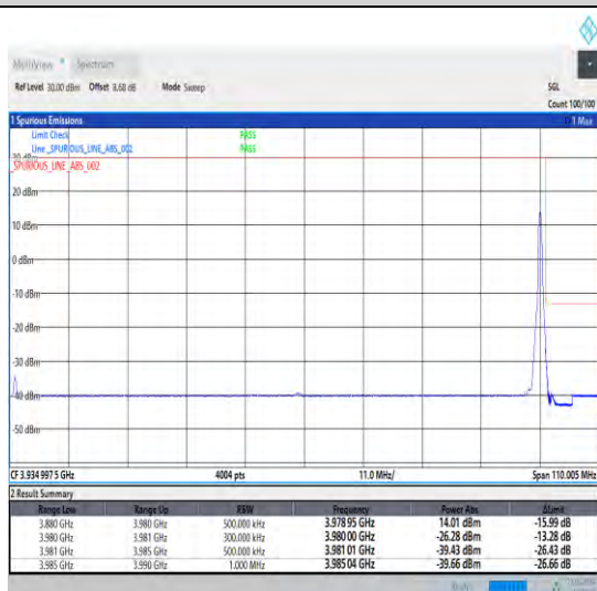
1-N77-3700-3980-30-100-H-5-CP-QPSK-Edge_1RB_Right-1@272-Ant0-1--PASS-see graph
