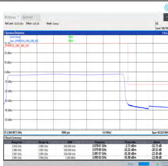
1-N77-3700-3980-30-30-H-6-CP-QPSK-Outer_Full-78@0-Ant0-1--PASS-see graph
