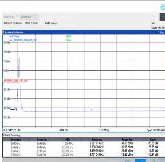
1-N77-3700-3980-30-100-L-4-CP-QPSK-Edge_1RB_Left-1@0-Ant0-1--PASS-see graph
