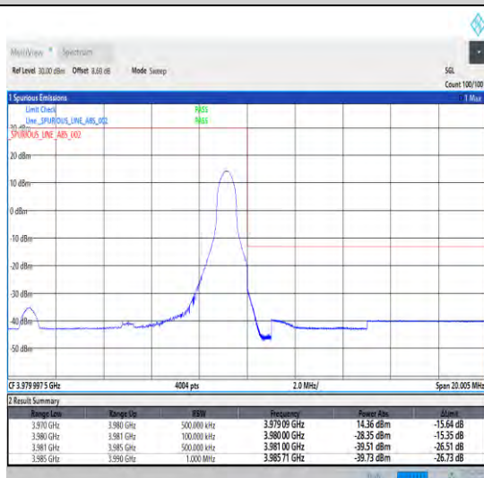
1-N77-3700-3980-30-10-H-5-CP-QPSK-Edge_1RB_Right-1@23-Ant0-1--PASS-see graph
