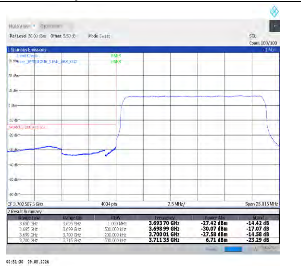
1-N77-3700-3980-PC2-30-15-L-3-DFT-PI2BPSK-Outer_Full-36@0-Ant0-1--PASS-see graph
