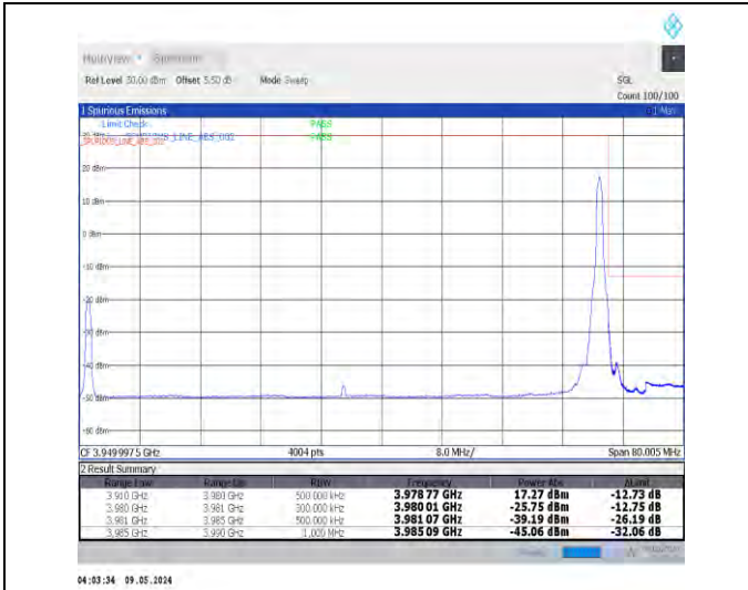
1-N77-3700-3980-PC2-30-70-H-2-DFT-PI2BPSK-Edge_1RB_Right-1@188-Ant0-1--PASS-see graph
