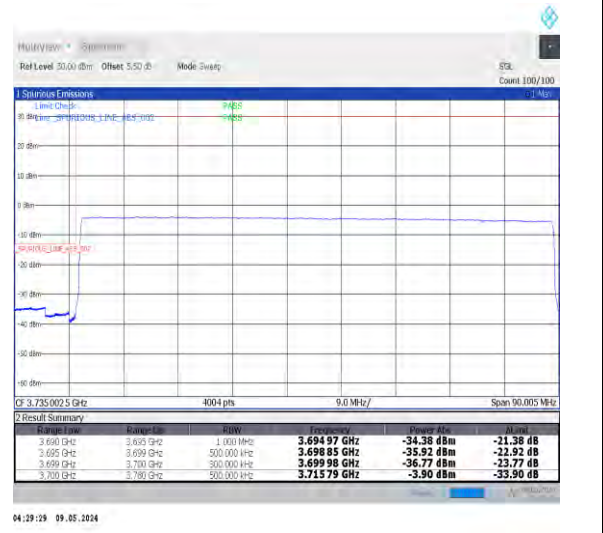
1-N77-3700-3980-PC2-30-80-L-6-CP-QPSK-Outer_Full-217@0-Ant0-1--PASS-see graph
