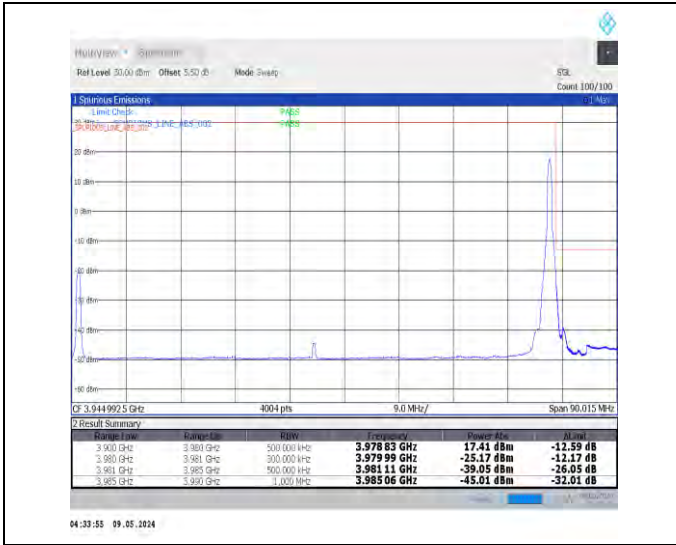
1-N77-3700-3980-PC2-30-80-H-2-DFT-PI2BPSK-Edge_1RB_Right-1@216-Ant0-1--PASS-see graph
