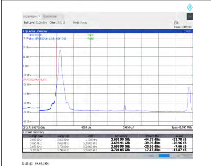
1-N77-3700-3980-PC2-30-40-L-4-CP-QPSK-Edge_1RB_Left-1@0-Ant0-1--PASS-see graph
