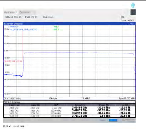
1-N77-3700-3980-PC2-30-60-L-6-CP-QPSK-Outer_Full-162@0-Ant0-1--PASS-see graph
