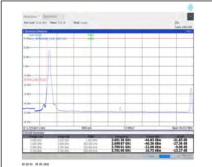
1-N77-3700-3980-PC2-30-60-L-1-DFT-PI2BPSK-Edge_1RB_Left-1@0-Ant0-1--PASS-see graph
