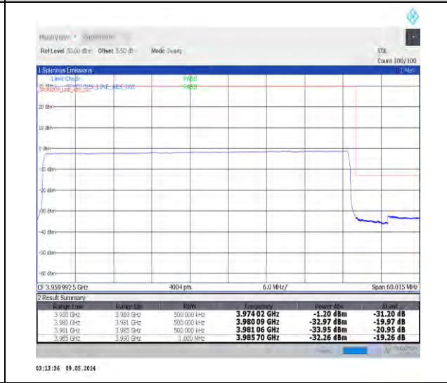
1-N77-3700-3980-PC2-30-50-H-6-CP-QPSK-Outer_Full-133@0-Ant0-1--PASS-see graph
