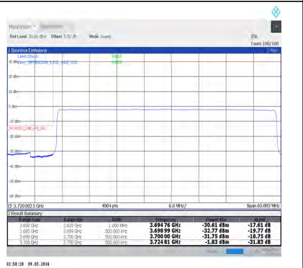
1-N77-3700-3980-PC2-30-50-L-6-CP-QPSK-Outer_Full-133@0-Ant0-1--PASS-see graph
