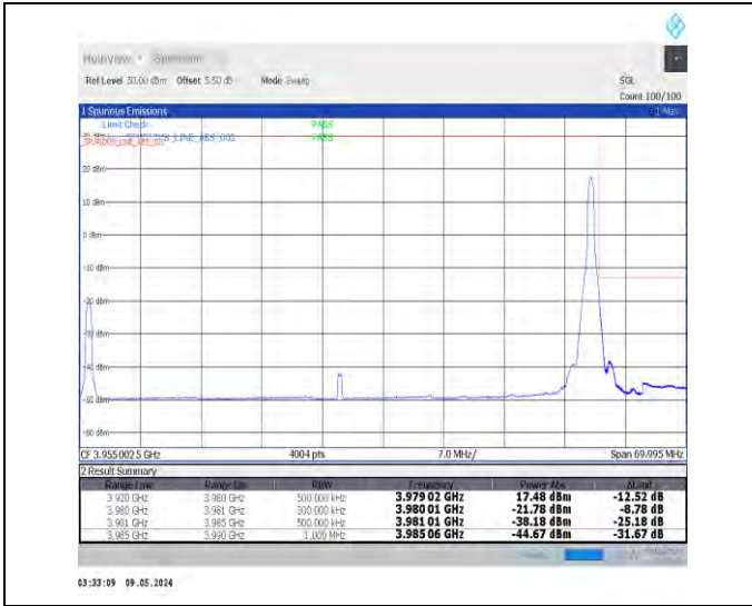
1-N77-3700-3980-PC2-30-60-H-2-DFT-PI2BPSK-Edge_1RB_Right-1@161-Ant0-1--PASS-see graph
