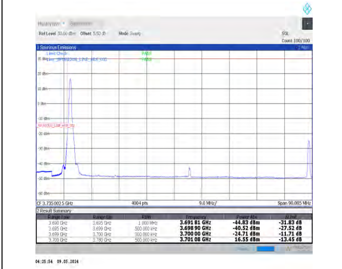
1-N77-3700-3980-PC2-30-80-L-4-CP-QPSK-Edge_1RB_Left-1@0-Ant0-1--PASS-see graph
