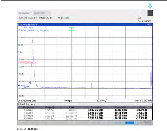
1-N77-3700-3980-PC2-30-90-L-4-CP-QPSK-Edge_1RB_Left-1@0-Ant0-1--PASS-see graph
