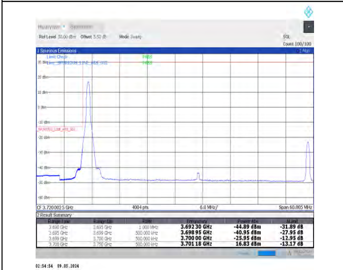
1-N77-3700-3980-PC2-30-50-L-4-CP-QPSK-Edge_1RB_Left-1@0-Ant0-1--PASS-see graph
