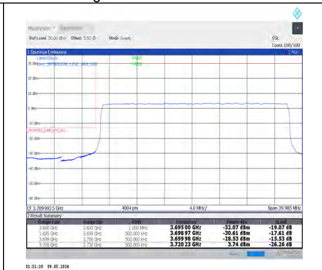
1-N77-3700-3980-PC2-30-30-L-3-DFT-PI2BPSK-Outer_Full-75@0-Ant0-1--PASS-see graph
