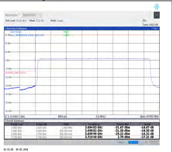
1-N77-3700-3980-PC2-30-40-L-3-DFT-PI2BPSK-Outer_Full-100@0-Ant0-1--PASS-see graph
