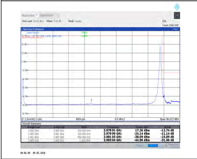
1-N77-3700-3980-PC2-30-80-H-5-CP-QPSK-Edge_1RB_Right-1@216-Ant0-1--PASS-see graph
