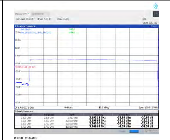
1-N77-3700-3980-PC2-30-90-L-6-CP-QPSK-Outer_Full-245@0-Ant0-1--PASS-see graph
