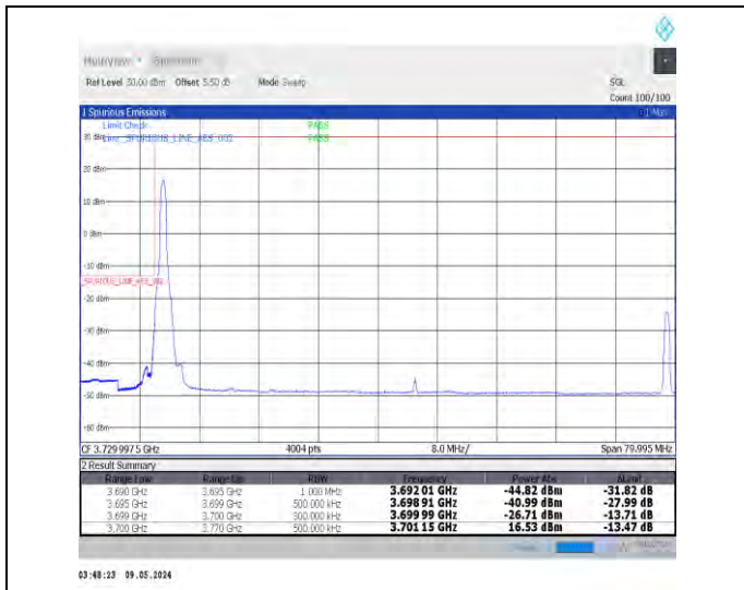
1-N77-3700-3980-PC2-30-70-L-1-DFT-PI2BPSK-Edge_1RB_Left-1@0-Ant0-1--PASS-see graph
