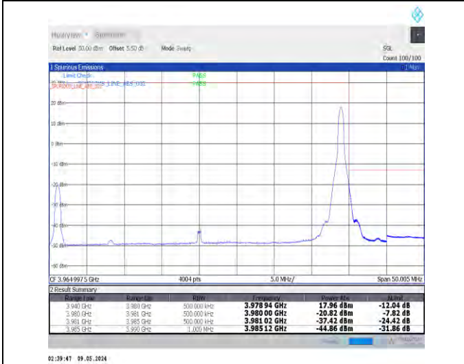
1-N77-3700-3980-PC2-30-40-H-5-CP-QPSK-Edge_1RB_Right-1@105-Ant0-1--PASS-see graph
