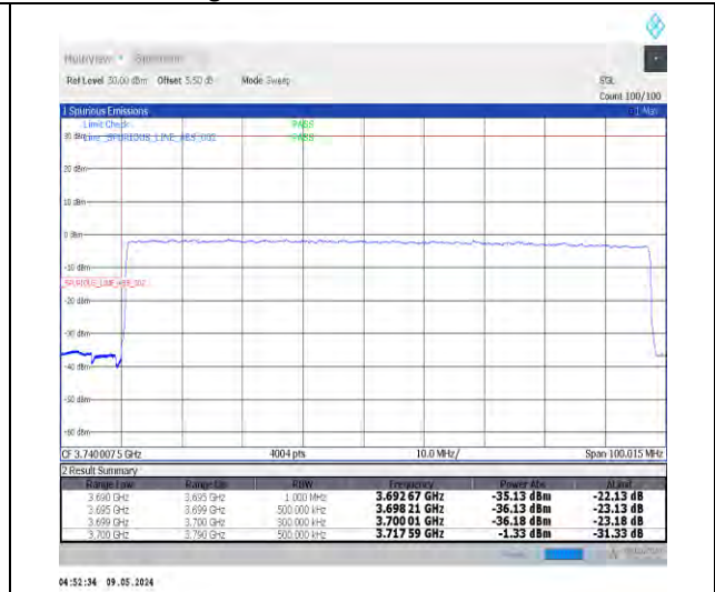
1-N77-3700-3980-PC2-30-90-L-3-DFT-PI2BPSK-Outer_Full-240@0-Ant0-1--PASS-see graph
