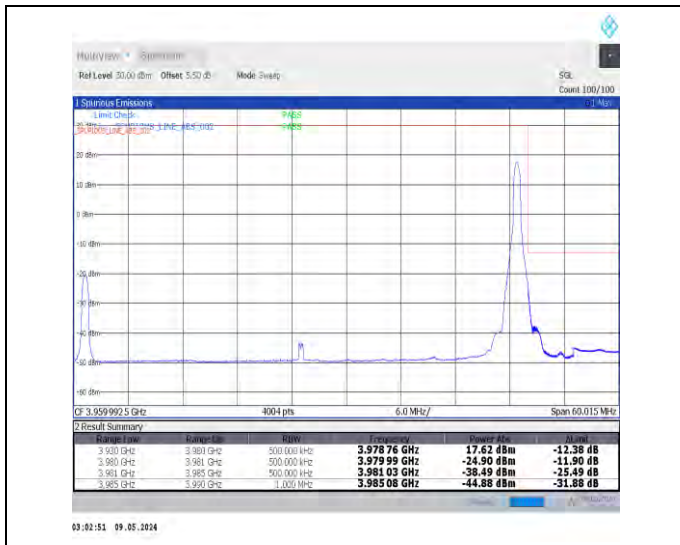
1-N77-3700-3980-PC2-30-50-H-2-DFT-PI2BPSK-Edge_1RB_Right-1@132-Ant0-1--PASS-see graph
