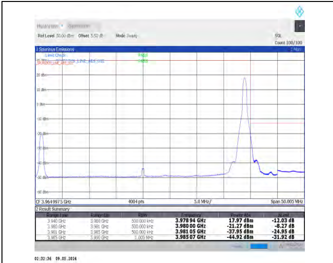
1-N77-3700-3980-PC2-30-40-H-2-DFT-PI2BPSK-Edge_1RB_Right-1@105-Ant0-1--PASS-see graph
