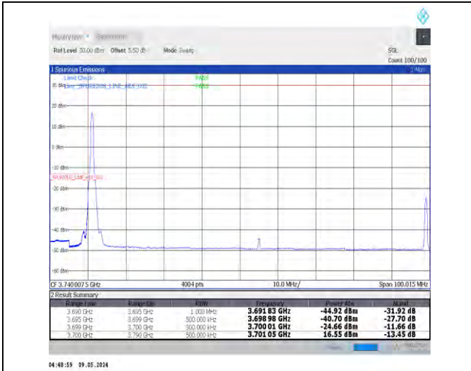
1-N77-3700-3980-PC2-30-90-L-1-DFT-PI2BPSK-Edge_1RB_Left-1@0-Ant0-1--PASS-see graph
