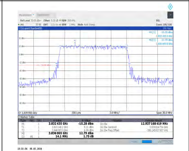
1-N77-3700-3980-PC2-30-15-M-3-DFT-16QAM-Outer _Full-36@0-Ant0-12.937-14.100-≤15-PASS
