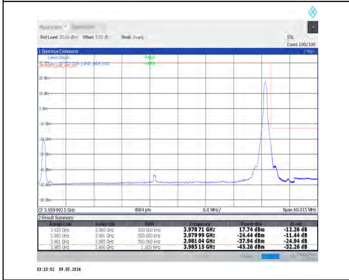
1-N77-3700-3980-PC2-30-50-H-5-CP-QPSK-Edge_1RB_Right-1@132-Ant0-1--PASS-see graph
