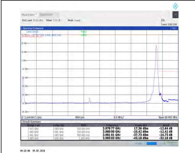
1-N77-3700-3980-PC2-30-70-H-5-CP-QPSK-Edge_1RB_Right-1@188-Ant0-1--PASS-see graph
