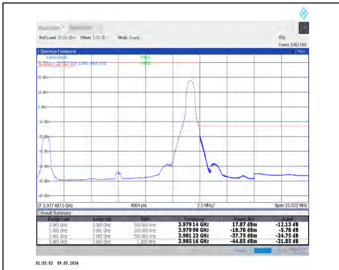
1-N77-3700-3980-PC2-30-15-H-2-DFT-PI2BPSK-Edge_1RB_Right-1@37-Ant0-1--PASS-see graph
