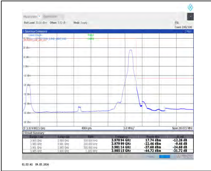
1-N77-3700-3980-PC2-30-20-H-2-DFT-PI2BPSK-Edge_1RB_Right-1@50-Ant0-1--PASS-see graph
