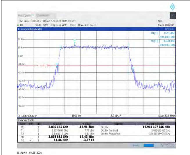
1-N77-3700-3980-PC2-30-15-M-2-DFT-PI2BPSK-Outer _Full-36@0-Ant0-12.941-14.460-≤15-PASS
