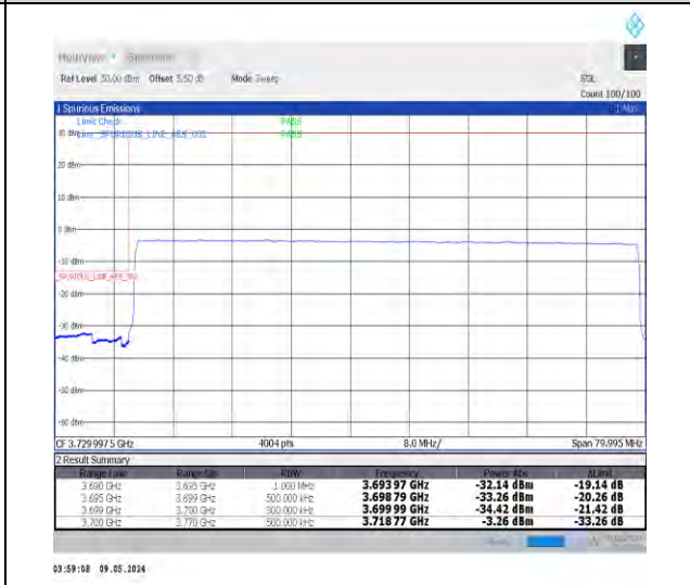
1-N77-3700-3980-PC2-30-70-L-6-CP-QPSK-Outer_Full-189@0-Ant0-1--PASS-see graph
