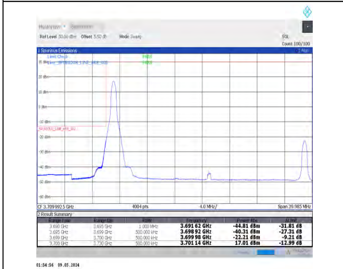
1-N77-3700-3980-PC2-30-30-L-4-CP-QPSK-Edge_1RB_Left-1@0-Ant0-1--PASS-see graph
