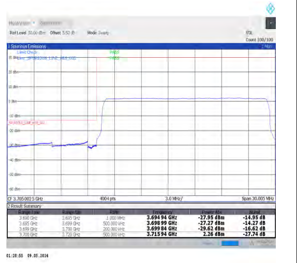
1-N77-3700-3980-PC2-30-20-L-6-CP-QPSK-Outer_Full-51@0-Ant0-1--PASS-see graph
