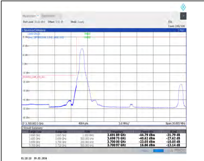
1-N77-3700-3980-PC2-30-20-L-1-DFT-PI2BPSK-Edge_1RB_Left-1@0-Ant0-1--PASS-see graph
