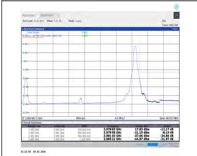
1-N77-3700-3980-PC2-30-30-H-5-CP-QPSK-Edge_1RB_Right-1@77-Ant0-1--PASS-see graph
