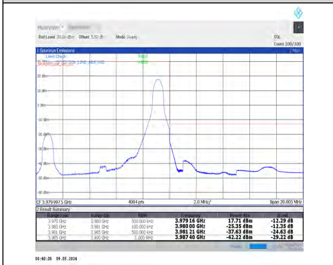
1-N77-3700-3980-PC2-30-10-H-5-CP-QPSK-Edge_1R_B_Right-1@23-Ant0-1--PASS-see graph
