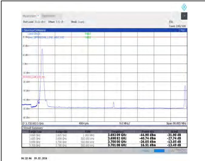
1-N77-3700-3980-PC2-30-80-L-1-DFT-PI2BPSK-Edge_1RB_Left-1@0-Ant0-1--PASS-see graph
