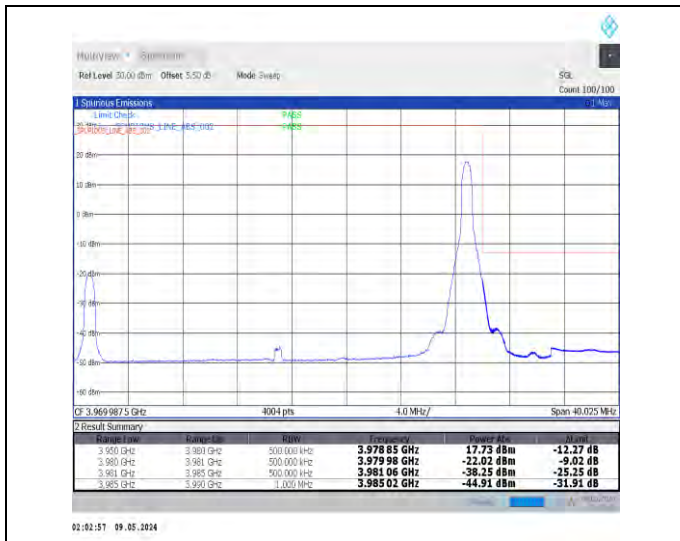
1-N77-3700-3980-PC2-30-30-H-2-DFT-PI2BPSK-Edge_1RB_Right-1@77-Ant0-1--PASS-see graph
