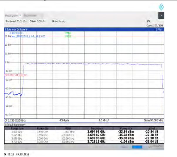
1-N77-3700-3980-PC2-30-80-L-3-DFT-PI2BPSK-Outer_Full-216@0-Ant0-1--PASS-see graph
