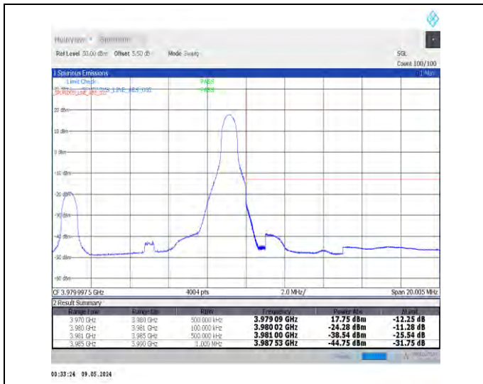
1-N77-3700-3980-PC2-30-10-H-2-DFT-PI2BPSK-Edge_1RB_Right-1@23-Ant0-1--PASS-see graph
