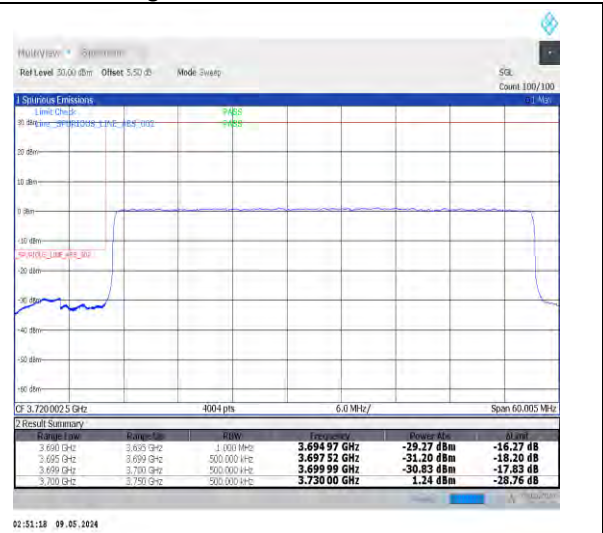
1-N77-3700-3980-PC2-30-50-L-3-DFT-PI2BPSK-Outer_Full-128@0-Ant0-1--PASS-see graph
