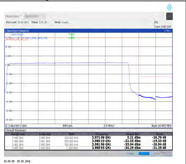
1-N77-3700-3980-PC2-30-40-H-3-DFT-PI2BPSK-Outer_Full-100@0-Ant0-1--PASS-see graph
