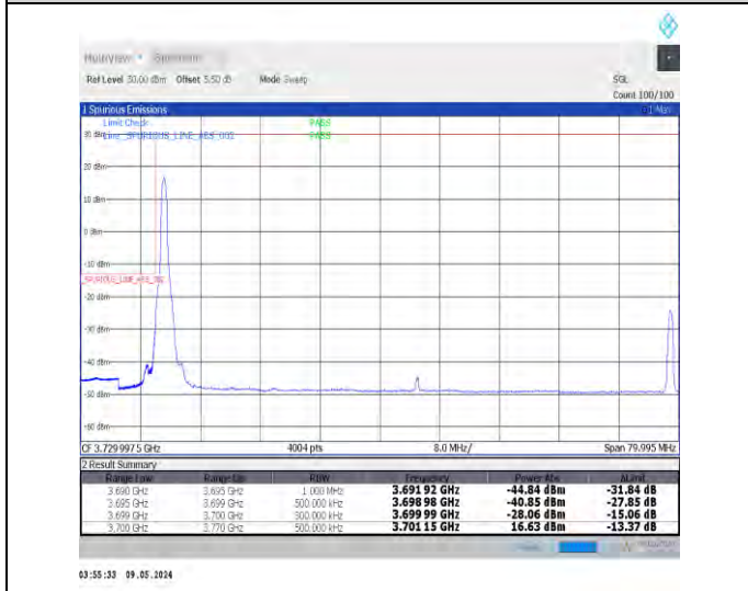
1-N77-3700-3980-PC2-30-70-L-4-CP-QPSK-Edge_1RB_Left-1@0-Ant0-1--PASS-see graph
