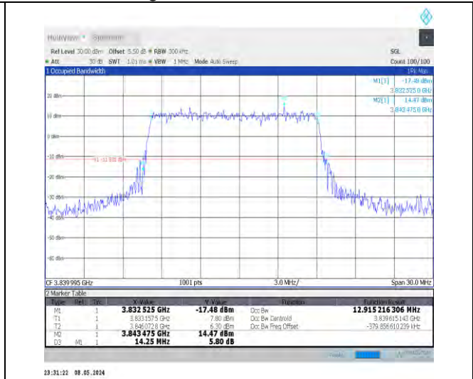
1-N77-3700-3980-PC2-30-15-M-1-DFT-QPSK-Outer _Full-36@0-Ant0-12.915-14.250-≤15-PASS
