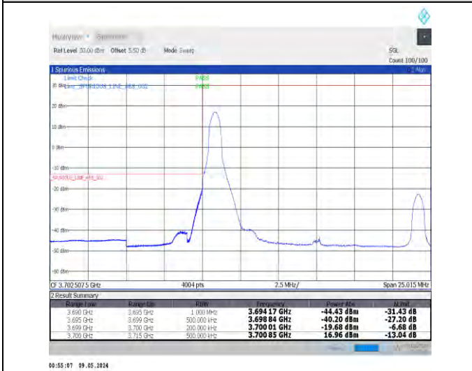
1-N77-3700-3980-PC2-30-15-L-4-CP-QPSK-Edge_1RB_Left-1@0-Ant0-1--PASS-see graph
