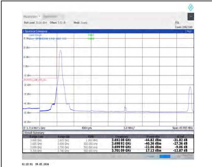
1-N77-3700-3980-PC2-30-40-L-1-DFT-PI2BPSK-Edge_1RB_Left-1@0-Ant0-1--PASS-see graph
