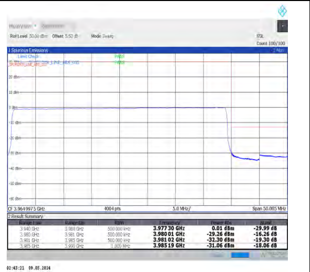
1-N77-3700-3980-PC2-30-40-H-6-CP-QPSK-Outer_Full-106@0-Ant0-1--PASS-see graph
