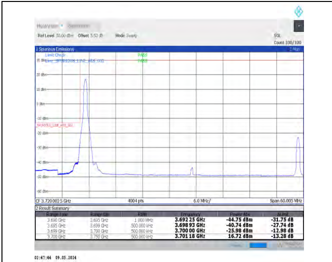
1-N77-3700-3980-PC2-30-50-L-1-DFT-PI2BPSK-Edge_1RB_Left-1@0-Ant0-1--PASS-see graph
