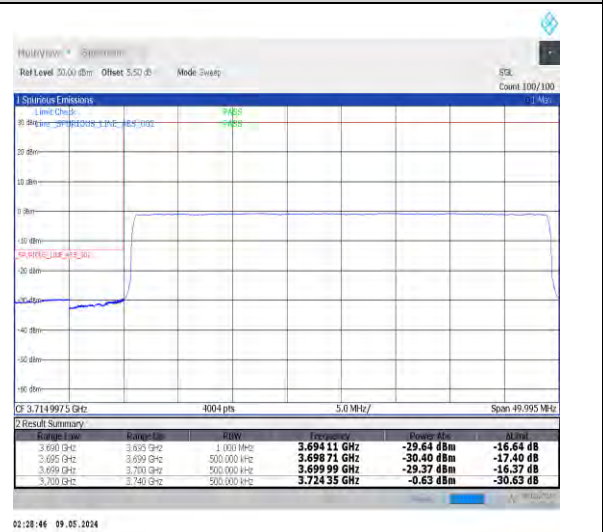
1-N77-3700-3980-PC2-30-40-L-6-CP-QPSK-Outer_Full-106@0-Ant0-1--PASS-see graph
