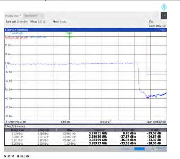
1-N77-3700-3980-PC2-30-70-H-3-DFT-PI2BPSK-Outer_Full-180@0-Ant0-1--PASS-see graph
