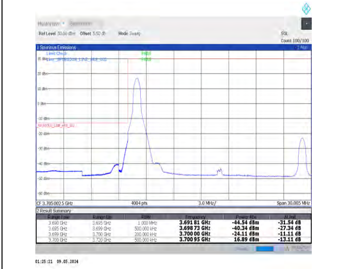
1-N77-3700-3980-PC2-30-20-L-4-CP-QPSK-Edge_1RB_Left-1@0-Ant0-1--PASS-see graph
