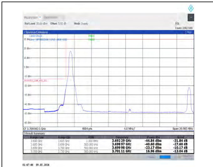
1-N77-3700-3980-PC2-30-30-L-1-DFT-PI2BPSK-Edge_1RB_Left-1@0-Ant0-1--PASS-see graph
