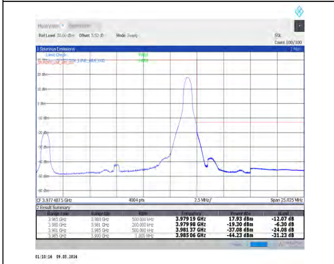
1-N77-3700-3980-PC2-30-15-H-5-CP-QPSK-Edge_1R_B_Right-1@37-Ant0-1--PASS-see graph
