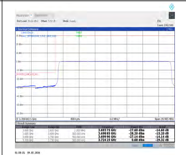
1-N77-3700-3980-PC2-30-30-L-6-CP-QPSK-Outer_Full-78@0-Ant0-1--PASS-see graph
