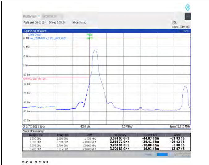
1-N77-3700-3980-PC2-30-15-L-1-DFT-PI2BPSK-Edge_1RB_Left-1@0-Ant0-1--PASS-see graph
