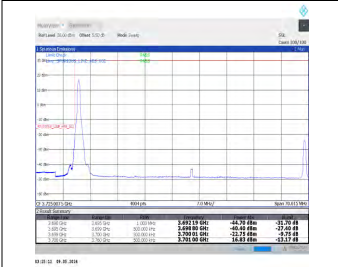
1-N77-3700-3980-PC2-30-60-L-4-CP-QPSK-Edge_1RB_Left-1@0-Ant0-1--PASS-see graph
