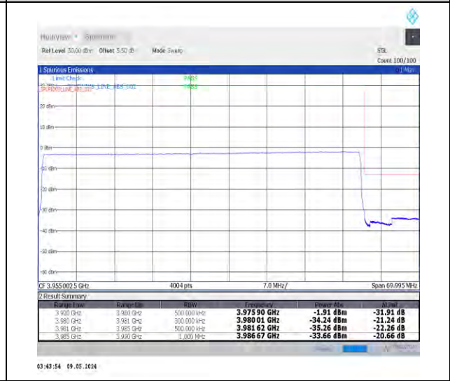
1-N77-3700-3980-PC2-30-60-H-6-CP-QPSK-Outer_Full-162@0-Ant0-1--PASS-see graph
