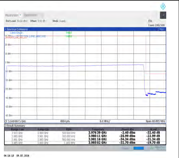
1-N77-3700-3980-PC2-30-70-H-6-CP-QPSK-Outer_Full-189@0-Ant0-1--PASS-see graph
