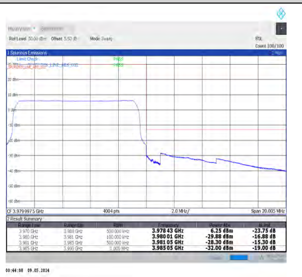
1-N77-3700-3980-PC2-30-10-H-6-CP-QPSK-Outer_Full-24@0-Ant0-1--PASS-see graph
