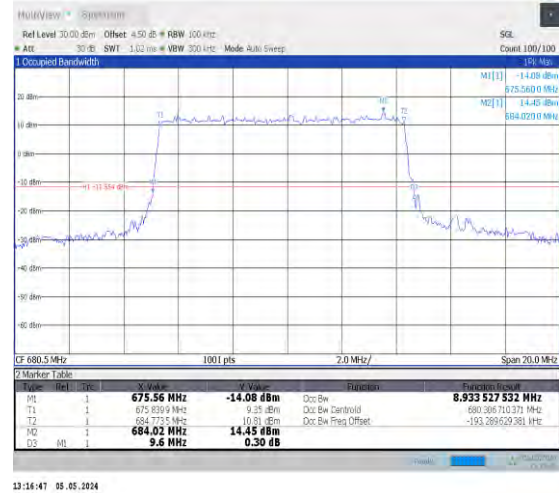
1-N71-PC3-15-10-M-1-DFT-QPSK-Outter_Full-50@0 -Ant0-8.934-9.600-≤10-PASS
