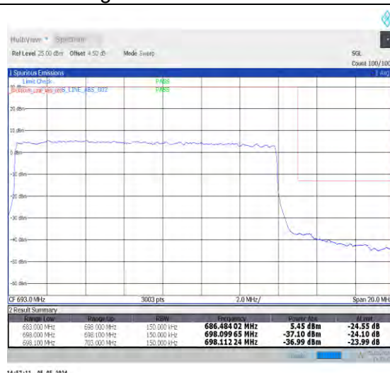
1-N71-PC3-15-15-H-3-DFT-PI2BPSK-Outer_Full-75@0-Ant0-1--PASS-see graph
