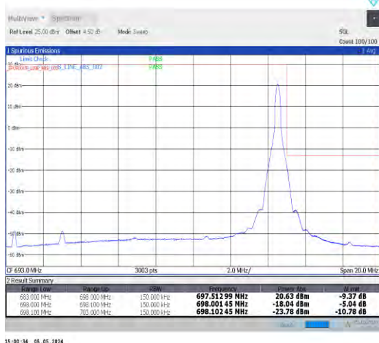
1-N71-PC3-15-15-H-5-CP-QPSK-Edge_1RB_Right-1@78-Ant0-1--PASS-see graph
