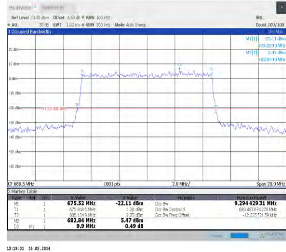
1-N71-PC3-15-10-M-9-CP-256QAM-Outer_Full-52@0 -Ant0-9.294-9.900-≤10-PASS
