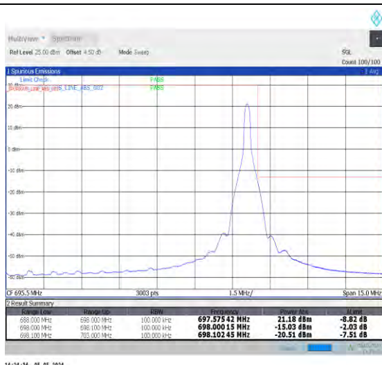
1-N71-PC3-15-10-H-2-DFT-PI2BPSK-Edge_1RB_Right-t1@51-Ant0-1--PASS-see graph
