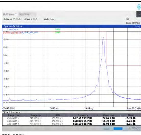
1-N71-PC3-15-15-H-2-DFT-PI2BPSK-Edge_1RB_Right-t1@78-Ant0-1--PASS-see graph
