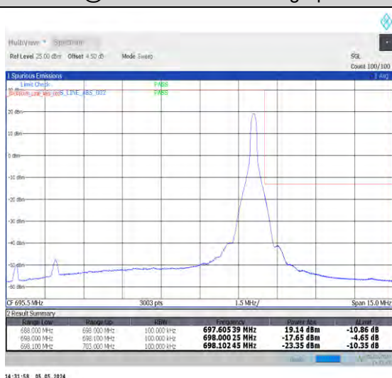
1-N71-PC3-15-10-H-5-CP-QPSK-Edge_1RB_Right-1@51-Ant0-1--PASS-see graph
