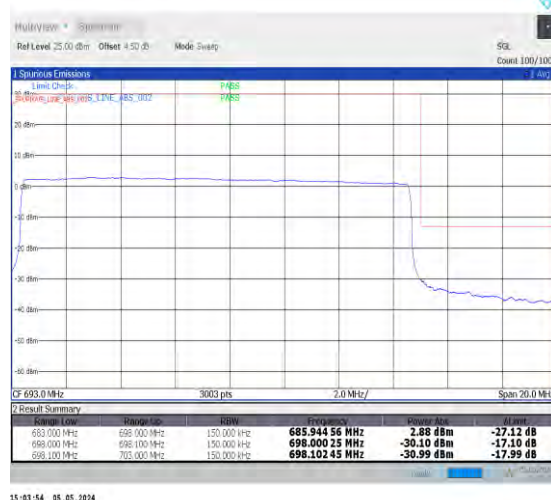
1-N71-PC3-15-15-H-6-CP-QPSK-Outer_Full-79@0-Ant0-1--PASS-see graph
