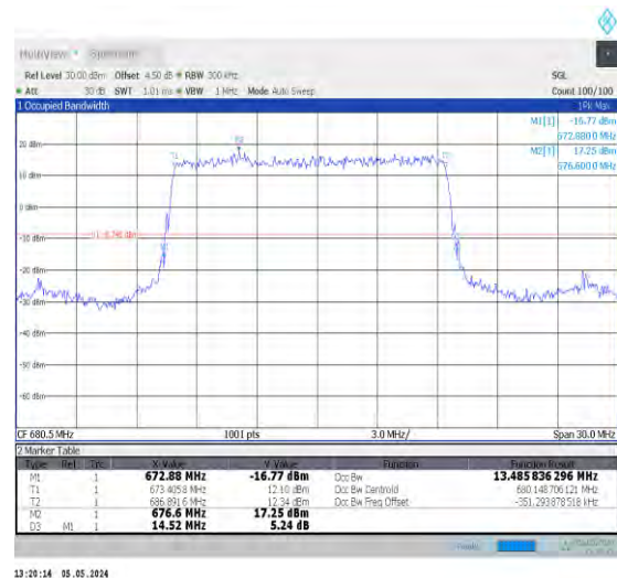
1-N71-PC3-15-15-M-2-DFT-PI2BPSK-Outer_Full-75@0 -Ant0-13.486-14.520-≤15-PASS
