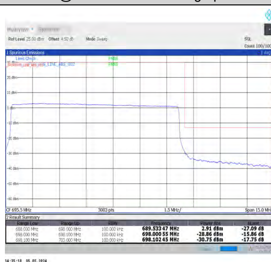
1-N71-PC3-15-10-H-6-CP-QPSK-Outer_Full-52@0-Ant0-1--PASS-see graph
