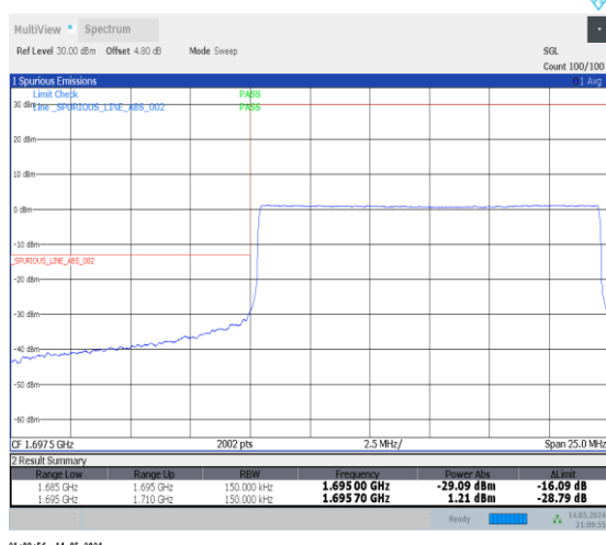
1-N70-PC3-15-15-L-6-CP-QPSK-Outer_Full-79@0-Ant2-1-seegraph-PASS-see graph
