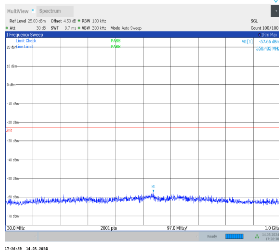
1-N70-PC3-15-15-M-1-DFT-PI2BPSK-Inner_1RB_Le ft-1@1-30-1000-Ant2-550.41--57.66--23-PASS
