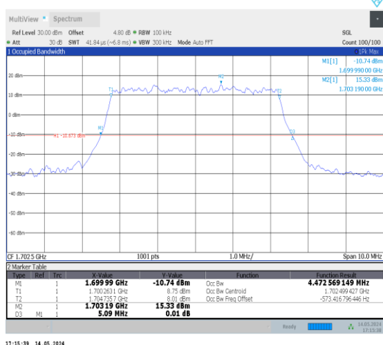
1-N70-PC3-15-5-M-1-DFT-QPSK-Outer_Full-25@0- Ant2-4.473-5.090-≤5-PASS
