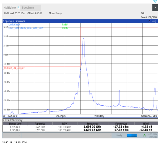
1-N70-PC3-15-10-L-4-CP-QPSK-Edge_1RB_Left-1@0-Ant2-1-seegraph-PASS-see graph
