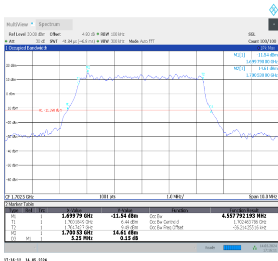
1-N70-PC3-15-5-M-3-DFT-16QAM-Outer_Full-25@0- Ant2-4.558-5.250-≤5-PASS
