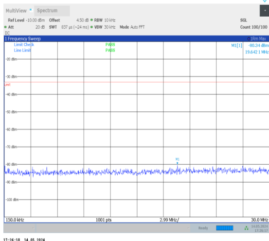
1-N70-PC3-15-15-M-1-DFT-PI2BPSK-Inner_1RB_Le ft-1@1-0.15-30-Ant2-19.64--80.34--33-PASS
