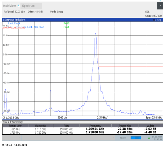
1-N70-PC3-15-15-H-2-DFT-PI2BPSK-Edge_1RB_Right-t1@78-Ant2-1-seegraph-PASS-see graph
