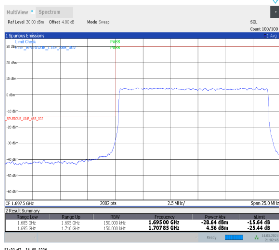
1-N70-PC3-15-15-L-3-DFT-PI2BPSK-Outer_Full-75@0-Ant2-1-seegraph-PASS-see graph
