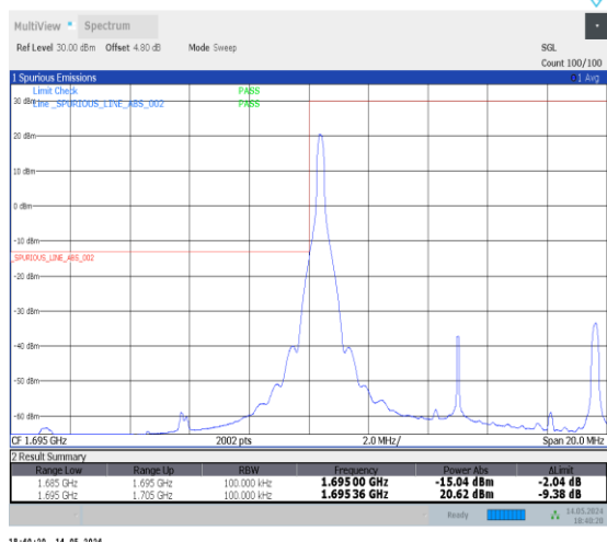
1-N70-PC3-15-10-L-1-DFT-PI2BPSK-Edge_1RB_Left-1@0-Ant2-1-seegraph-PASS-see graph
