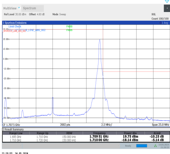
1-N70-PC3-15-15-H-5-CP-QPSK-Edge_1RB_Right-1@78-Ant2-1-seegraph-PASS-see graph
