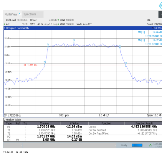
1-N70-PC3-15-5-M-4-DFT-64QAM-Outer_Full-25@0- -Ant2-4.483-5.050-≤5-PASS
