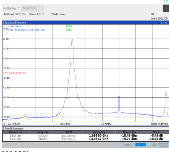
1-N70-PC3-15-15-L-4-CP-QPSK-Edge_1RB_Left-1@0-Ant2-1-seegraph-PASS-see graph
