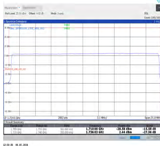
1-N66-15-30-L-6-CP-QPSK-Outer_Full-160@0-Ant0-1-seegraph-PASS-see graph
