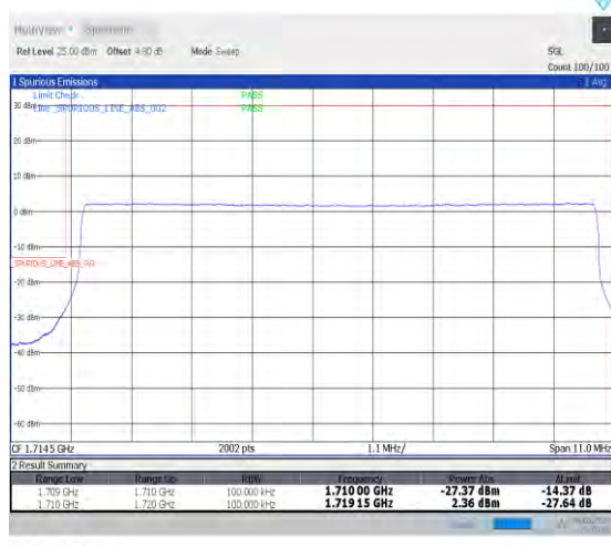
1-N66-15-10-L-6-CP-QPSK-Outer_Full-52@0-Ant0-1-seegraph-PASS-see graph
