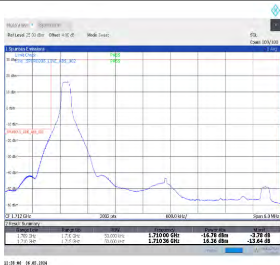
1-N66-15-5-L-4-CP-QPSK-Edge_1RB_Left-1@0-Ant0-1-seegraph-PASS-see graph
