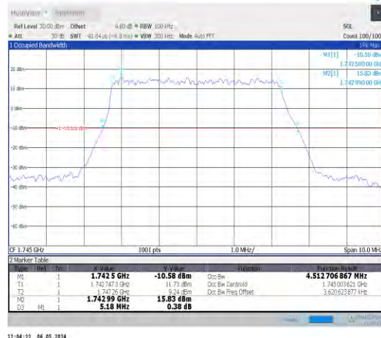
1-N66-15-5-M-2-DFT-PI2BPSK-Outer_Full-25@0-An t0-4.513-5.180-≤5-PASS
