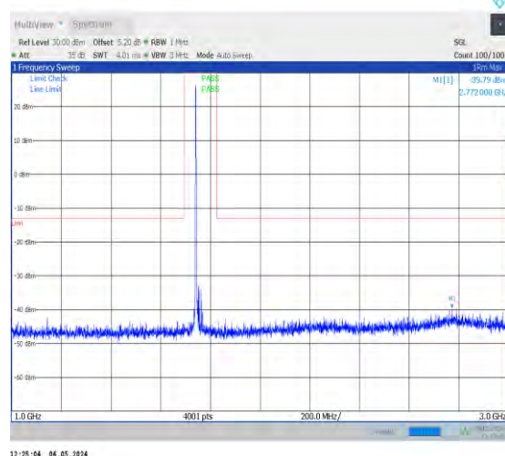
1-N66-15-40-H-1-DFT-PI2BPSK-Inner_1RB_Left-1@ 1-1000-3000-Ant0-2772.00--39.79--13-PASS
