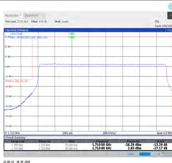
1-N66-15-5-L-6-CP-QPSK-Outer_Full-25@0-Ant0-1-seegraph-PASS-see graph
