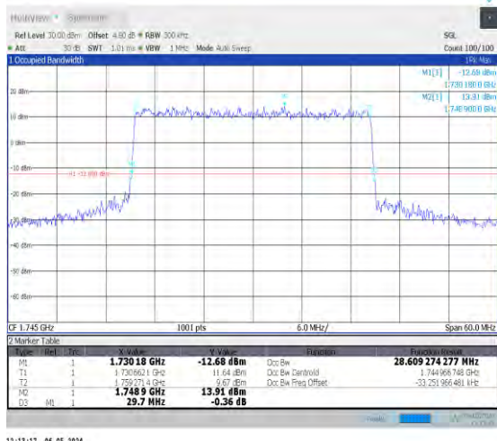
1-N66-15-30-M-1-DFT-QPSK-Outter_Full-160@0-Ant 0-28.61-29.700-≤30-PASS
