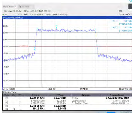
1-N66-15-20-M-1-DFT-QPSK-Outer_Full-100@0-Ant 0-17.922-19.120≤20-PASS
