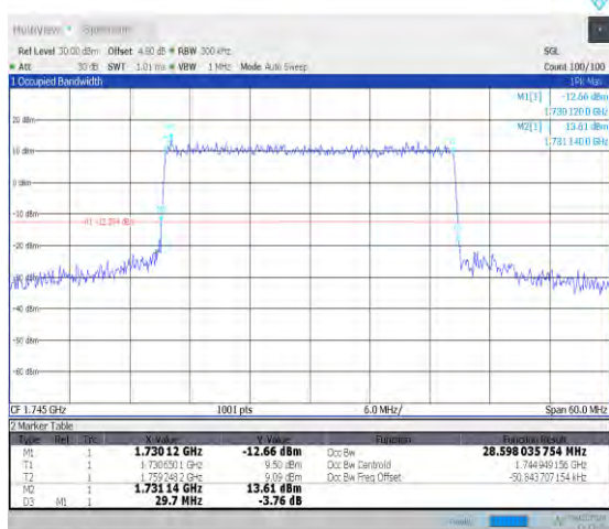
1-N66-15-30-M-3-DFT-16QAM-Outter_Full-160@0-Ant 0-28.6-29.700-≤30-PASS
