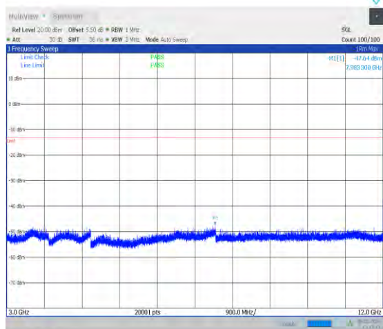
1-N66-15-40-L-1-DFT-PI2BPSK-Inner_1RB_Left-1 @ 1-3000-12000-Ant0-7983.30--47.64--13-PASS
