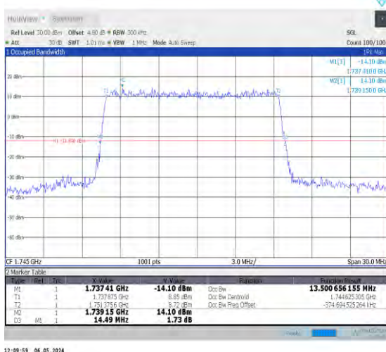
1-N66-15-15-M-5-DFT-256QAM-Outer_Full-75@0-Ant 0-13.501-14.490-≤15-PASS
