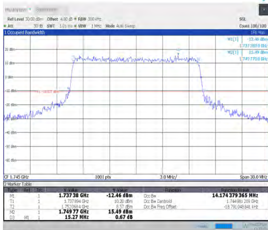
1-N66-15-15-M-7-CP-16QAM-Outer_Full-79@0-Ant0 -14.174-15.270≤15-PASS
