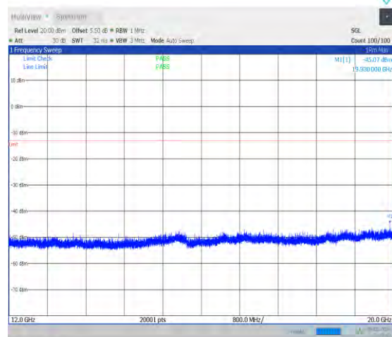
1-N66-15-40-L-1-DFT-PI2BPSK-Inner_1RB_Left-1@ 1-12000-20000-Ant0-19930.00--45.07--13-PASS
