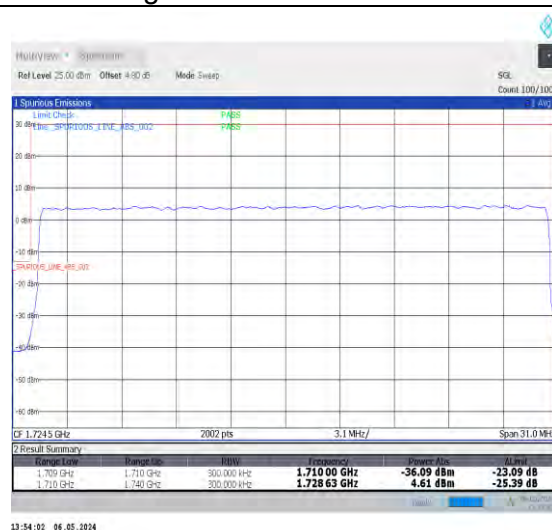
1-N66-15-30-L-3-DFT-PI2BPSK-Outer_Full-160@0-Ant0-1-seegraph-PASS-see graph
