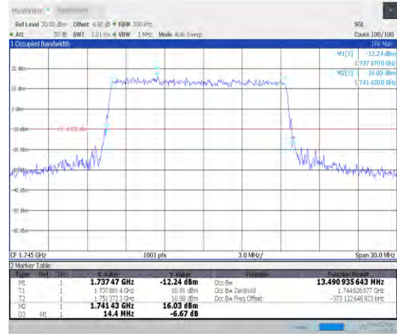
1-N66-15-15-M-4-DFT-64QAM-Outer_Full-75@0-Ant 0-13.491-14.400-≤15-PASS
