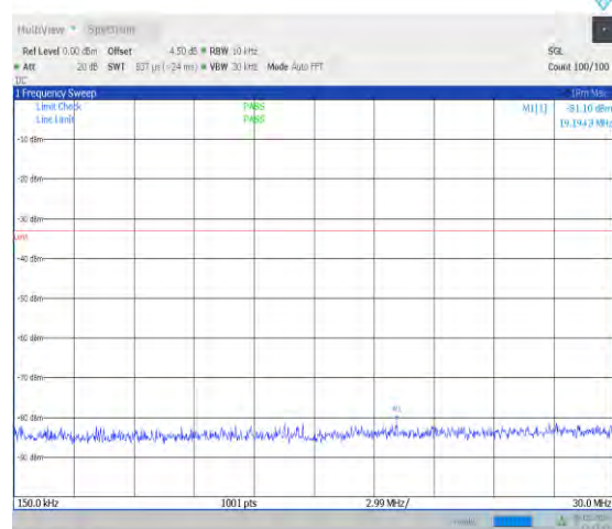
1-N66-15-40-M-1-DFT-PI2BPSK-Inner_1RB_Left-1@ 1-0.15-30-Ant0-19.19--81.10--33-PASS
