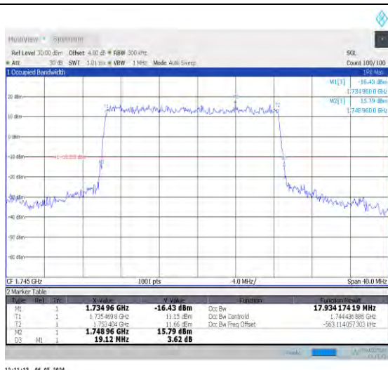
1-N66-15-20-M-2-DFT-PI2BPSK-Outer_Full-100@0-Ant0-17.934-19.120-≤20-PASS
