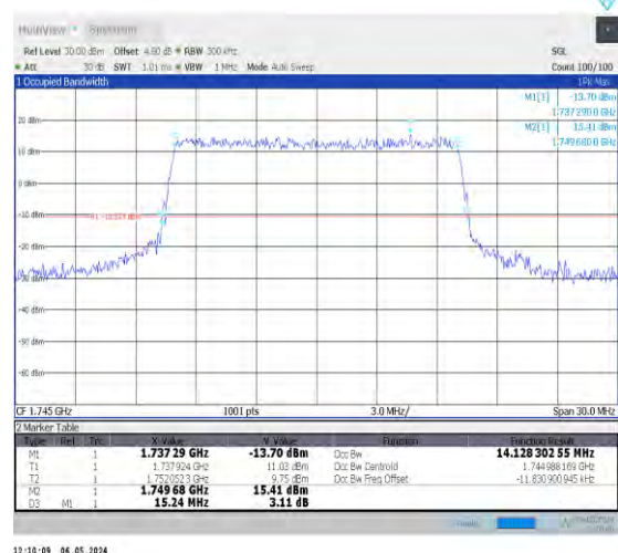
1-N66-15-15-M-6-CP-QPSK-Outer_Full-79@0-Ant 0-14.128-15.240-≤15-PASS
