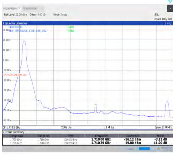
1-N66-15-10-L-4-CP-QPSK-Edge_1RB_Left-1@0-Ant0-1-seegraph-PASS-see graph
