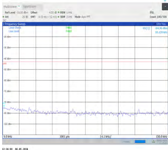
1-N66-15-40-H-1-DFT-PI2BPSK-Inner_1RB_Left-1 @1-0.009-0.15-Ant0-0.01--84.36--43-PASS
