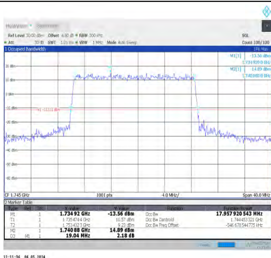
1-N66-15-20-M-4-DFT-64QAM-Outer_Full-100@0-Ant0-17.958-19.040-≤20-PASS
