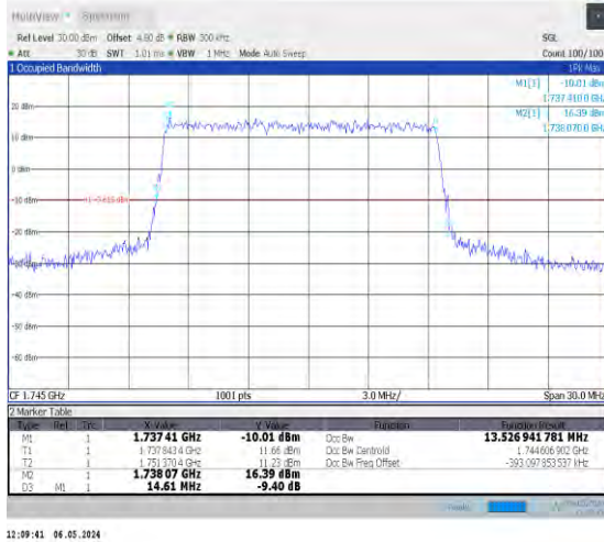
1-N66-15-15-M-3-DFT-16QAM-Outer_Full-75@0-Ant 0-13.527-14.610-≤15-PASS
