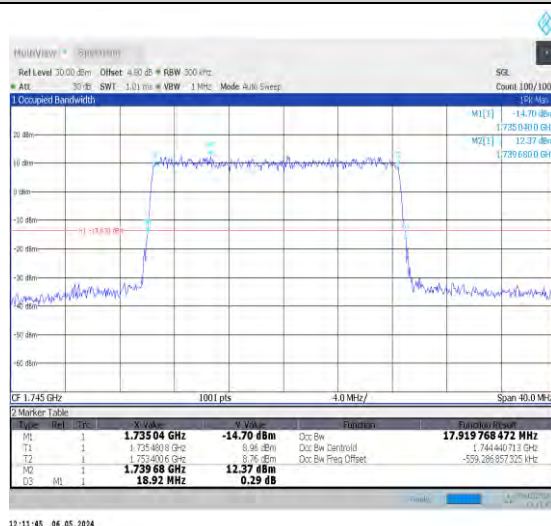
1-N66-15-20-M-5-DFT-256QAM-Outer_Full-100@0-Ant0-17.92-18.920-≤20-PASS
