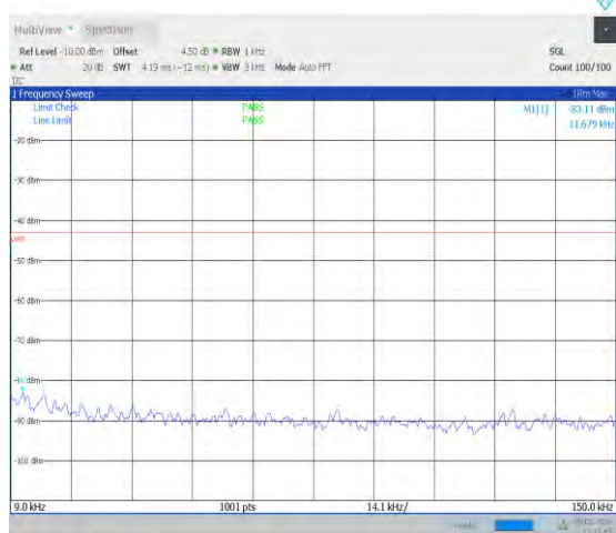
1-N66-15-40-M-1-DFT-PI2BPSK-Inner_1RB_Left-1 @ 1-0.009-0.15-Ant0-0.01--83.11--43-PASS
