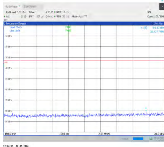
1-N66-15-40-H-1-DFT-PI2BPSK-Inner_1RB_Left-1@ 1-0.15-30-Ant0-26.48--81.13--33-PASS
