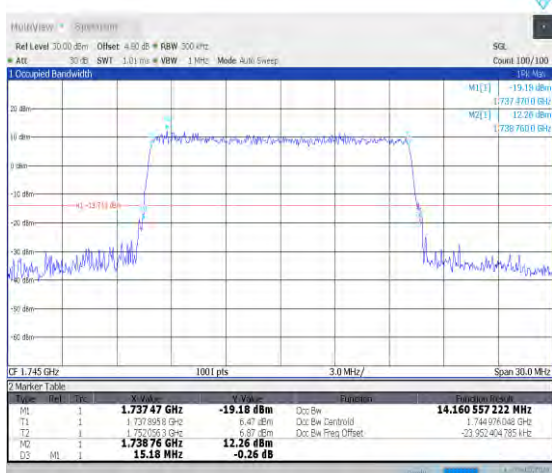
1-N66-15-15-M-9-CP-256QAM-Outer_Full-79@0-Ant 0-14.161-15.180≤15-PASS
