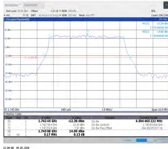
1-N66-15-5-M-4-DFT-64QAM-Outer_Full-25@0-Ant0 -4.504-5.170-≤5-PASS
