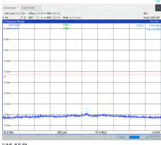
1-N66-15-40-H-1-DFT-PI2BPSK-Inner_1RB_Left-1 @1-30-1000-Ant0-545.07--57.65--23-PASS
