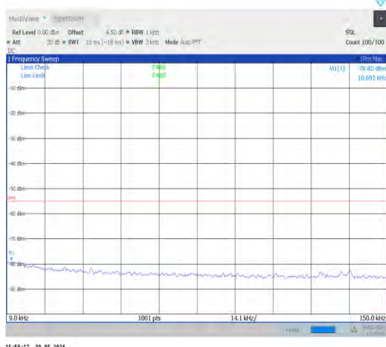
1-N41-30-100-H-1-DFT-PI2BPSK-Inner_1RB_Left-1 @1-0.009-0.15-Ant0-0.01--78.85--55-PASS
