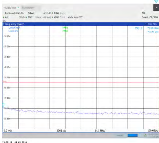
1-N41-30-100-M-1-DFT-PI2BPSK-Inner_1RB_Left-1 @1-0.009-0.15-Ant0-0.01--78.90--55-PASS
