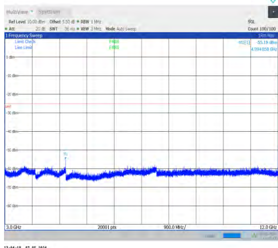
1-N41-30-100-L-1-DFT-PI2BPSK-Inner_1RB_Left-1 @1-3000-12000-Ant0-4994.85--55.18--25-PASS
