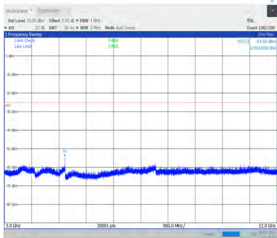
1-N41-30-100-L-1-DFT-PI2BPSK-Inner_1RB_Left-1 @1-3000-12000-Ant0-4994.85--54.58--25-PASS
