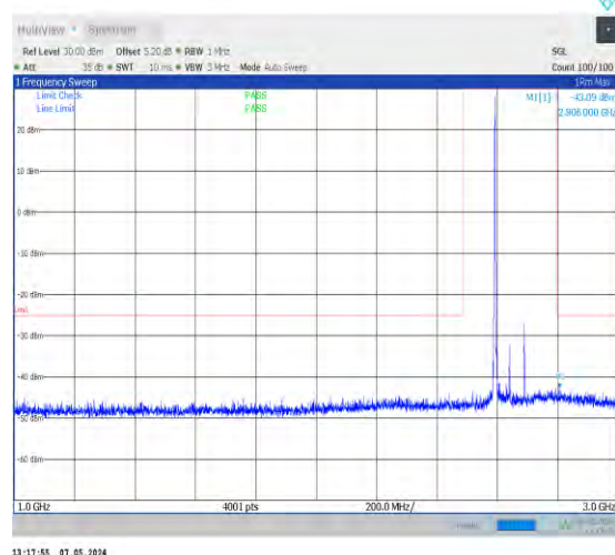
1-N41-30-100-H-1-DFT-PI2BPSK-Inner_1RB_Left-1 @1-1000-3000-Ant0-2806.00--43.09--25-PASS
