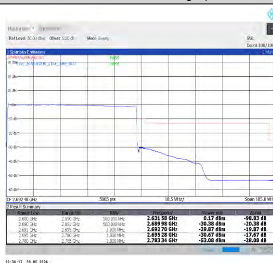
1-N41-30-90-H-6-CP-QPSK-Outer_Full-245@0-Ant0-1--PASS-see graph
