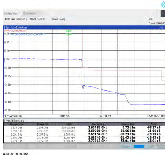
1-N41-30-80-H-6-CP-QPSK-Outer_Full-217@0-A nt0-1--PASS-see graph
