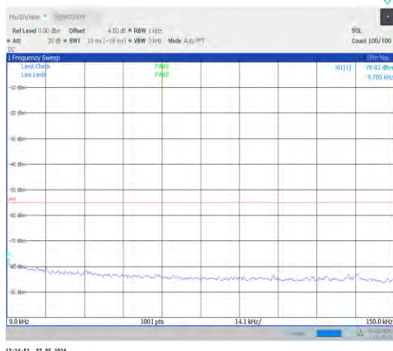
1-N41-30-100-H-1-DFT-PI2BPSK-Inner_1RB_Left-1 @1-0.009-0.15-Ant0-0.01--78.83--55-PASS
