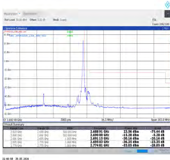
1-N41-30-80-H-5-CP-QPSK-Edge_1RB_Right-1@216- Ant0-1--PASS-see graph
