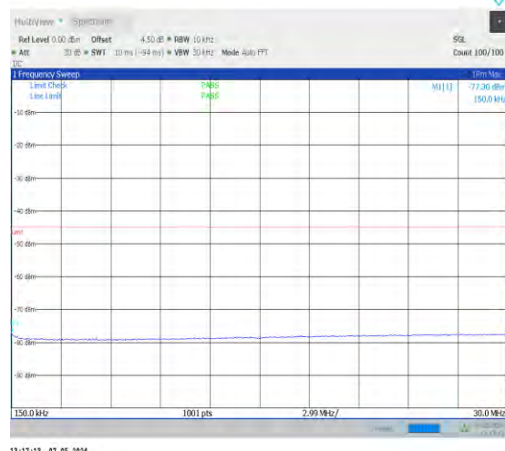
1-N41-30-100-H-1-DFT-PI2BPSK-Inner_1RB_Left-1 @1-0.15-30-Ant0-0.15--77.30--45-PASS
