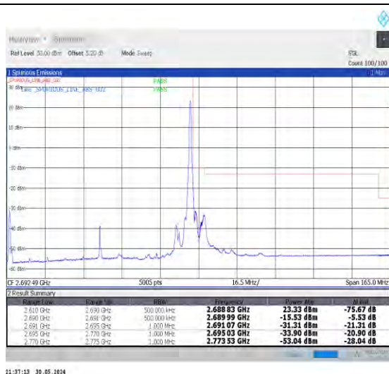
1-N41-30-80-H-2-DFT-PI2BPSK-Edge_1RB_Right-1@ 216-Ant0-1--PASS-see graph
