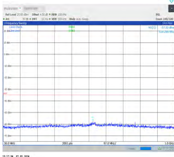
1-N41-30-100-H-1-DFT-PI2BPSK-Inner_1RB_Left-1 @1-30-1000-Ant0-538.28--57.35--35-PASS
