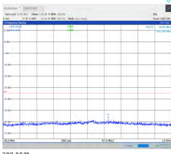
1-N41-30-100-H-1-DFT-PI2BPSK-Inner_1RB_Left-1 @1-30-1000-Ant0-538.28--56.83--35-PASS
