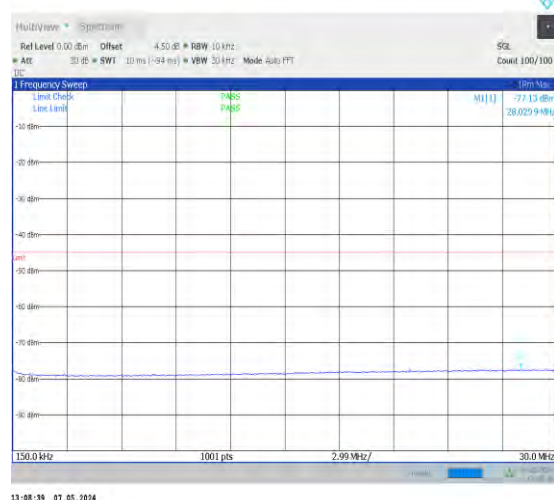
1-N41-30-100-M-1-DFT-PI2BPSK-Inner_1RB_Left-1 @1-0.15-30-Ant0-28.03--77.13--45-PASS
