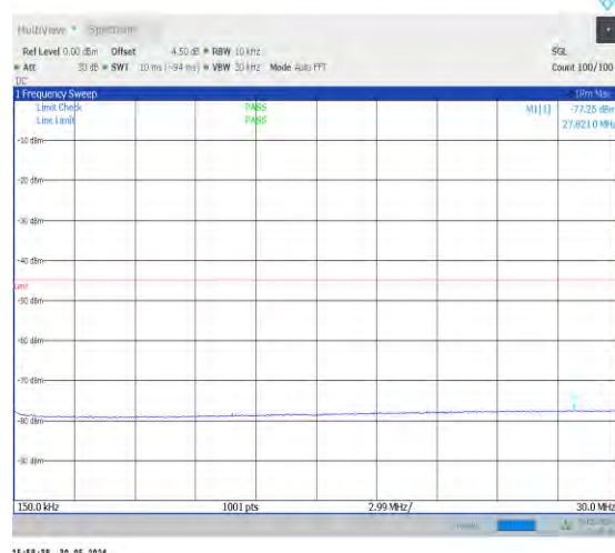
1-N41-30-100-H-1-DFT-PI2BPSK-Inner_1RB_Left-1 @1-0.15-30-Ant0-0.15--77.25--45-PASS
