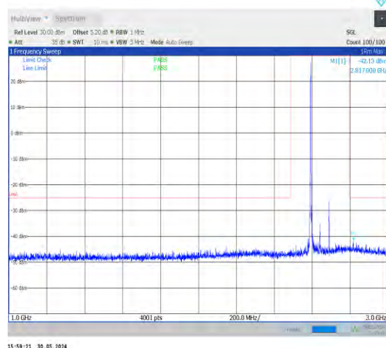
1-N41-30-100-H-1-DFT-PI2BPSK-Inner_1RB_Left-1 @1-1000-3000-Ant0-2806.00--42.13--25-PASS
