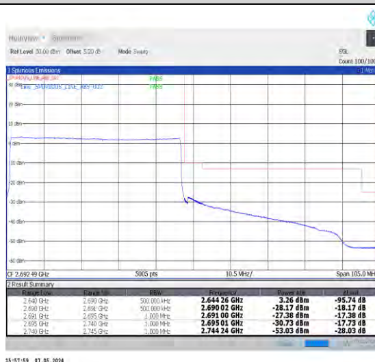
1-N41-30-50-H-6-CP-QPSK-Outer_Full-133@0-A nt0-1--PASS-see graph
