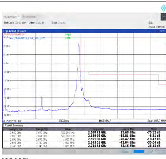
1-N41-30-50-H-2-DFT-PI2BPSK-Edge_1RB_Right-1@ 132-Ant0-1--PASS-see graph
