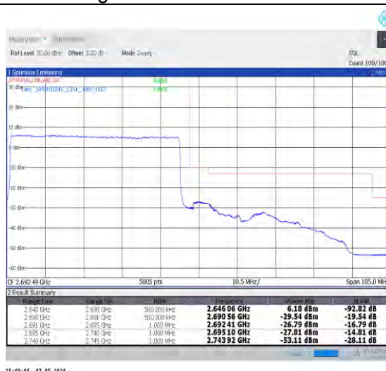
1-N41-30-50-H-3-DFT-PI2BPSK-Outer_Full-128@ 0-Ant0-1--PASS-see graph
