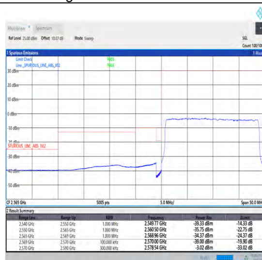
1-N38-30-20-L-3-DFT-PI2BPSK-Outer_Full-50@0-Ant0-1--PASS-see graph
