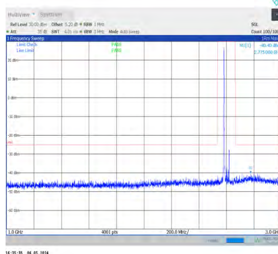
1-N38-30-40-H-1-DFT-PI2BPSK-Inner_1RB_Left-1@ 1-1000-3000-Ant0-2775.00--40.40--25-PASS
