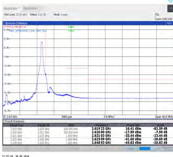
1-N38-30-10-H-5-CP-QPSK-Edge_1RB_Right-1@23-Ant0-1--PASS-see graph
