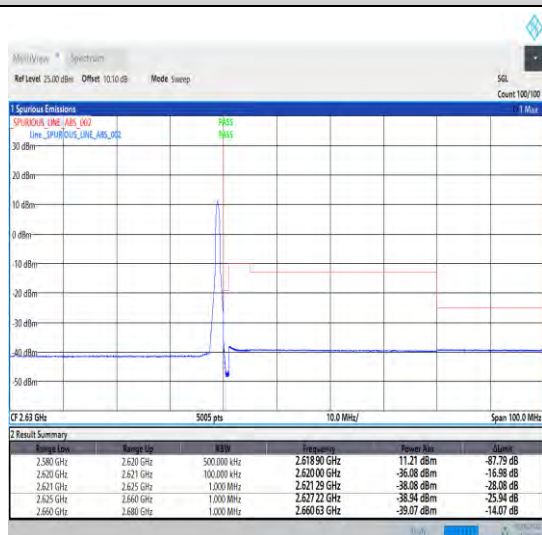
1-N38-30-40-H-5-CP-QPSK-Edge_1RB_Right-1@105-Ant0-1--PASS-see graph
