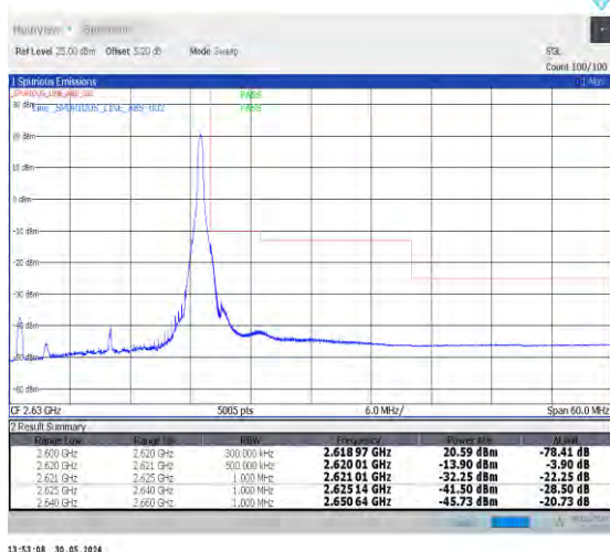
1-N38-30-20-H-5-CP-QPSK-Edge_1RB_Right-1@50-Ant0-1--PASS-see graph
