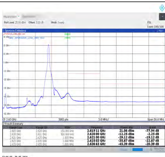
1-N38-30-15-H-2-DFT-PI2BPSK-Edge_1RB_Right-1@37-Ant0-1--PASS-see graph
