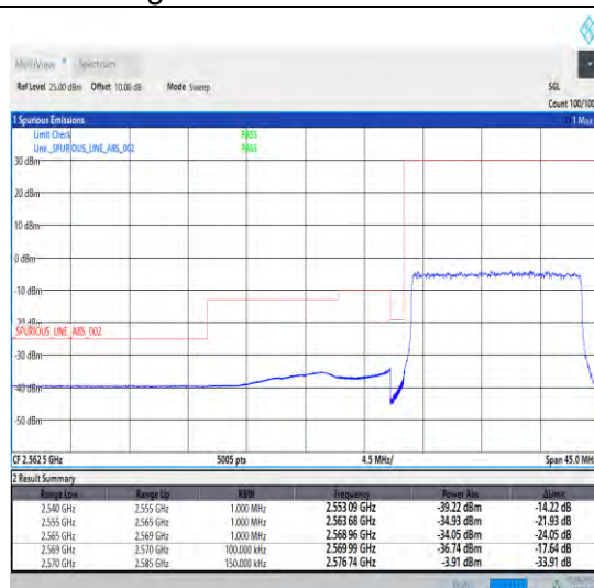
1-N38-30-15-L-3-DFT-PI2BPSK-Outer_Full-36@0-Ant0-1--PASS-see graph
