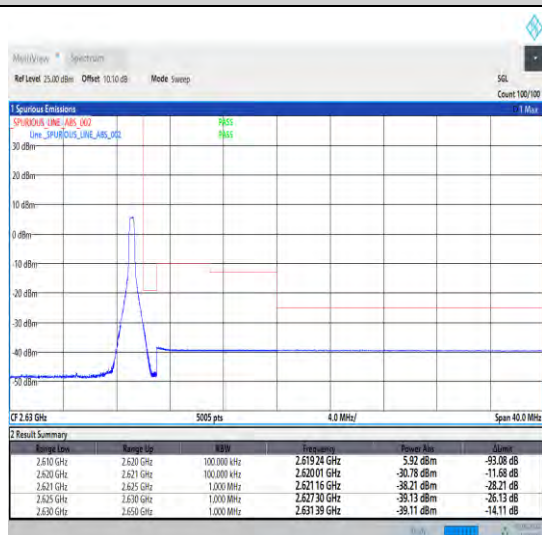
1-N38-30-10-H-5-CP-QPSK-Edge_1RB_Right-1@23-Ant0-1--PASS-see graph
