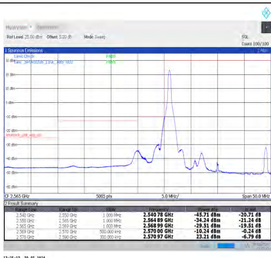
1-N38-30-20-L-1-DFT-PI2BPSK-Edge_1RB_Left-1@0-Ant0-1--PASS-see graph
