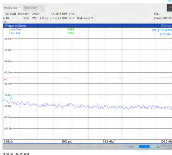
1-N38-30-40-L-1-DFT-PI2BPSK-Inner_1RB_Left-1 @1-0.009-0.15-Ant0-0.02--74.04--55-PASS
