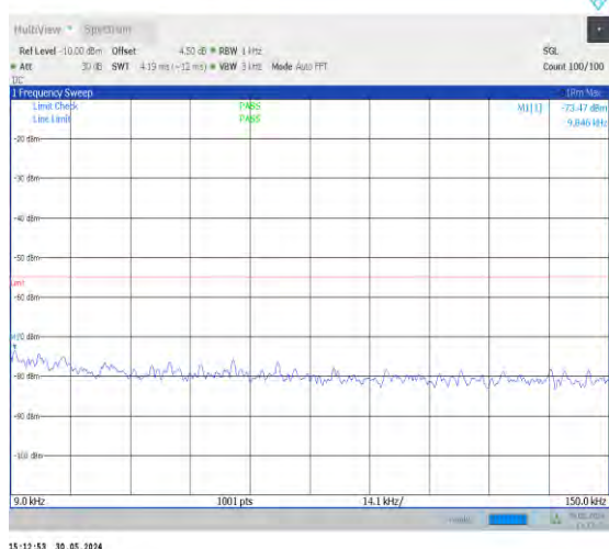
1-N38-30-40-M-1-DFT-PI2BPSK-Inner_1RB_Left-1 @ 1-0.009-0.15-Ant0-0.02--73.47--55-PASS
