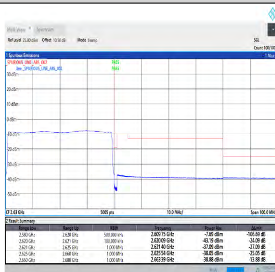
1-N38-30-40-H-6-CP-QPSK-Outer_Full-106@0-Ant0-1--PASS-see graph
