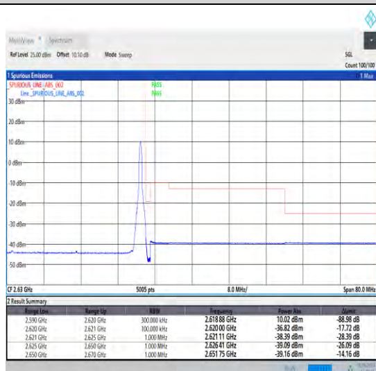
1-N38-30-30-H-5-CP-QPSK-Edge_1RB_Right-1@77-Ant0-1--PASS-see graph
