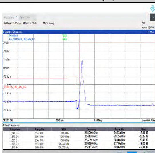
1-N38-30-30-L-4-CP-QPSK-Edge_1RB_Left-1@0-Ant0-1--PASS-see graph
