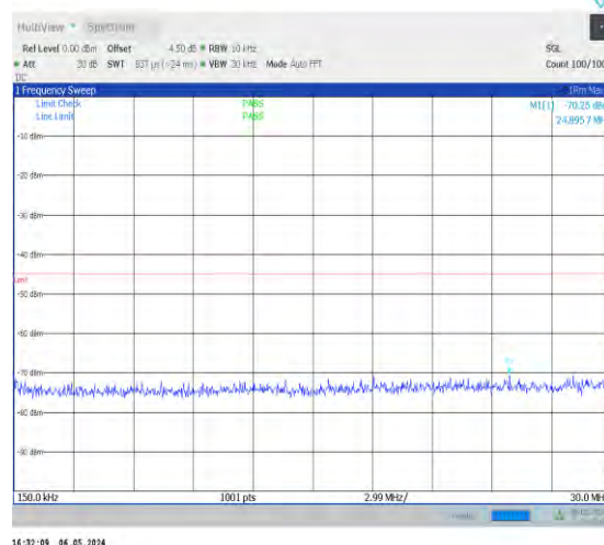
1-N38-30-40-L-1-DFT-PI2BPSK-Inner_1RB_Left-1@ 1-0.15-30-Ant0-24.90--70.25--45-PASS
