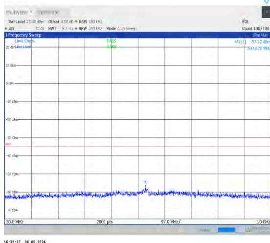
1-N38-30-40-L-1-DFT-PI2BPSK-Inner_1RB_Left-1 @1-30-1000-Ant0-541.68--57.72--35-PASS
