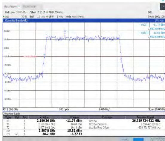
1-N38-30-30-M-2-DFT-PI2BPSK-Outer_Full-75@0-A nt0-26.762-28.200-≤30-PASS
