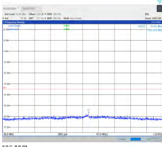
1-N38-30-40-H-1-DFT-PI2BPSK-Inner_1RB_Left-1 @1-30-1000-Ant0-551.38--57.22--35-PASS
