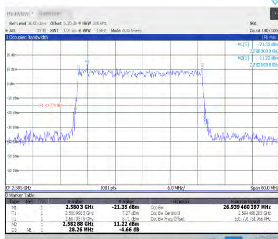
1-N38-30-30-M-5-DFT-256QAM-Outer_Full-75@0-A nt0-26.941-28.260-≤30-PASS
