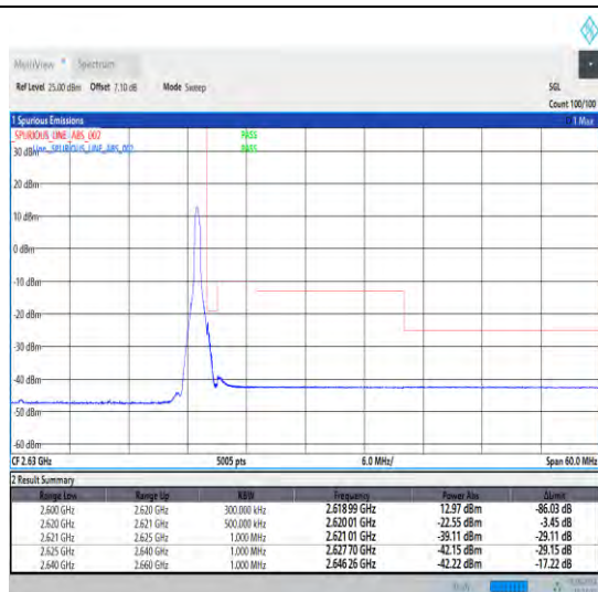
1-N38-30-20-H-2-DFT-PI2BPSK-Edge_1RB_Right-1@50-Ant0-1--PASS-see graph
