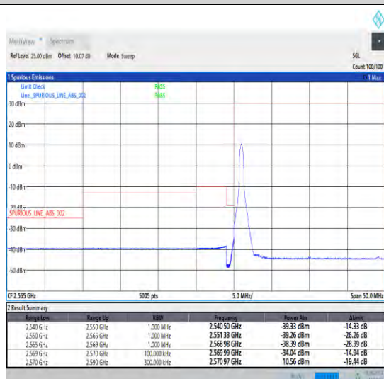
1-N38-30-20-L-4-CP-QPSK-Edge_1RB_Left-1@0-Ant0-1--PASS-see graph
