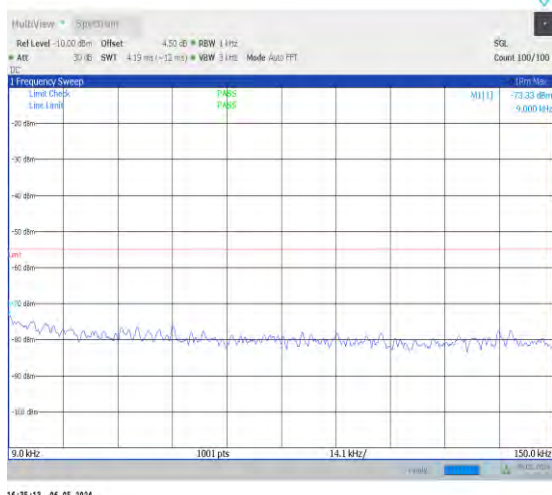
1-N38-30-40-H-1-DFT-PI2BPSK-Inner_1RB_Left-1 @1-0.009-0.15-Ant0-0.01--73.33--55-PASS
