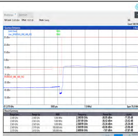
1-N38-30-40-L-6-CP-QPSK-Outer_Full-106@0-Ant0-1--PASS-see graph
