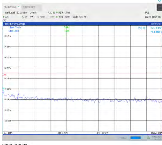
1-N38-30-40-H-1-DFT-PI2BPSK-Inner_1RB_Left-1 @1-0.009-0.15-Ant0-0.01--72.79--55-PASS
