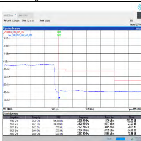
1-N38-30-40-H-3-DFT-PI2BPSK-Outer_Full-100@0-Ant0-1--PASS-see graph
