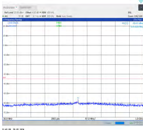
1-N38-30-40-H-1-DFT-PI2BPSK-Inner_1RB_Left-1 @1-30-1000-Ant0-551.38--58.01--35-PASS
