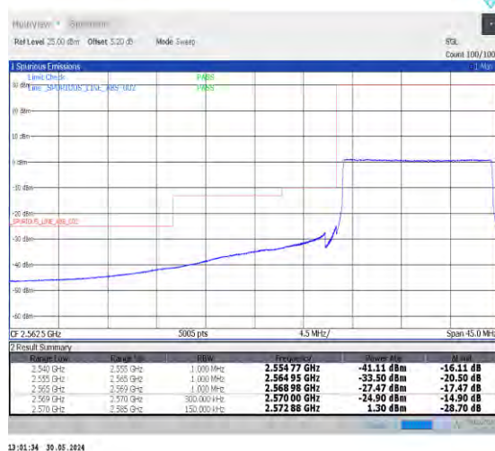
1-N38-30-15-L-6-CP-QPSK-Outer_Full-38@0-Ant0-1--PASS-see graph
