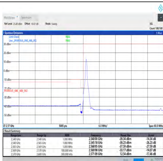
1-N38-30-30-L-1-DFT-PI2BPSK-Edge_1RB_Left-1@0-Ant0-1--PASS-see graph
