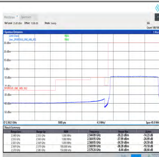
1-N38-30-15-L-6-CP-QPSK-Outer_Full-38@0-Ant0-1--PASS-see graph
