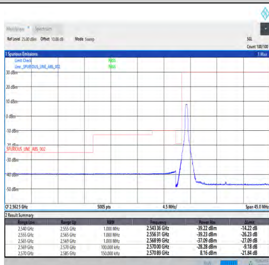
1-N38-30-15-L-4-CP-QPSK-Edge_1RB_Left-1@0-Ant0-1--PASS-see graph
