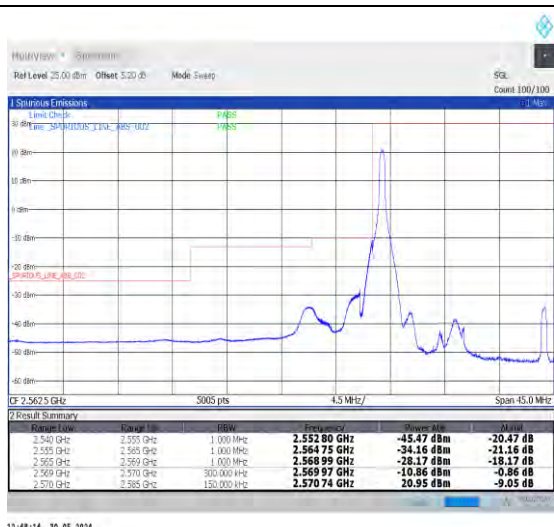
1-N38-30-15-L-1-DFT-PI2BPSK-Edge_1RB_Left-1@0-Ant0-1--PASS-see graph
