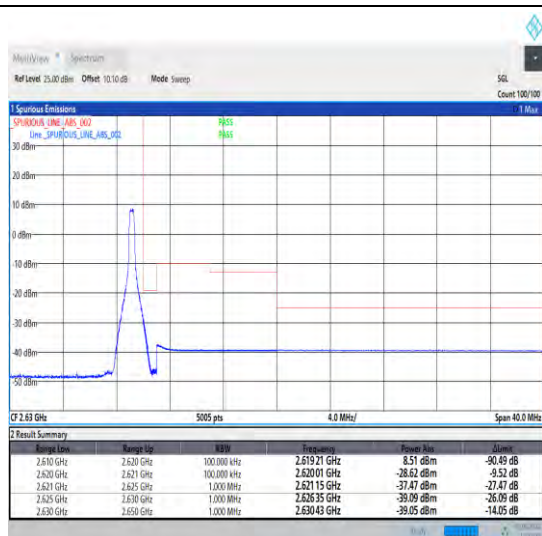
1-N38-30-10-H-2-DFT-PI2BPSK-Edge_1RB_Right-1@23-Ant0-1--PASS-see graph
