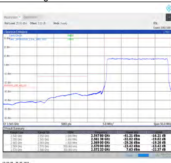
1-N38-30-20-L-3-DFT-PI2BPSK-Outer_Full-50@0-Ant0-1--PASS-see graph
