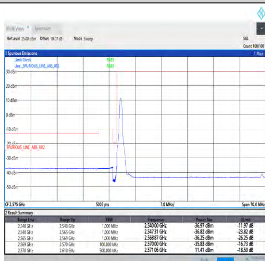
1-N38-30-40-L-4-CP-QPSK-Edge_1RB_Left-1@0-Ant0-1--PASS-see graph
