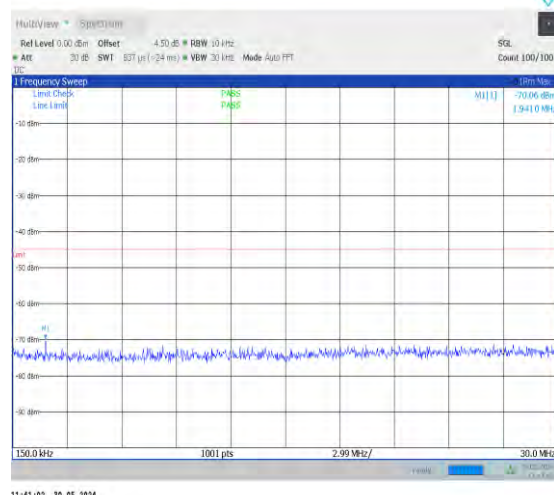
1-N38-30-40-H-1-DFT-PI2BPSK-Inner_1RB_Left-1@ 1-0.15-30-Ant0-27.07--70.06--45-PASS
