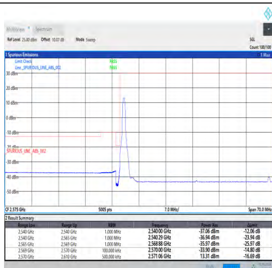
1-N38-30-40-L-1-DFT-PI2BPSK-Edge_1RB_Left-1@0-Ant0-1--PASS-see graph
