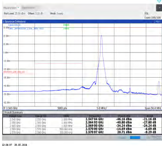
1-N38-30-20-L-4-CP-QPSK-Edge_1RB_Left-1@0-Ant0-1--PASS-see graph
