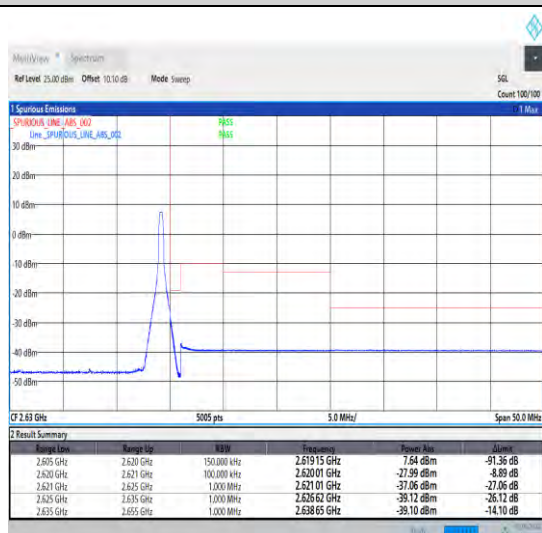
1-N38-30-15-H-5-CP-QPSK-Edge_1RB_Right-1@37-Ant0-1--PASS-see graph
