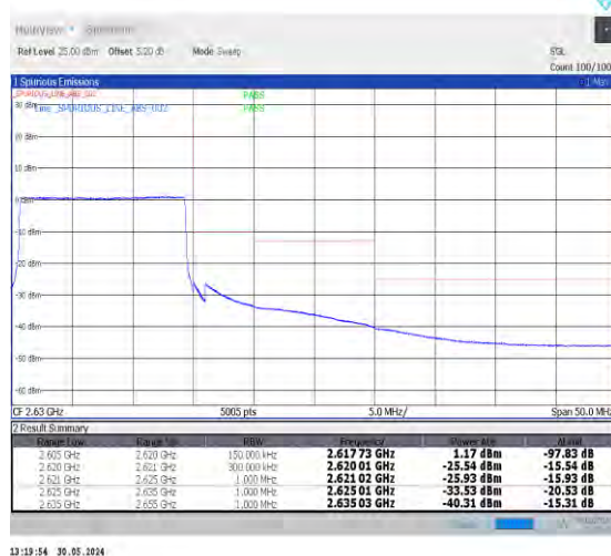
1-N38-30-15-H-6-CP-QPSK-Outer_Full-38@0-Ant0-1--PASS-see graph
