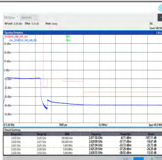
1-N38-30-10-H-6-CP-QPSK-Outer_Full-24@0-Ant0-1--PASS-see graph
