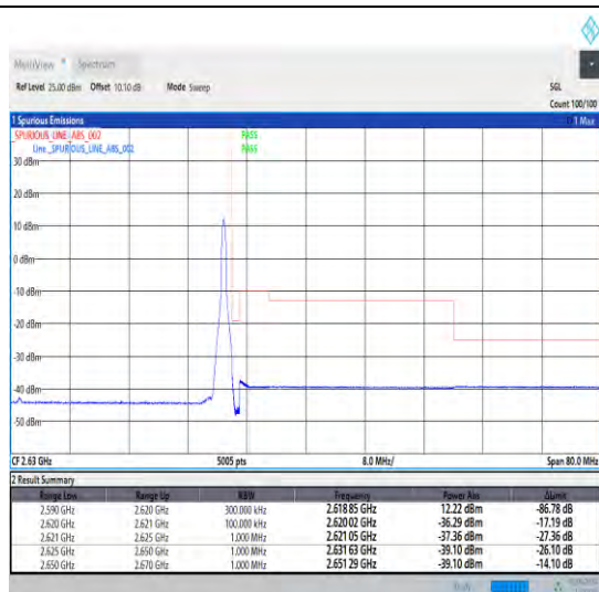
1-N38-30-30-H-2-DFT-PI2BPSK-Edge_1RB_Right-1@77-Ant0-1--PASS-see graph
