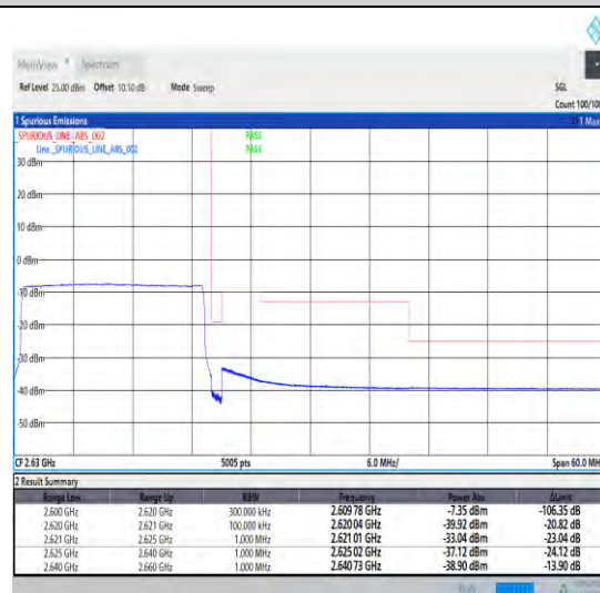
1-N38-30-20-H-6-CP-QPSK-Outer_Full-51@0-Ant0-1--PASS-see graph
