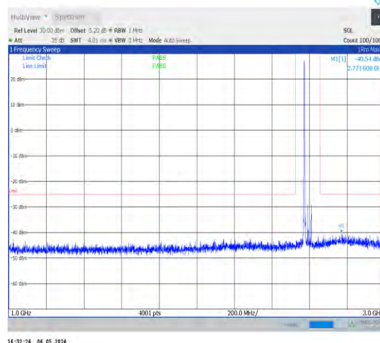
1-N38-30-40-L-1-DFT-PI2BPSK-Inner_1RB_Left-1@ 1-1000-3000-Ant0-2771.00--40.54--25-PASS
