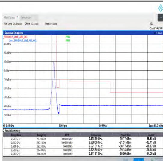
1-N38-30-20-H-5-CP-QPSK-Edge_1RB_Right-1@50-Ant0-1--PASS-see graph
