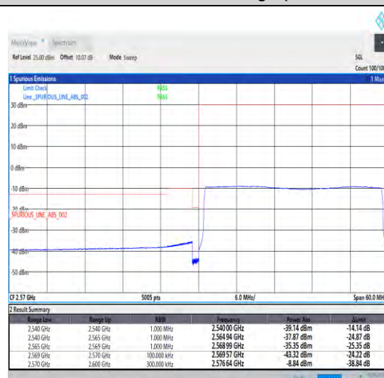
1-N38-30-30-L-6-CP-QPSK-Outer_Full-78@0-Ant0-1--PASS-see graph
