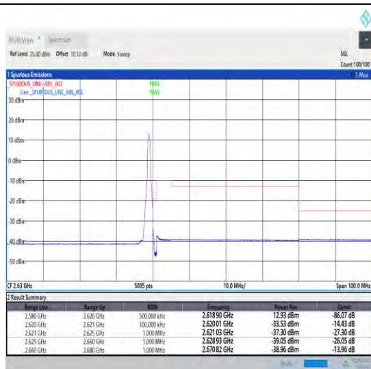
1-N38-30-40-H-2-DFT-PI2BPSK-Edge_1RB_Right-1@105-Ant0-1--PASS-see graph
