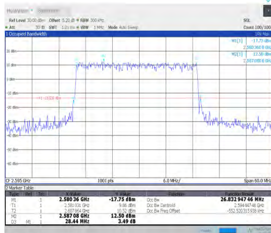
1-N38-30-30-M-3-DFT-16QAM-Outer_Full-75@0-Ant 0-26.834-28.440-≤30-PASS
