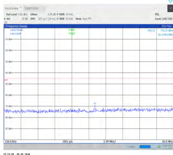
1-N38-30-40-M-1-DFT-PI2BPSK-Inner_1RB_Left-1@ 1-0.15-30-Ant0-29.91--70.75--45-PASS
