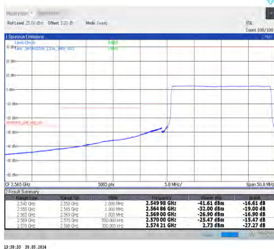
1-N38-30-20-L-6-CP-QPSK-Outer_Full-51@0-Ant0-1--PASS-see graph
