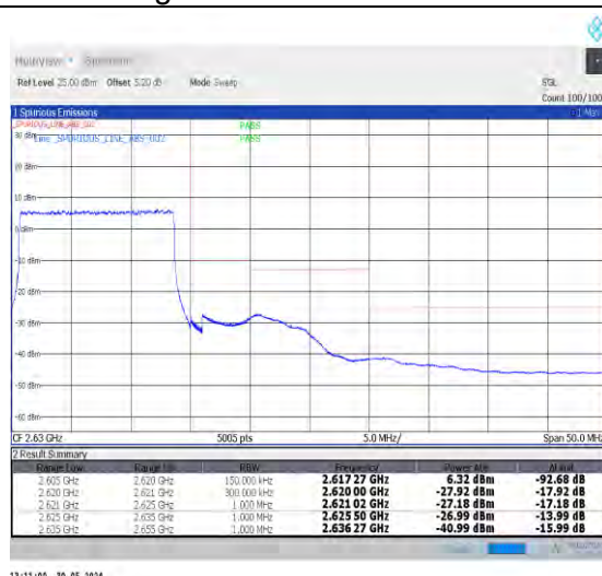
1-N38-30-15-H-3-DFT-PI2BPSK-Outer_Full-36@0-Ant0-1--PASS-see graph
