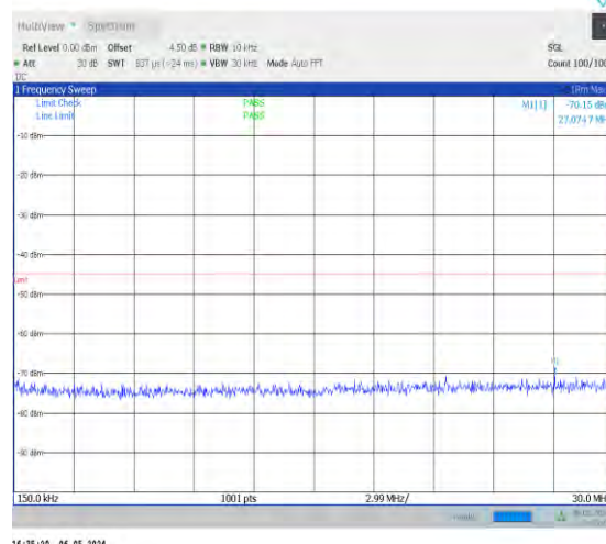
1-N38-30-40-H-1-DFT-PI2BPSK-Inner_1RB_Left-1@ 1-0.15-30-Ant0-27.07--70.15--45-PASS
