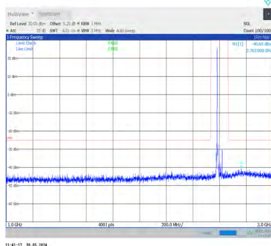
1-N38-30-40-H-1-DFT-PI2BPSK-Inner_1RB_Left-1@ 1-1000-3000-Ant0-2775.00--40.65--25-PASS
