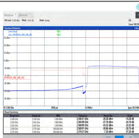
1-N38-30-20-L-6-CP-QPSK-Outer_Full-51@0-Ant0-1--PASS-see graph
