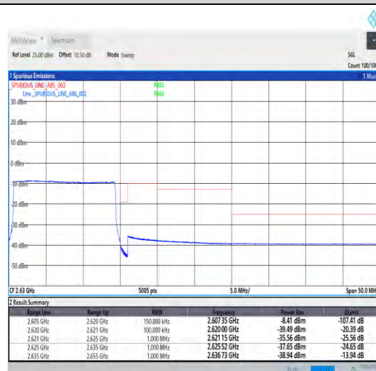
1-N38-30-15-H-6-CP-QPSK-Outer_Full-38@0-Ant0-1--PASS-see graph
