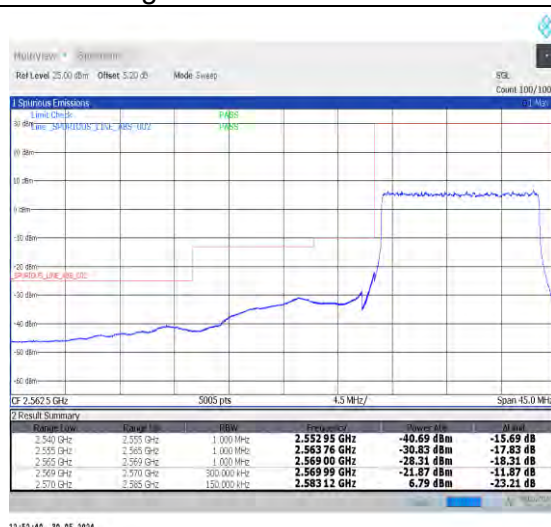
1-N38-30-15-L-3-DFT-PI2BPSK-Outer_Full-36@0-Ant0-1--PASS-see graph
