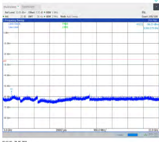
1-N38-30-40-L-1-DFT-PI2BPSK-Inner_1RB_Left-1 @ 1-3000-12000-Ant0-3621.90--56.23--25-PASS
