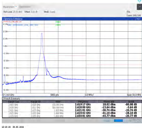
1-N38-30-15-H-5-CP-QPSK-Edge_1RB_Right-1@37-Ant0-1--PASS-see graph
