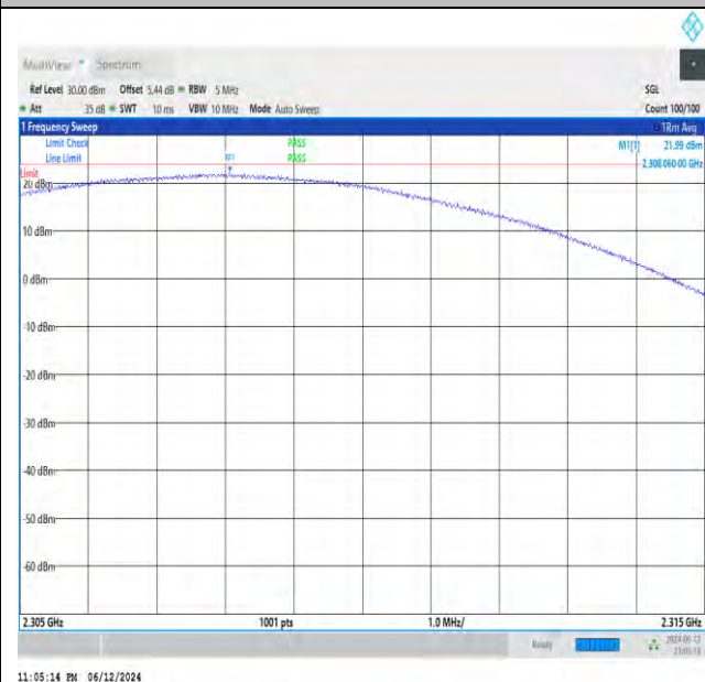
NTVN_N30_PC3_15_5_M_TID23_NS_01_2305_2315_#1
