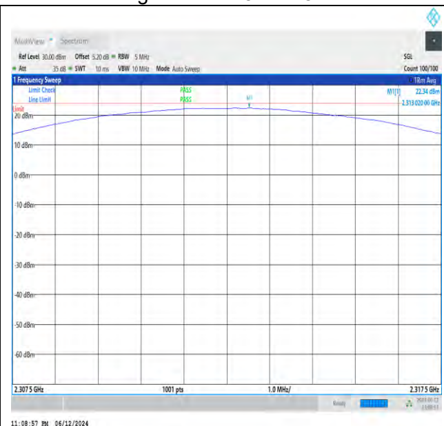
NTNV_N30_PC3_15_5_H_TID5_NS_01_2307.5_2317.5_#1
