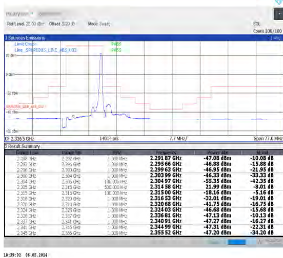
1-N30-PC3-15-10-H-5-CP-QPSK-Edge_1RB_Right-1@51-Ant0-1--PASS-see graph
