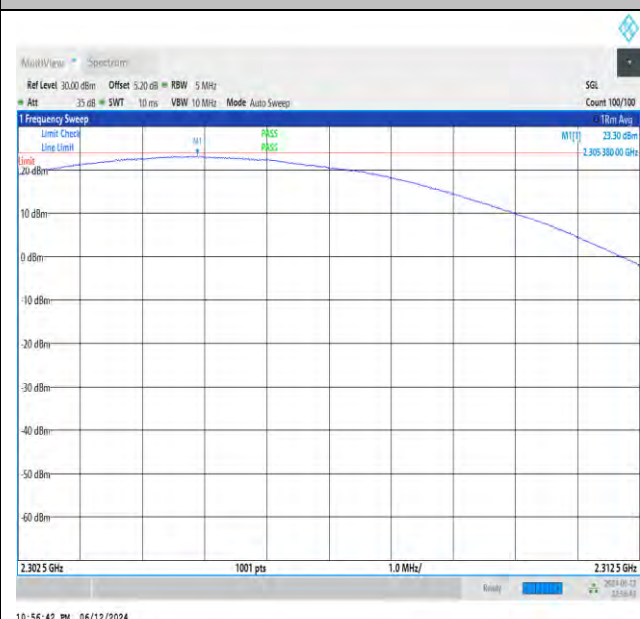
NTVN_N30_PC3_15_5_L_TID7_NS_01_2302.5_2312.5_ #1
