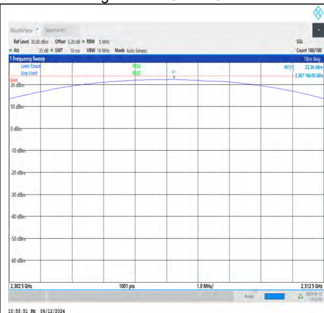
NTVN_N30_PC3_15_5_L_TID5_NS_01_2302.5_2312.5_ #1
