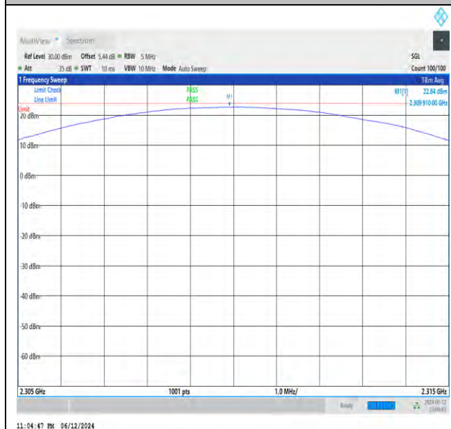
NTVN_N30_PC3_15_5_M_TID22_NS_01_2305_2315_#1
