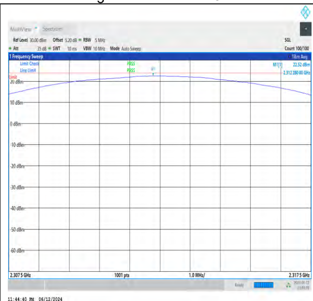
NTVN_N30_PC3_15_5_H_TID1_NS_01_2307.5_2317.5_#1
