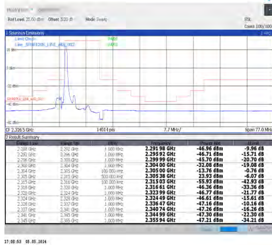
1-N30-PC3-15-10-L-1-DFT-PI2BPSK-Edge_1RB_Left-1@0-Ant0-1--PASS-see graph
