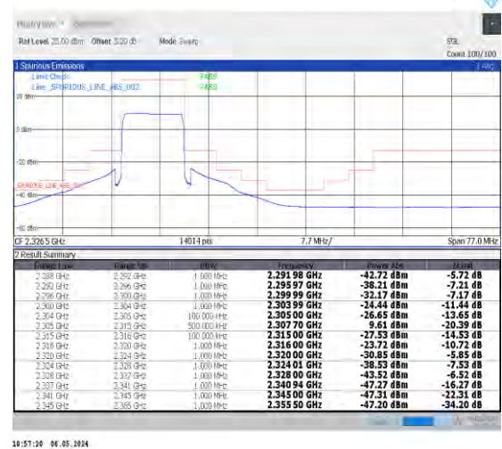
1-N30-PC3-15-10-H-6-CP-QPSK-Outer_Full-52@0-Ant0-1--PASS-see graph
