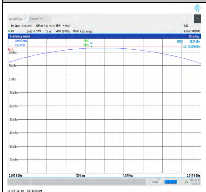
NTVN_N30_PC3_15_5_H_TID2_NS_01_2307.5_2317.5_#1
