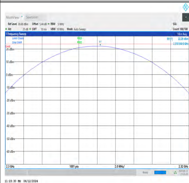
NTNV_N30_PC3_15_10_M_TID22_NS_01_2300_2320_#
