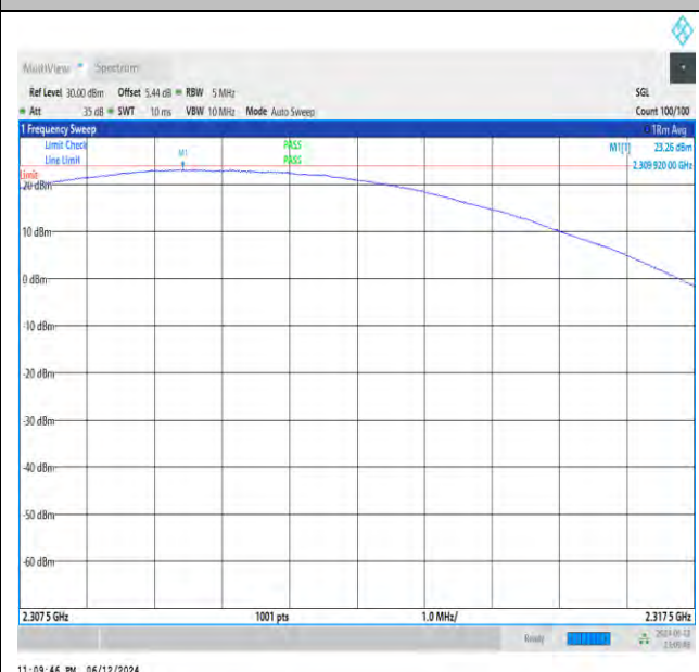
NTNV_N30_PC3_15_5_H_TID7_NS_01_2307.5_2317.5_#1
