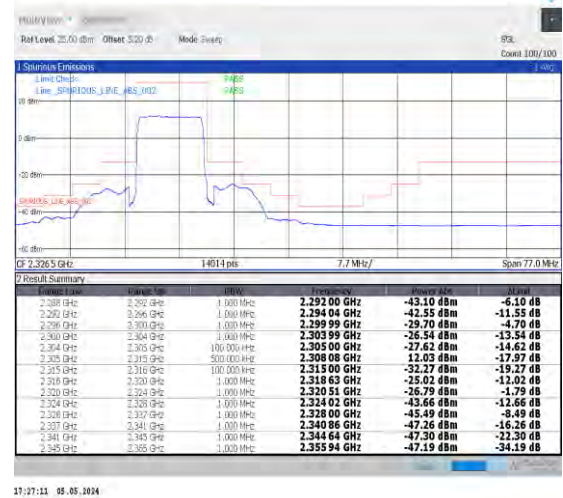
1-N30-PC3-15-10-L-3-DFT-PI2BPSK-Outer_Full-50@0-Ant0-1--PASS-see graph
