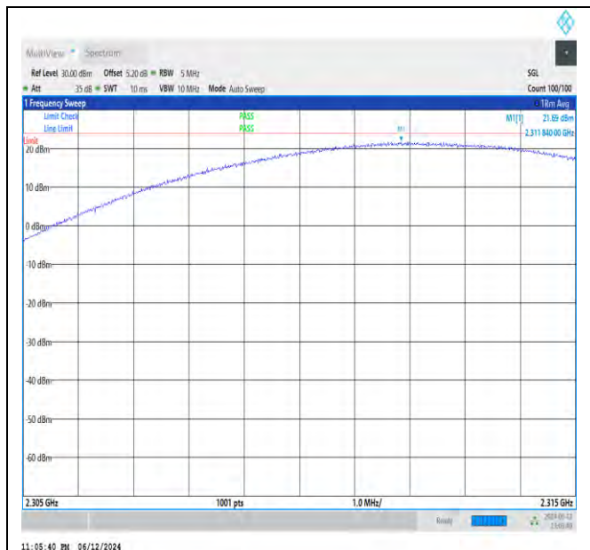
NTVN_N30_PC3_15_5_M_TID24_NS_01_2305_2315_#1
