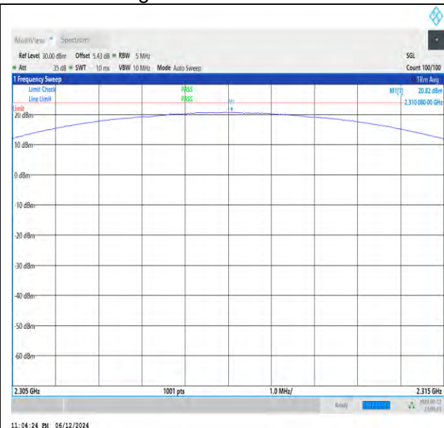
NTVN_N30_PC3_15_5_M_TID21_NS_01_2305_2315_#1
