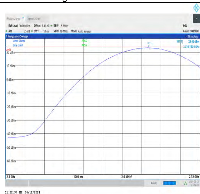
NTNV_N30_PC3_15_10_M_TID8_NS_01_2300_2320_#1
