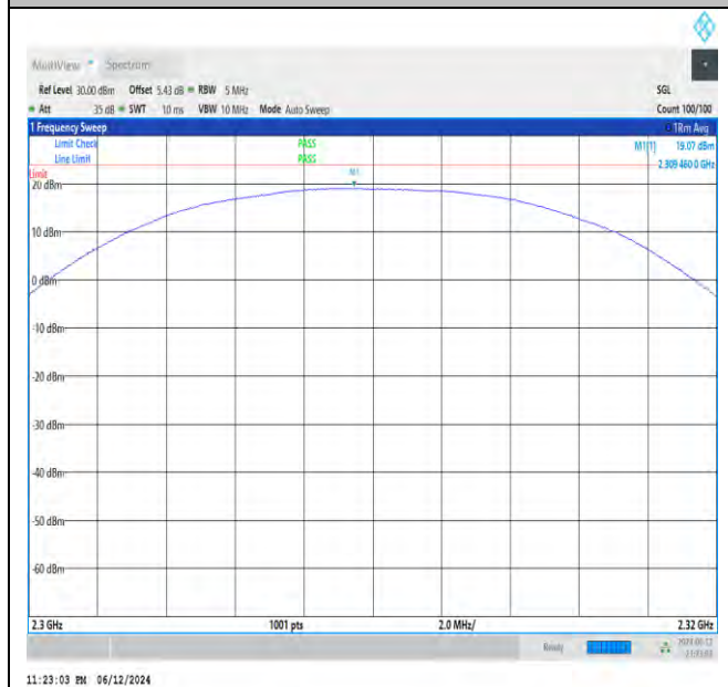
NTNV_N30_PC3_15_10_M_TID21_NS_01_2300_2320_#
