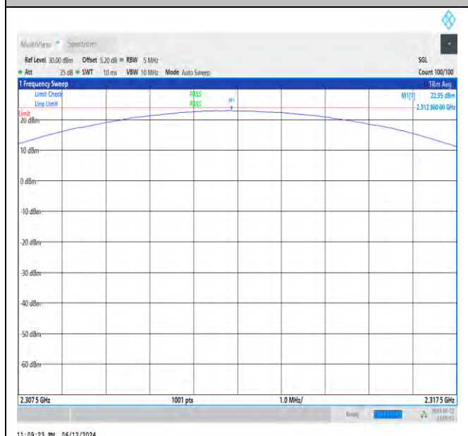
NTNV_N30_PC3_15_5_H_TID6_NS_01_2307.5_2317.5_#1
