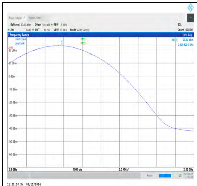
NTNV_N30_PC3_15_10_M_TID7_NS_01_2300_2320_#1
