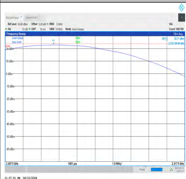
NTVN_N30_PC3_15_5_H_TID3_NS_01_2307.5_2317.5_#1
