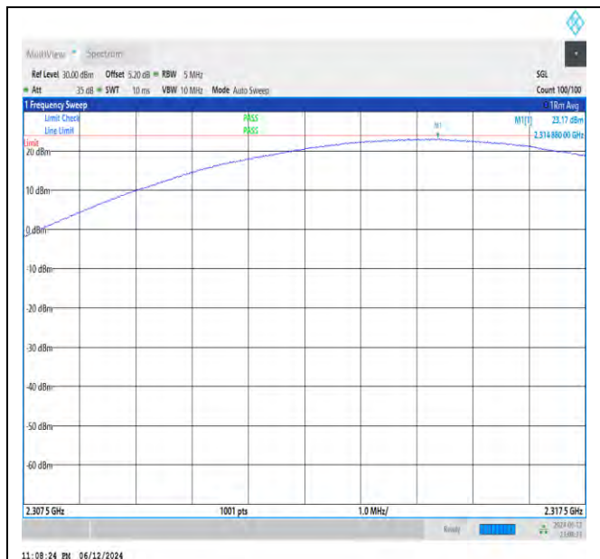
NTNV_N30_PC3_15_5_H_TID4_NS_01_2307.5_2317.5_#1
