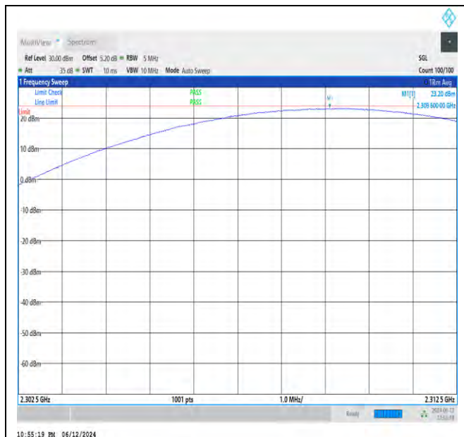
NTVN_N30_PC3_15_5_L_TID4_NS_01_2302.5_2312.5_ #1
