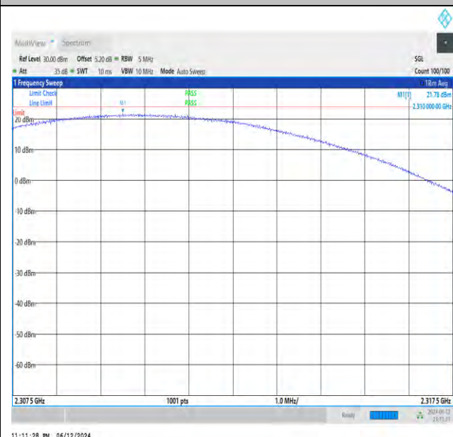
NTNV_N30_PC3_15_5_H_TID23_NS_01_2307.5_2317.5_#1
