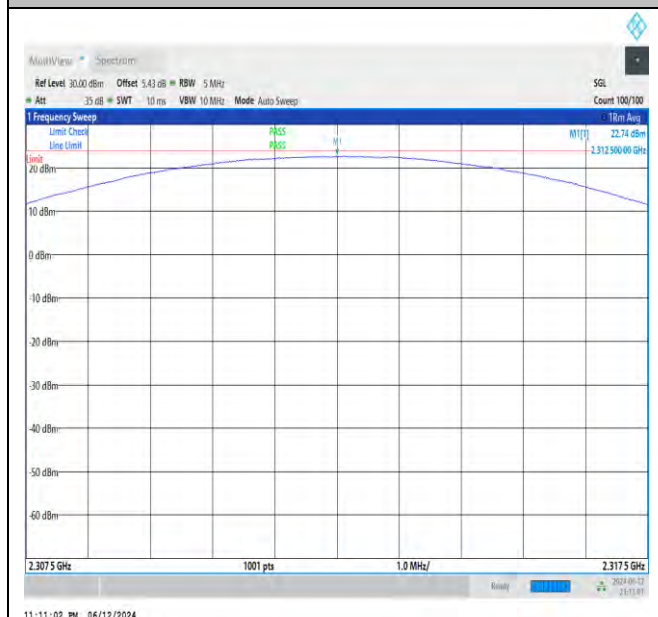
NTNV_N30_PC3_15_5_H_TID22_NS_01_2307.5_2317.5_#1
