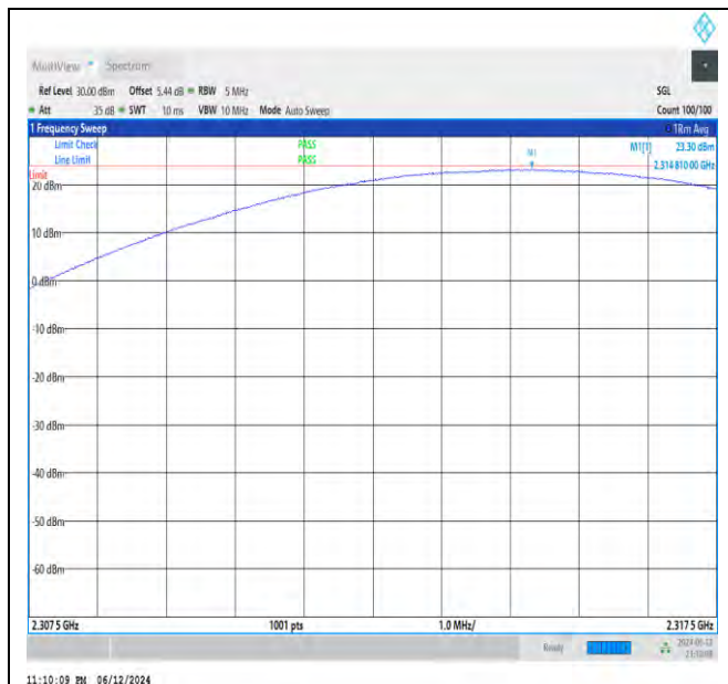
NTNV_N30_PC3_15_5_H_TID8_NS_01_2307.5_2317.5_#1
