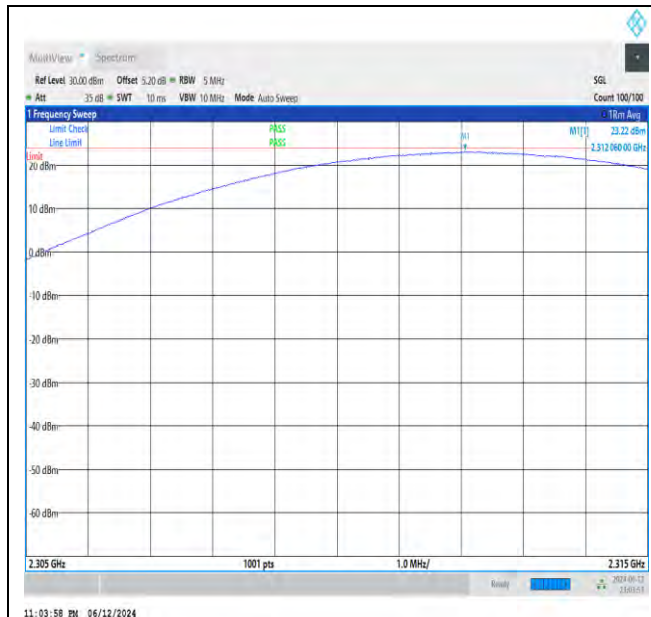
NTVN_N30_PC3_15_5_M_TID8_NS_01_2305_2315_#1
