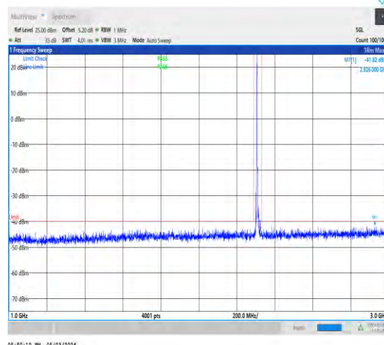
1-N30-PC3-15-10-M-1-DFT-PI2BPSK-Inner_1RB_Lef t-1@1-1000-3000-Ant0-2926.00--41.82--40-PASS
