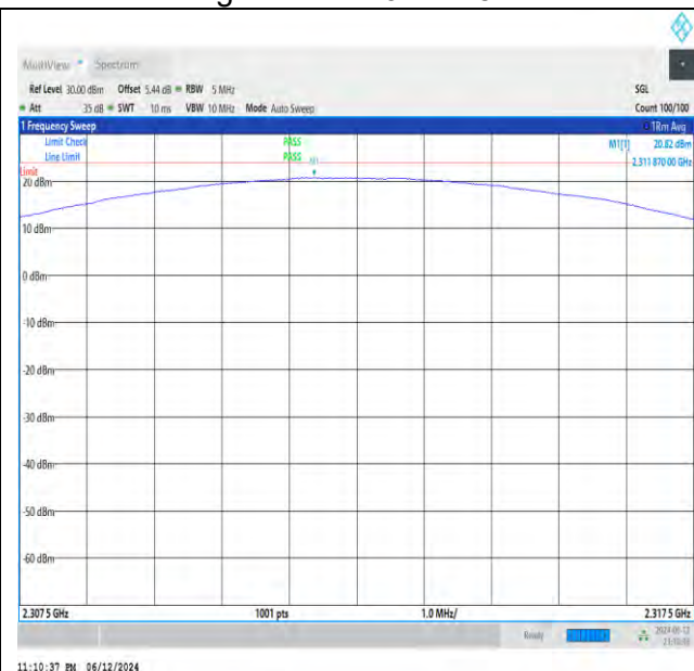
NTNV_N30_PC3_15_5_H_TID21_NS_01_2307.5_2317.5_#1
