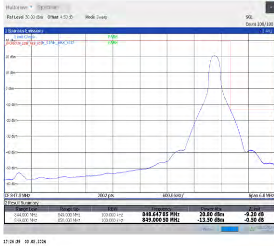
1-N26-824-849-15-5-H-2-DFT-PI2BPSK-Edge_1RB_Right-1@24-Ant0-1-seegraph-PASS-see graph
