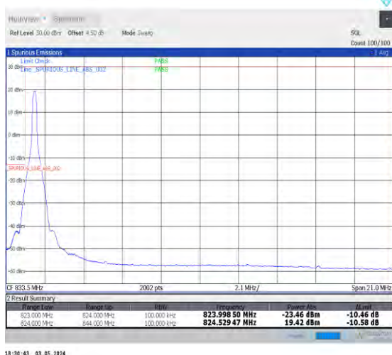
1-N26-824-849-15-20-L-4-CP-QPSK-Edge_1RB_Left- 1@0-Ant0-1-seegraph-PASS-see graph
