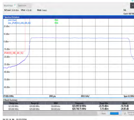
1-N26-824-849-15-5-L-6-CP-QPSK-Outer_Full-25 @0-Ant0-1-seegraph-PASS-see graph
