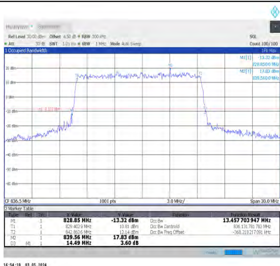
1-N26-824-849-15-15-M-1-DFT-QPSK-Outer_Full-75 @0-Ant0-13.458-14.490-≤15-PASS
