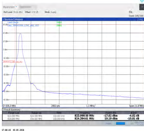
1-N26-824-849-15-10-L-4-CP-QPSK-Edge_1RB_Left- 1@0-Ant0-1-seegraph-PASS-see graph
