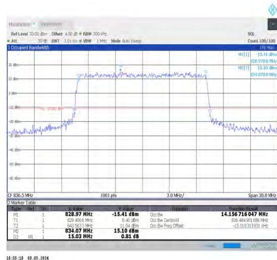
1-N26-824-849-15-15-M-6-CP-QPSK-Outer_Full-79@0-Ant0-14.157-15.030-≤15-PASS
