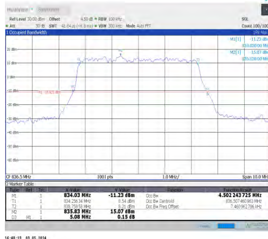
1-N26-824-849-15-5-M-4-DFT-64QAM-Outet_Full-25 @0-Ant0-4.502-5.080-≤5-PASS
