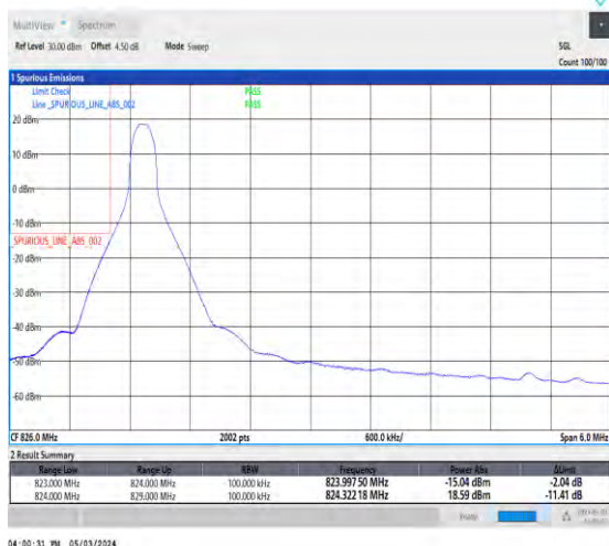
1-N26-824-849-15-5-L-4-CP-QPSK-Edge_1RB_Left-1 @0-Ant0-1-seegraph-PASS-see graph
