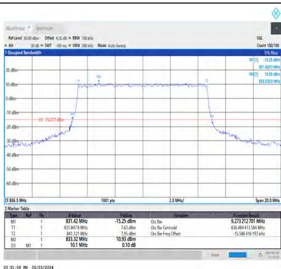
1-N26-824-849-15-10-M-8-CP-64QAM-Outer_Full-52 @0-Ant0-9.273-10.100-≤10-PASS
