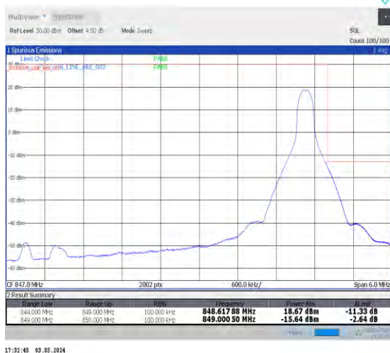
1-N26-824-849-15-5-H-5-CP-QPSK-Edge_1RB_Right-1@24-Ant0-1-seegraph-PASS-see graph
