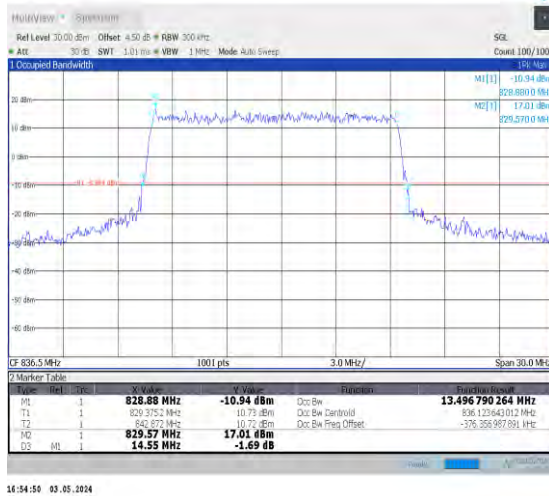
1-N26-824-849-15-15-M-3-DFT-16QAM-Outer_Full-7 5@0-Ant0-13.497-14.550-≤15-PASS
