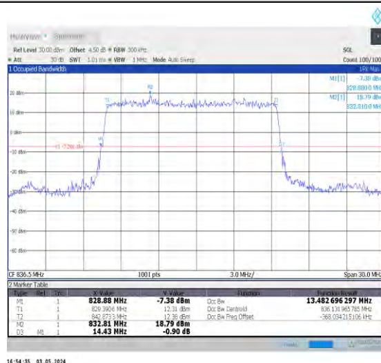
1-N26-824-849-15-15-M-2-DFT-PI2BPSK-Outer_Full-75 @0-Ant0-13.483-14.430-≤15-PASS
