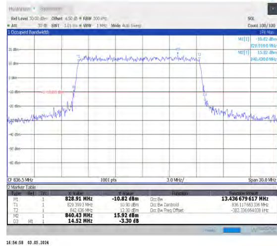
1-N26-824-849-15-15-M-4-DFT-64QAM-Outer_Full-75@0-Ant0-13.437-14.520-≤15-PASS
