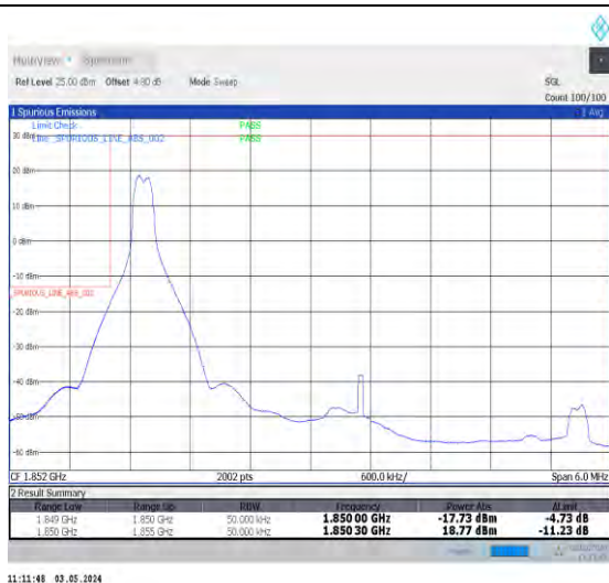
1-N25-PC3-15-5-L-1-DFT-PI2BPSK-Edge_1RB_Left-1 @0-Ant0-1-seegraph-PASS-see graph
