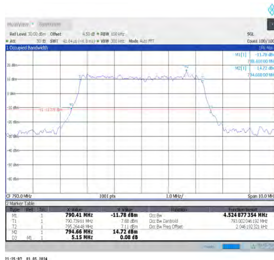
1-N14-PC3-15-5-M-8-CP-64QAM-Outer_Full-25@0-Ant0-4.525-5.150-≤5-PASS
