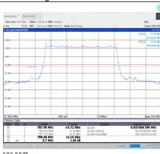
1-N14-PC3-15-10-M-1-DFT-QPSK-Outter_Full-50@0 -Ant0-8.936-9.700-≤10-PASS
