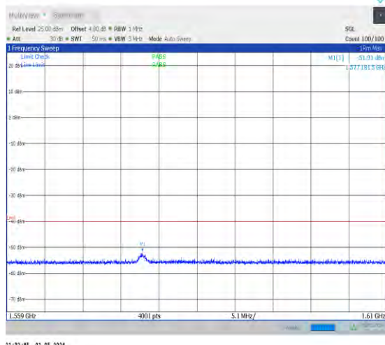
1-N14-PC3-15-10-H-1-DFT-PI2BPSK-Inner_1RB_L eft-1@1-1559-1610-Ant0-1577.18--51.91--40-PASS
