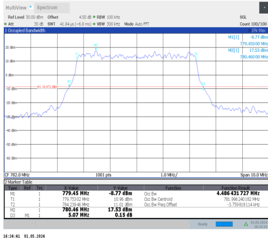
1-N13-PC3-15-5-M-1-DFT-QPSK-Outter_Full-25@0- Ant0-4.486-5.070-≤5-PASS
