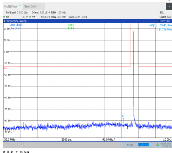
1-N13-PC3-15-10-L-1-DFT-PI2BPSK-Inner_1RB_Le ft-1@1-30-1000-Ant0-717.73--59.40--13-PASS
