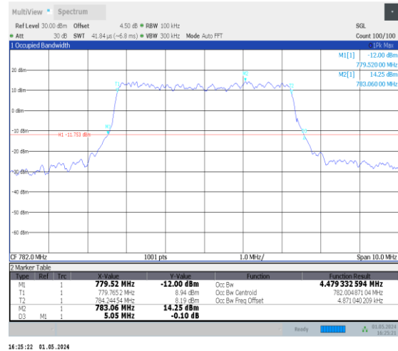
1-N13-PC3-15-5-M-4-DFT-64QAM-Outter_Full-25@0- -Ant0-4.479-5.050-≤5-PASS
