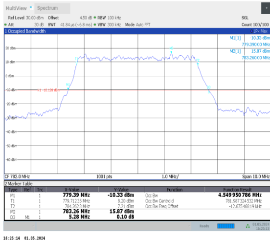
1-N13-PC3-15-5-M-3-DFT-16QAM-Outter_Full-25@0- -Ant0-4.55-5.280-≤5-PASS
