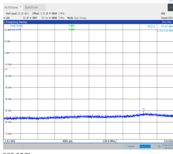
1-N13-PC3-15-10-M-1-DFT-PI2BPSK-Inner_1RB_L ef t-1@1-1610-3000-Ant0-2752.23--51.87--13-PASS
