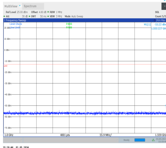
1-N13-PC3-15-10-L-1-DFT-PI2BPSK-Inner_1RB_Left -1@1-1000-1559-Ant0-1555.23--53.22--13-PASS
