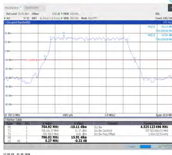
1-N12-PC3-15-5-M-2-DFT-P12BPSK-Outer_Full-25@0-Ant0-4.525-5.270-≤5-PASS
