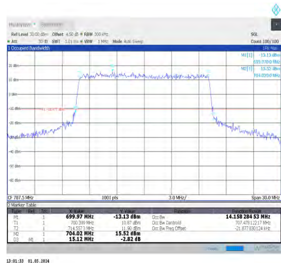
1-N12-PC3-15-15-M-6-CP-QPSK-Outer_Full-79@0- Ant0-14.158-15.120-≤15-PASS
