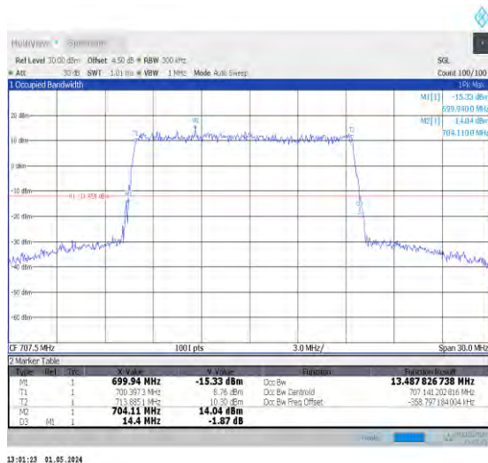
1-N12-PC3-15-15-M-5-DFT-256QAM-Outer_Full-75 @0-Ant0-13.488-14.400-≤15-PASS
