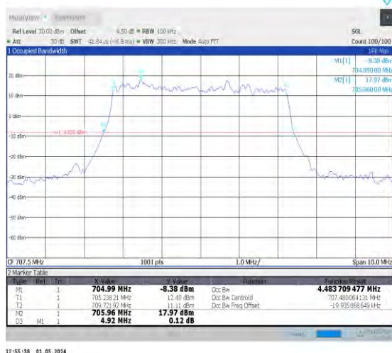
1-N12-PC3-15-5-M-1-DFT-QPSK-Outer_Full-25@0-Ant0-4.484-4.920-≤5-PASS
