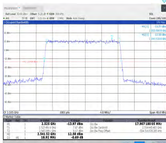
1-N7-PC3-15-20-M-5-DFT-256QAM-Outer_Full-100@0-Ant0-17.907-18.920-≤20-PASS
