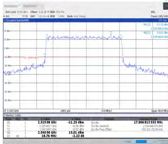
1-N7-PC3-15-20-M-3-DFT-16QAM-Outer_Full-100@0-Ant0-17.907-18.760-≤20-PASS
