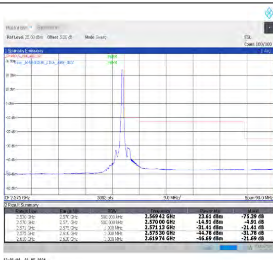
1-N7-PC3-15-40-H-2-DFT-PI2BPSK-Edge_1RB_Right-1@215-Ant0-1--PASS-see graph
