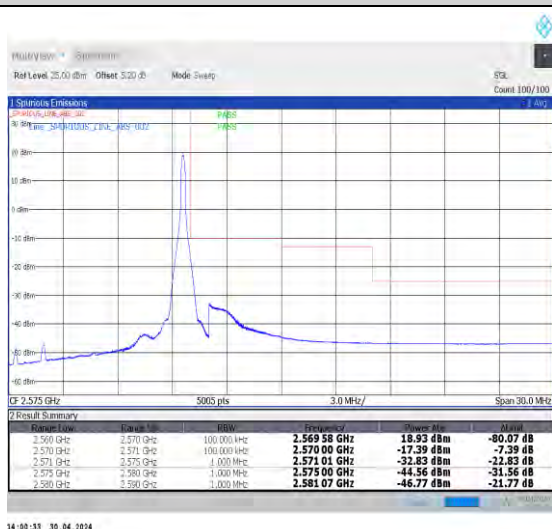
1-N7-PC3-15-10-H-5-CP-QPSK-Edge_1RB_Right-1@51-Ant0-1--PASS-see graph
