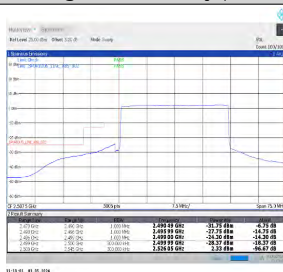
1-N7-PC3-15-30-L-6-CP-QPSK-Outer_Full-160@ 0-Ant0-1--PASS-see graph
