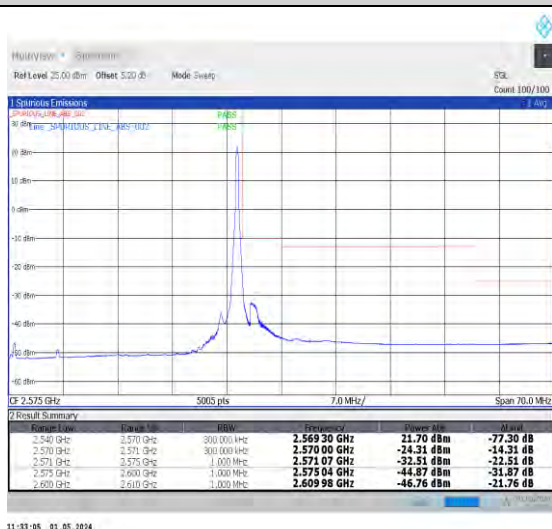
1-N7-PC3-15-30-H-5-CP-QPSK-Edge_1RB_Right-1@159-Ant0-1--PASS-see graph
