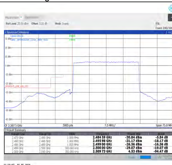
1-N7-PC3-15-30-L-3-DFT-PI2BPSK-Outer_Full-16 0@0-Ant0-1--PASS-see graph
