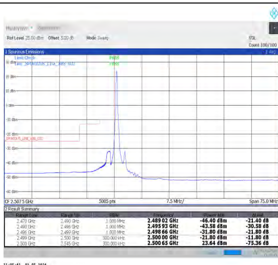
1-N7-PC3-15-30-L-1-DFT-PI2BPSK-Edge_1RB_Left-1 @0-Ant0-1--PASS-see graph
