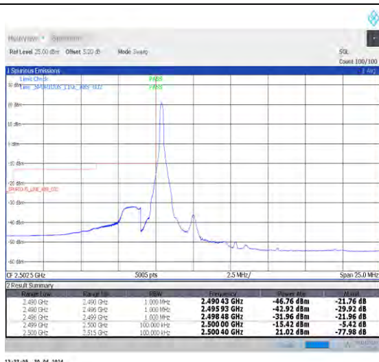
1-N7-PC3-15-10-L-1-DFT-PI2BPSK-Edge_1RB_Left-1 @0-Ant0-1--PASS-see graph
