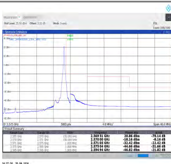
1-N7-PC3-15-15-H-5-CP-QPSK-Edge_1RB_Right-1@78-Ant0-1--PASS-see graph
