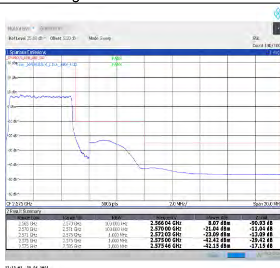
1-N7-PC3-15-5-H-3-DFT-PI2BPSK-Outer_Full-25 @0-Ant0-1--PASS-see graph
