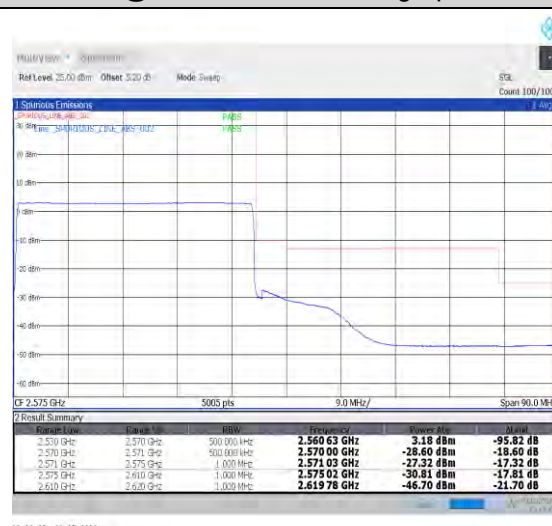
1-N7-PC3-15-40-H-6-CP-QPSK-Outer_Full-216@0-Ant0-1--PASS-see graph
