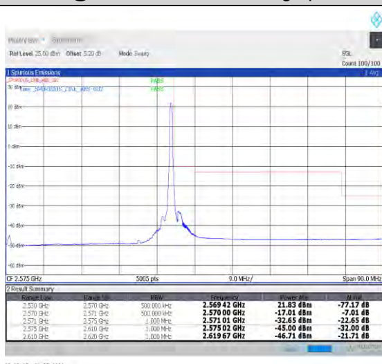
1-N7-PC3-15-40-H-5-CP-QPSK-Edge_1RB_Right-1@215-Ant0-1--PASS-see graph
