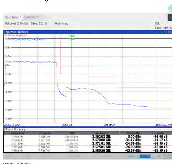
1-N7-PC3-15-10-H-3-DFT-PI2BPSK-Outer_Full-50@0-Ant0-1--PASS-see graph
