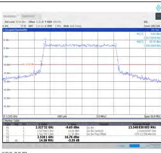
1-N7-PC3-15-15-M-3-DFT-16QAM-Outer_Full-75@0 -Ant0-13.549-14.580-≤15-PASS
