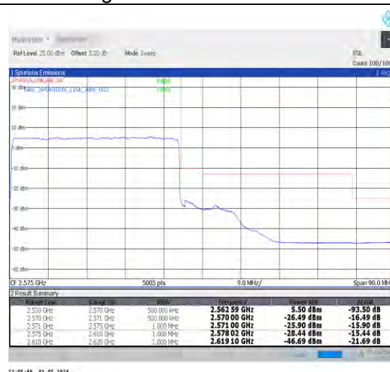
1-N7-PC3-15-40-H-3-DFT-PI2BPSK-Outer_Full-216@0-Ant0-1--PASS-see graph
