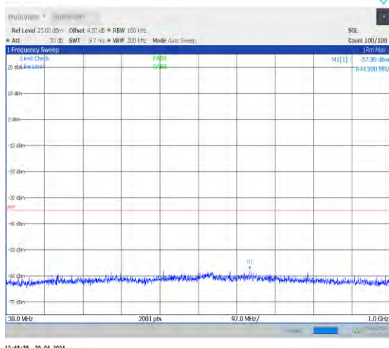
1-N7-PC3-15-40-M-1-DFT-PI2BPSK-Inner_1RB_Lef t-1@1-30-1000-Ant0-548.47--57.90--35-PASS
