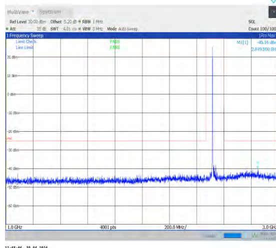
1-N7-PC3-15-40-M-1-DFT-PI2BPSK-Inner_1RB_Left -1@1-1000-3000-Ant0-2737.50--40.16--25-PASS
