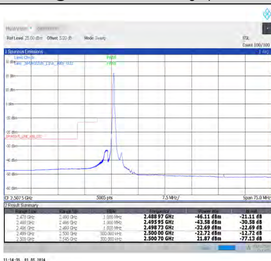
1-N7-PC3-15-30-L-4-CP-QPSK-Edge_1RB_Left-1@0- Ant0-1--PASS-see graph
