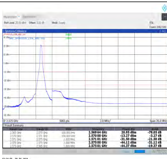
1-N7-PC3-15-5-H-2-DFT-PI2BPSK-Edge_1RB_Right-1 @24-Ant0-1--PASS-see graph
