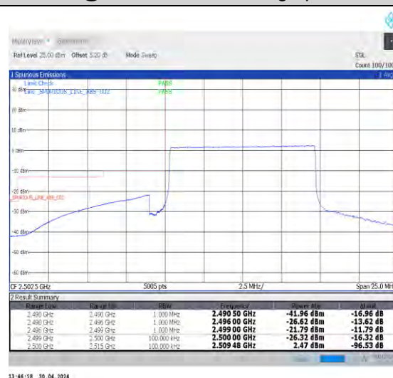
1-N7-PC3-15-10-L-6-CP-QPSK-Outer_Full-52@0-Ant0-1--PASS-see graph
