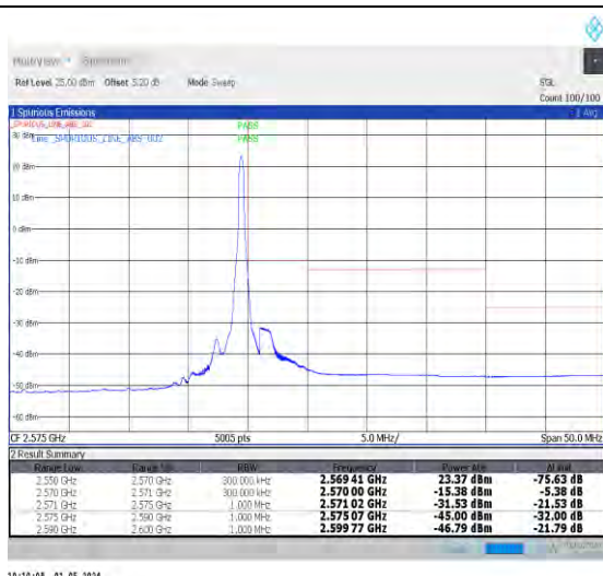
1-N7-PC3-15-20-H-2-DFT-PI2BPSK-Edge_1RB_Right-1@105-Ant0-1--PASS-see graph
