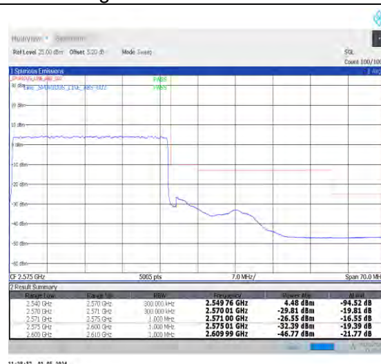
1-N7-PC3-15-30-H-3-DFT-PI2BPSK-Outer_Full-160@0-Ant0-1--PASS-see graph
