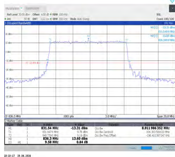
1-N5-15-10-M-3-DFT-16QAM-Outer_Full-50@0-Ant0- -8.912-9.580-≤10-PASS
