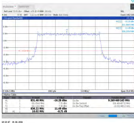
1-N5-15-10-M-6-CP-QPSK-Outer_Full-52@0-Ant0-9. 269-10.020≤10-PASS
