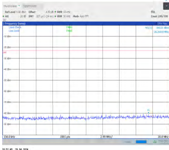
1-N5-15-20-M-1-DFT-PI2BPSK-Inner_1RB_Left-1@ 1-0.15-30-Ant0-26.27--80.51--23-PASS
