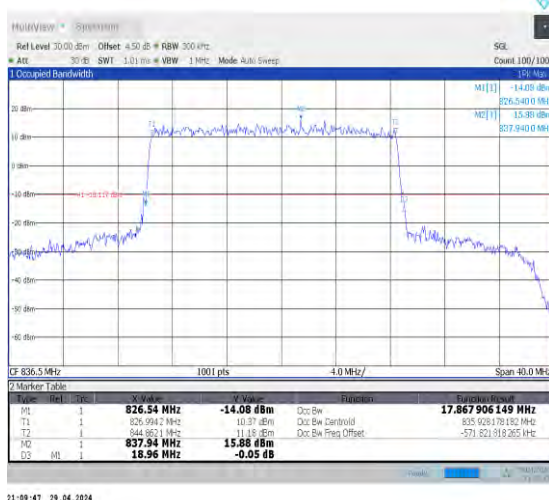
1-N5-15-20-M-4-DFT-64QAM-Outet_Full-100@0-Ant 0-17.868-18.960-≤20-PASS
