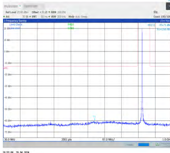
1-N5-15-20-M-1-DFT-PI2BPSK-Inner_1RB_Left-1@ 1-30-1000-Ant0-554.29--59.71--13-PASS
