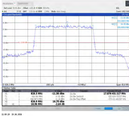
1-N5-15-20-M-2-DFT-PI2BPSK-Outet_Full-100@0-A nt0-17.876-18.960-≤20-PASS
