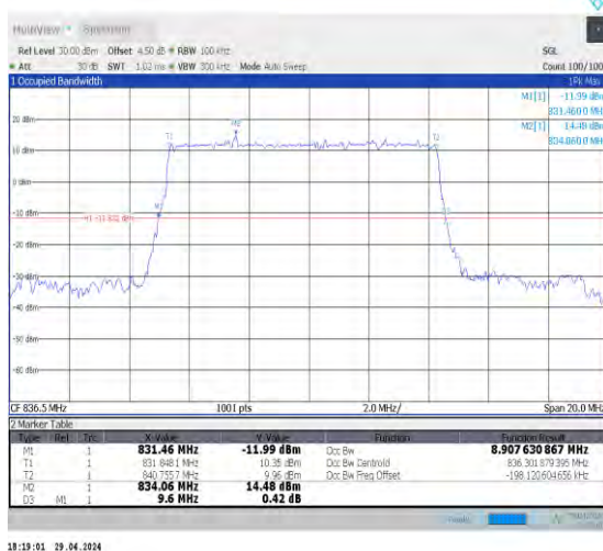
1-N5-15-10-M-2-DFT-PI2BPSK-Outer_Full-50@0-Ant0- 8.908-9.600-≤10-PASS
