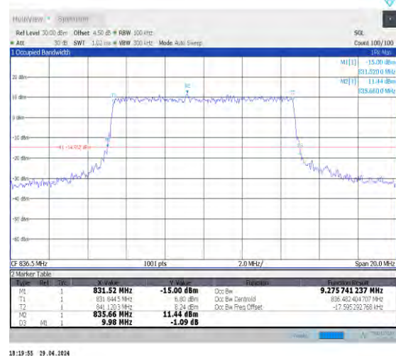
1-N5-15-10-M-7-CP-16QAM-Outer_Full-52@0-Ant0- 9.276-9.980≤10-PASS
