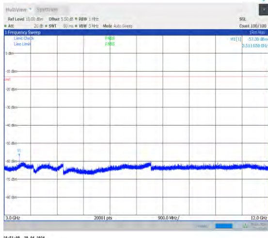
1-N5-15-20-L-1-DFT-PI2BPSK-Inner_1RB_Left-1@ -3000-12000-Ant0-3511.65--57.30--13-PASS
