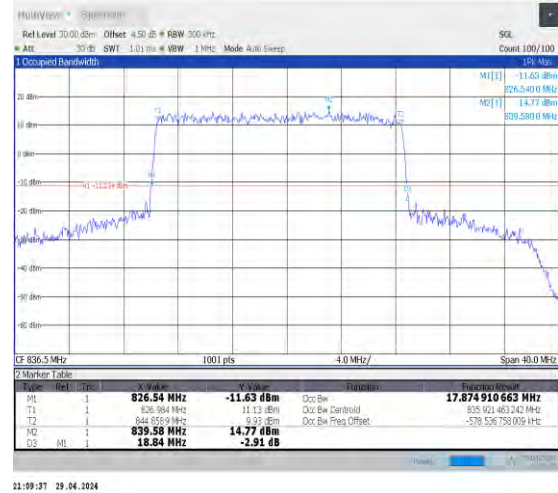
1-N5-15-20-M-3-DFT-16QAM-Outet_Full-100@0-Ant 0-17.875-18.840-≤20-PASS
