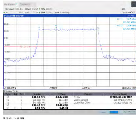
1-N5-15-10-M-1-DFT-QPSK-Outer_Full-50@0-Ant0- 8.918-9.680-≤10-PASS
