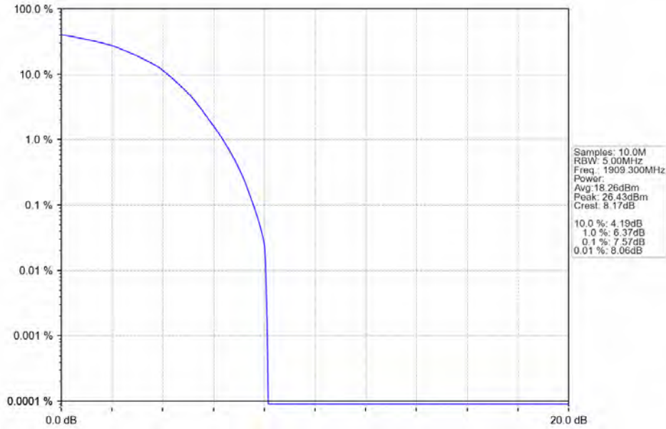
Band2_1.4MHz_64QAM_HCH_1909.3MHz_RB_6_0_NTNV
