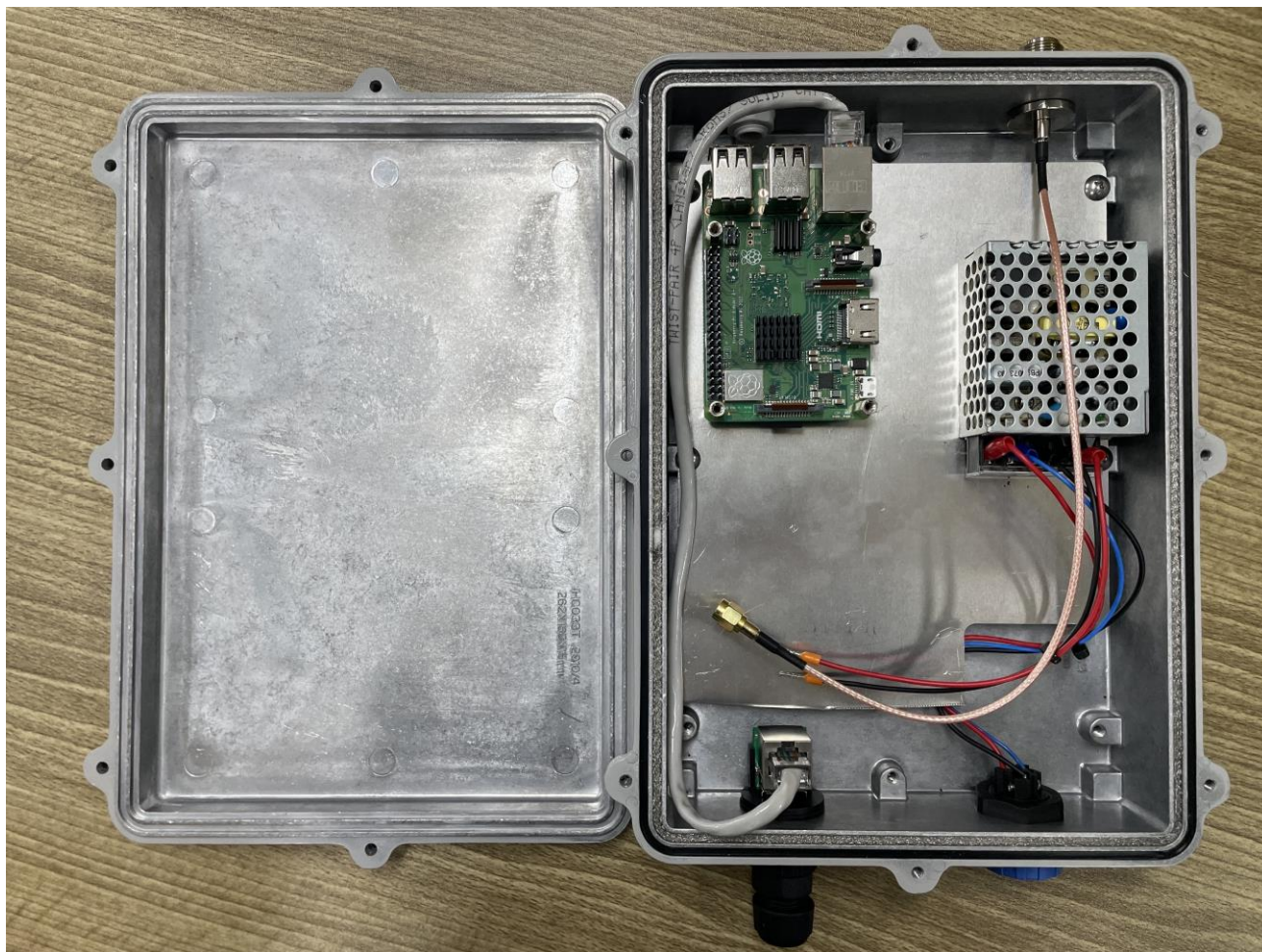
[Raspberry Pi PCB Board (Full photo)]
