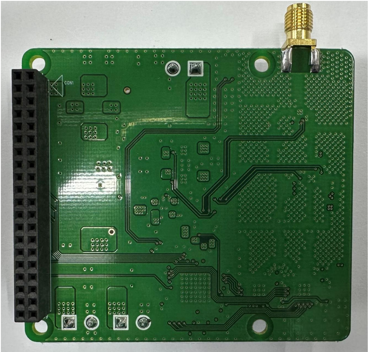
[PCB Board(Rear)]
