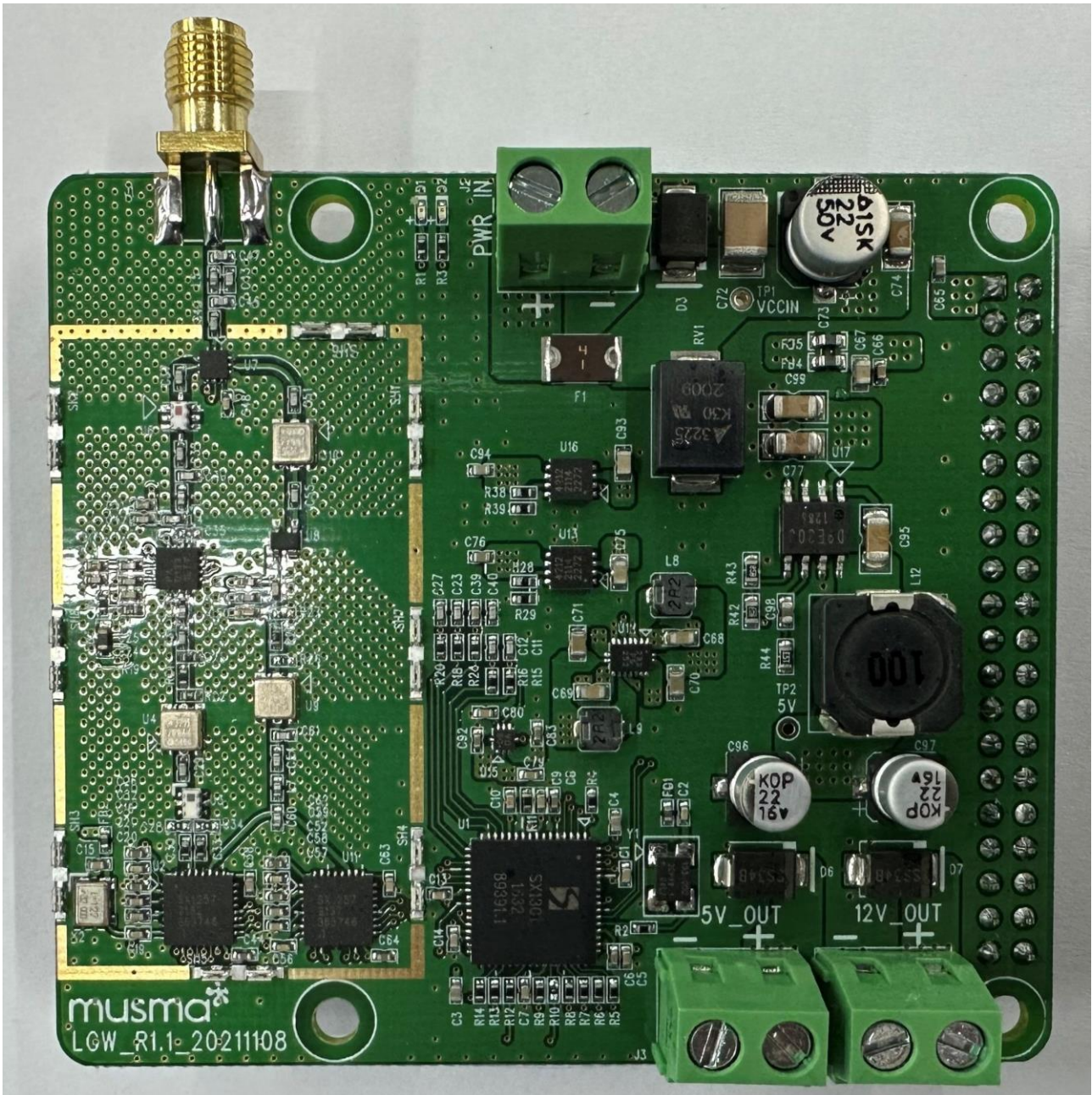
[PCB Board (Shield can removal)]
