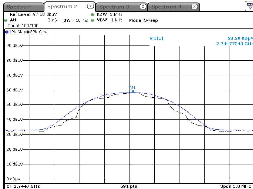
Radiated Spurious Emissions plot – Average Result (SF7_High 3rd Harmonic, Z-H)
