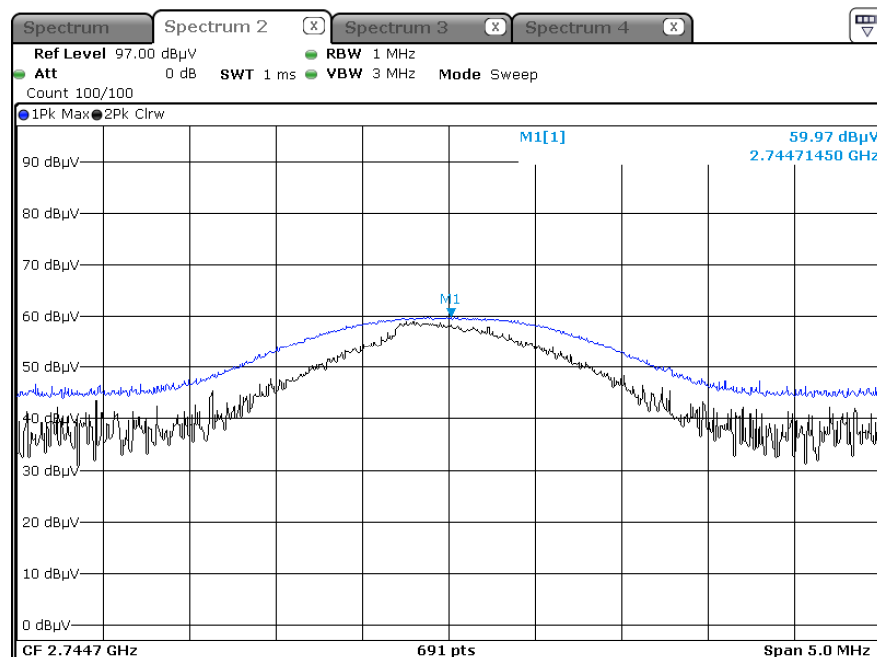
Radiated Spurious Emissions plot – Peak Result (SF7_High 3rd Harmonic, Z-H)
