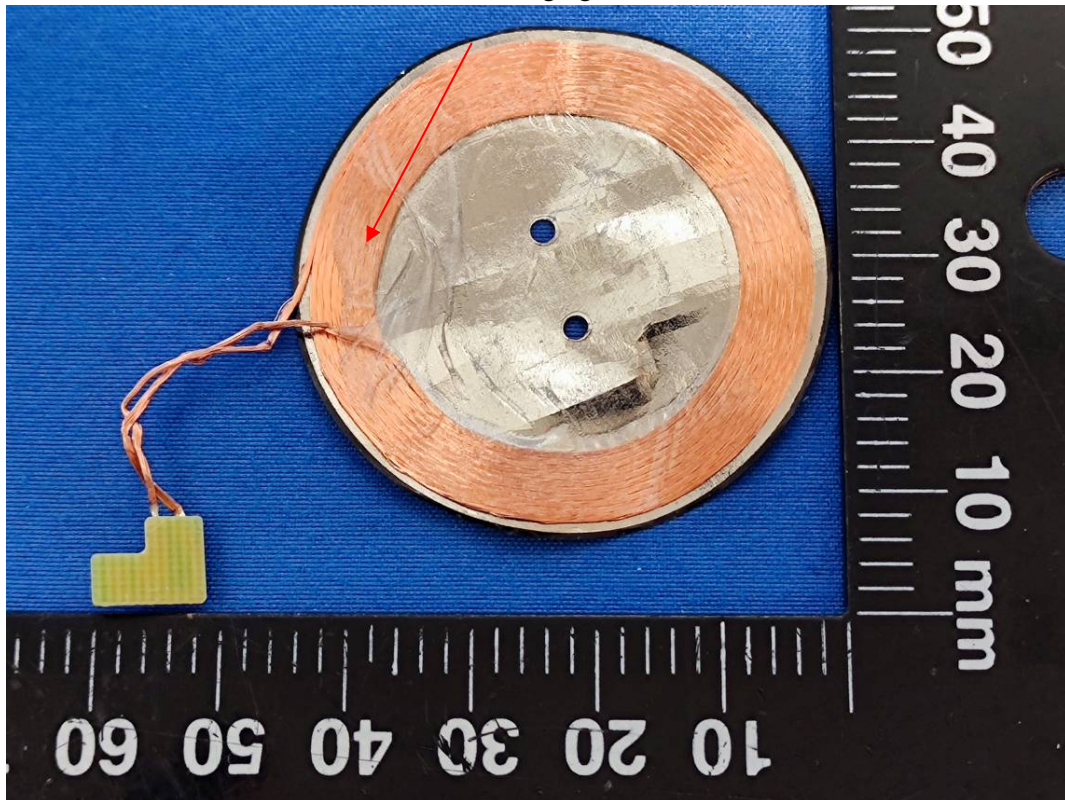
Wireless Charging Antenna
