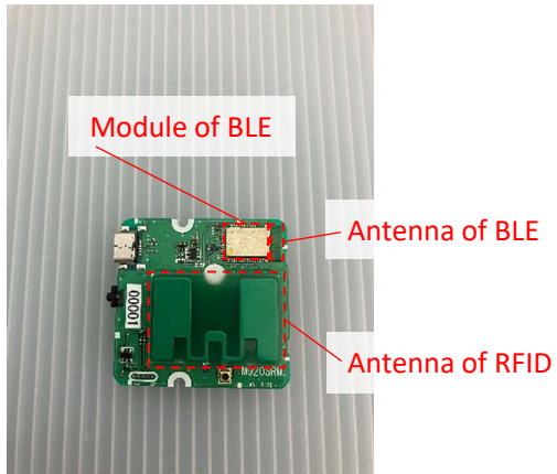
Antenna side
