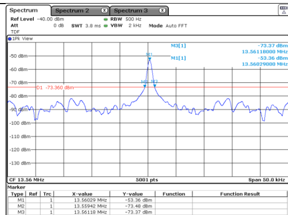
20 dB Bandwidth
