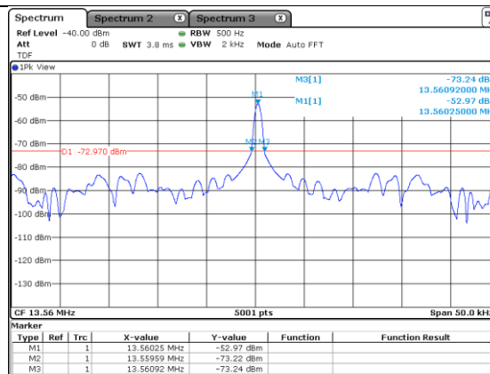
20 dB Bandwidth
