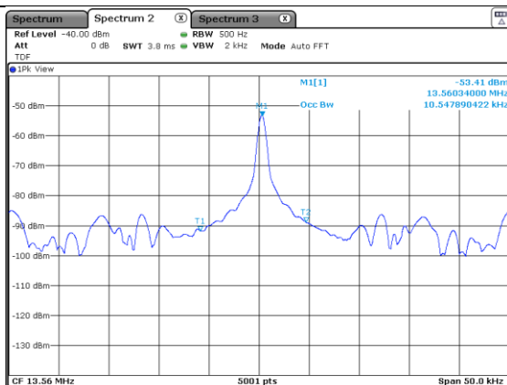
99% Occupied Bandwidth
