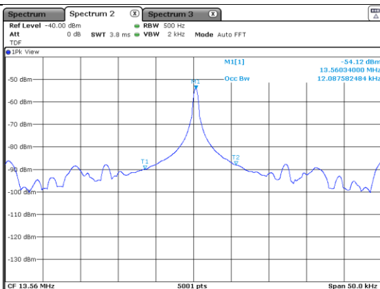
99% Occupied Bandwidth
