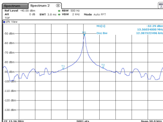
99% Occupied Bandwidth
