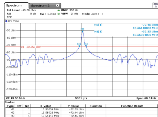
20 dB Bandwidth
