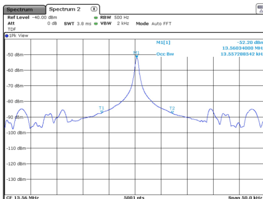
99% Occupied Bandwidth
