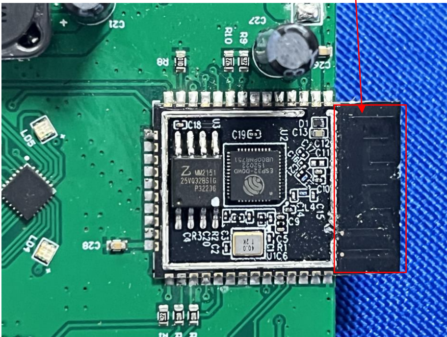
WIFI2.4G Antenna
