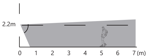
Overhead View
