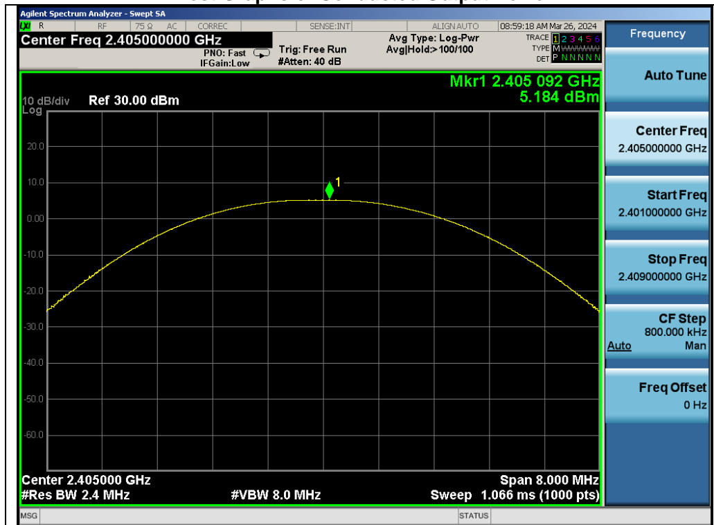
Test_Graph_GFSK_ANT1_2405_Peak Power
