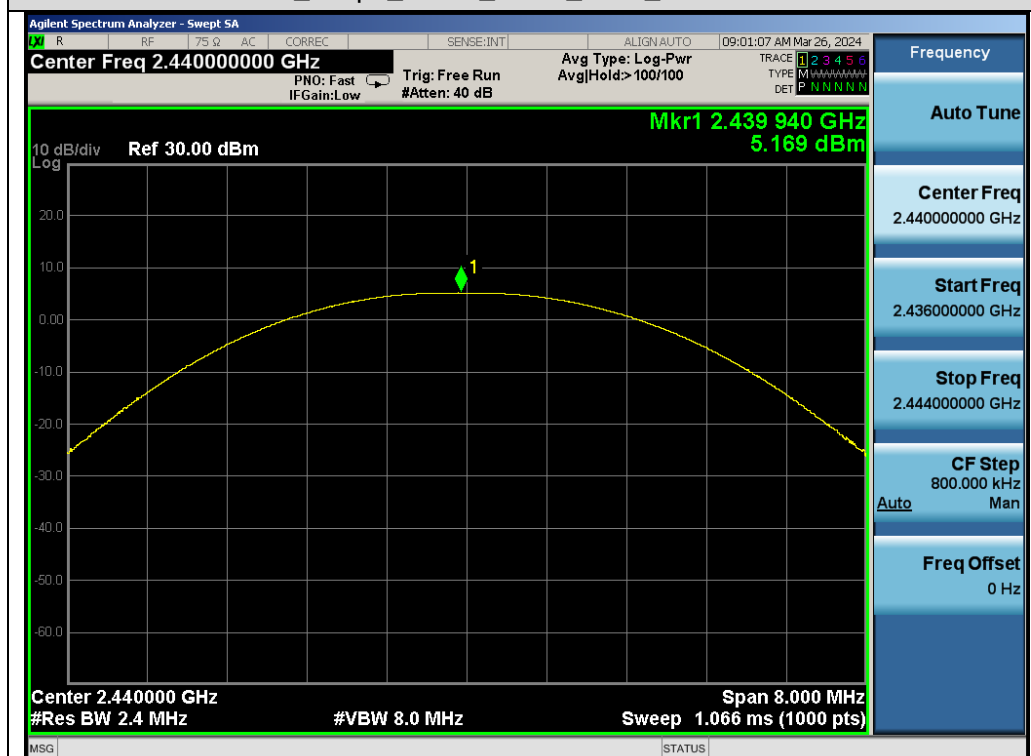
Test_Graph_GFSK_ANT1_2440_Peak Power
